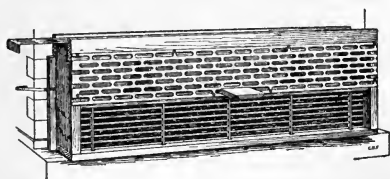
FIG. 30. — Alley queen and drone trap.
