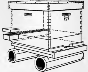
FIG. 106. — Alexander feeder in collar under hive-body.
