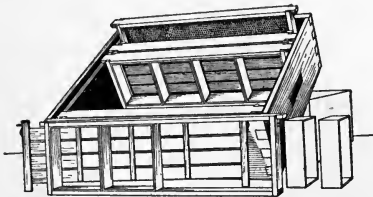
FIG. 133. — Super for tall ( 4\frac{1}{2} by 4\frac{1}{2} ) sections in wide frames. Shallow extracting frames are shown at the sides.
