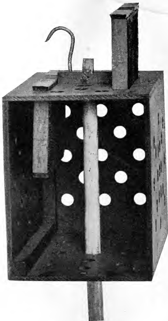
FIG. 47. — Swarm catcher.
