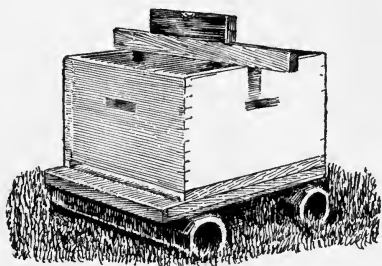
FIG. 104. — Hive leveling device. In the upper figure the wedge-shaped piece is on edge so that when the top is level the hive entrance is one inch lower than the back. In the lower figure the wedge is on its side.
