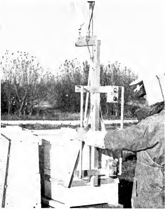
Cradle of hive loader with control buttons. Spring-loaded clamps fit into the hive handholds to support the hive. (Fig. 67)
