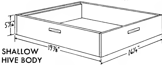
SHALLOW FRAME
