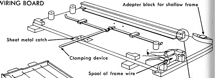
WIRING BOARD
