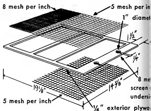
(A) DETAILS OF POLLEN-REMOVING SCREENS
