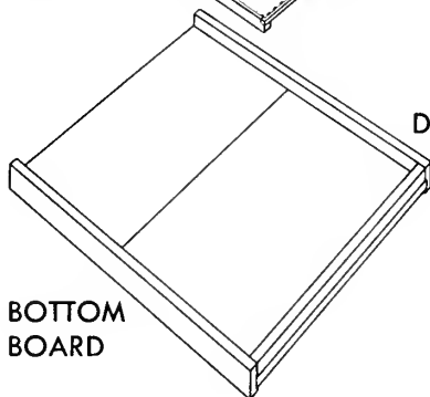
POLLEN TRAY
