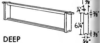
DEEP FRAME
