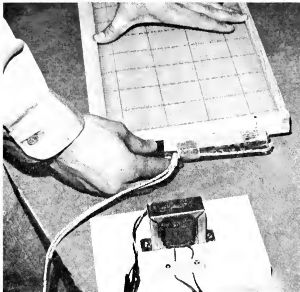
A simple device for embedding wires into comb foundation. When the copper contacts at each end of the wooden piece touch the wires on the frame end bar, the heated wires sink into the wax. (Fig. 20)
