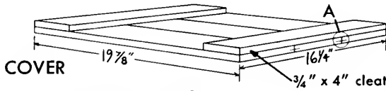
(A) DETAIL OF COVER AND BOTTOM
