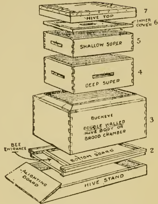
Fig. 53.—A Canadian Hive, known as the "Buckeye."
