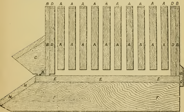
Fig. 6.—(b) Section of Frame Hive, seen from side (frames running parallel to entrance). A, Bars of frame; B, Front and back walls of hive; c, Porch; D, Dummy-board; E, Floor-board; F, Stand; G, Plinth; H, Alighting-board; K, Entrance contractor.
