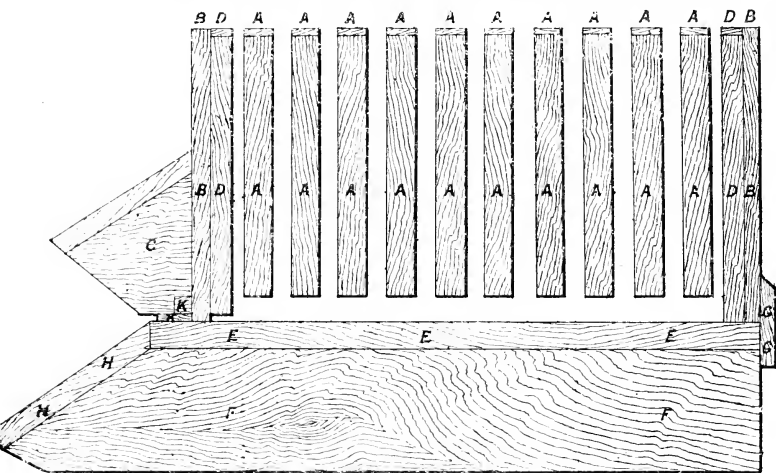
Fig. 6.—(b) Section of Frame Hive, seen from side (frames running parallel to entrance). A, Bars of frame; B, Front and back walls of hive; C, Porch; D, Dummy-beards; E, Floor-board; F, Stand; G, Plinth; H, Alighting-board; K, Entrance-contractor.
