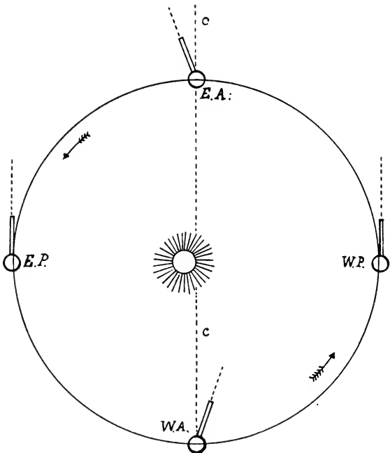
Fig. 10. —ABERRATION & PARALLAX.
