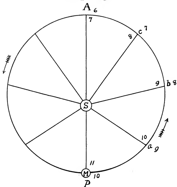
Fig. 13. —KEPLER'S LAW.
