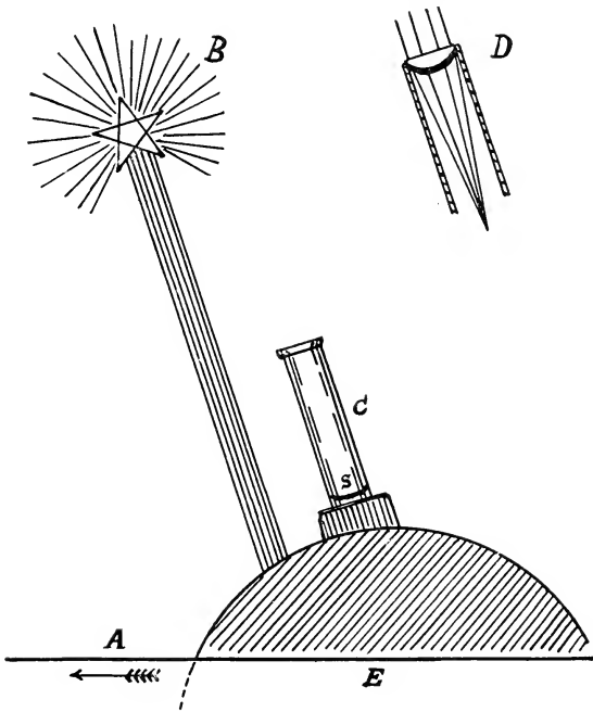
Fig. 9. — ABERRATION.
