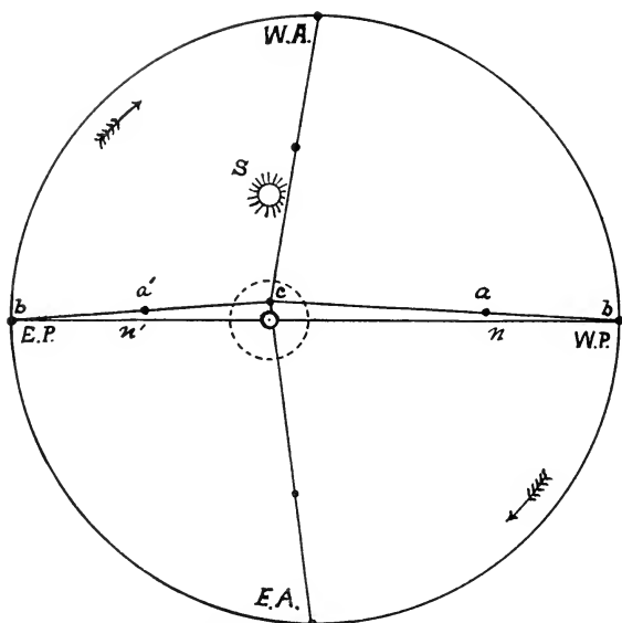
Fig. 11. —ABERRATION & PARALLAX.
