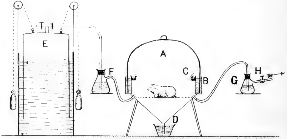
A Respiration Chamber. B Water Seal. C Soda Lime Tray. D Excreta Outlet. E Gasometer. F Wash Bottle. G Indicator Wash Bottle. H Outlet to Vacuum Pump.
