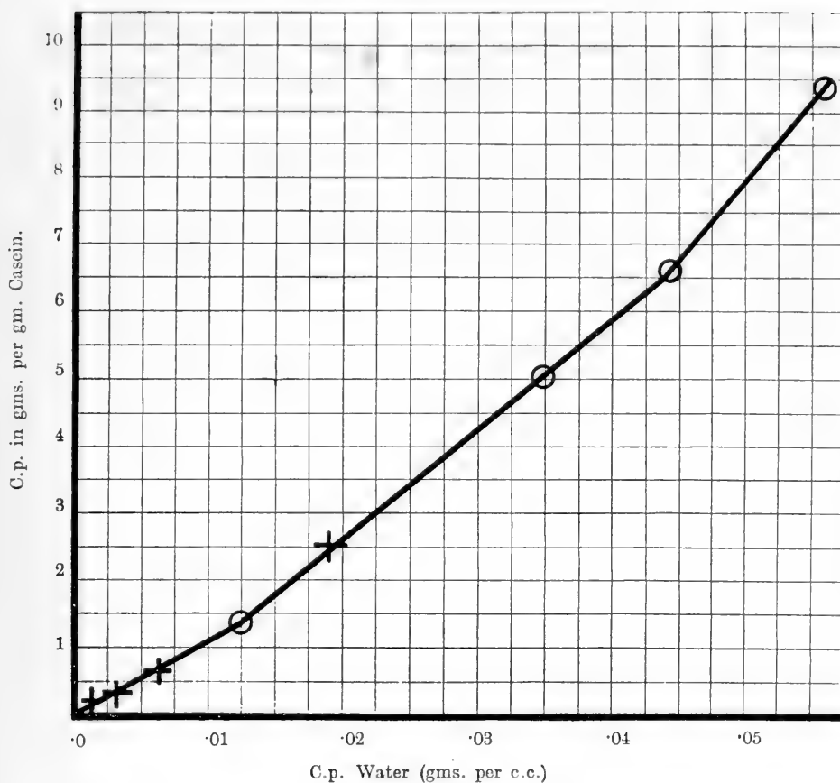
DIAGRAM IV.—Equilibria with phenol between water and casein. ( Experiment I , Table V.)
