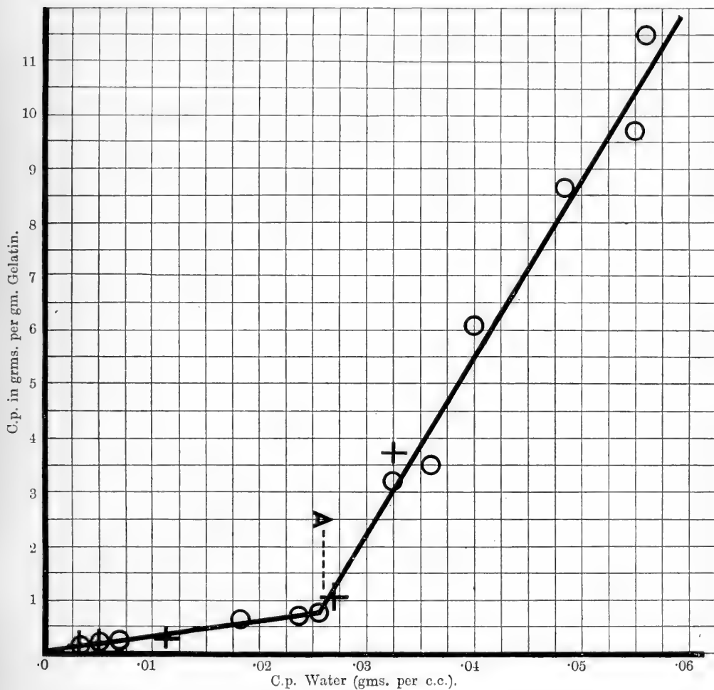
DIAGRAM I.—Equilibria with phenol between water and gelatin showing influence of phenol-coagulation upon the distribution of phenol between water and protein. ( Experiment II , Table I).
