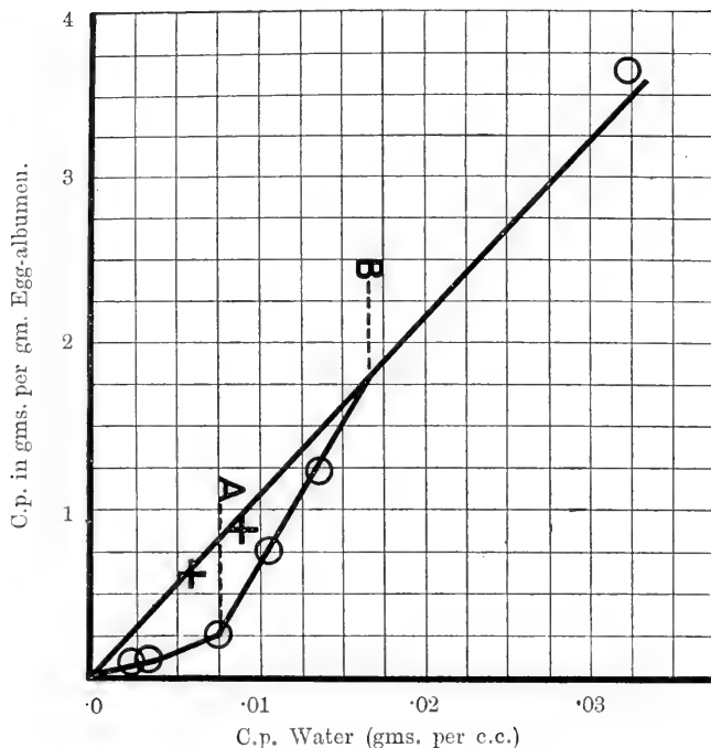
DIAGRAM II.—Equilibria with phenol between water and egg-albumen showing the influence of phenol-coagulation on the distribution of phenol between water and protein. ( Experiment I , Table II).
