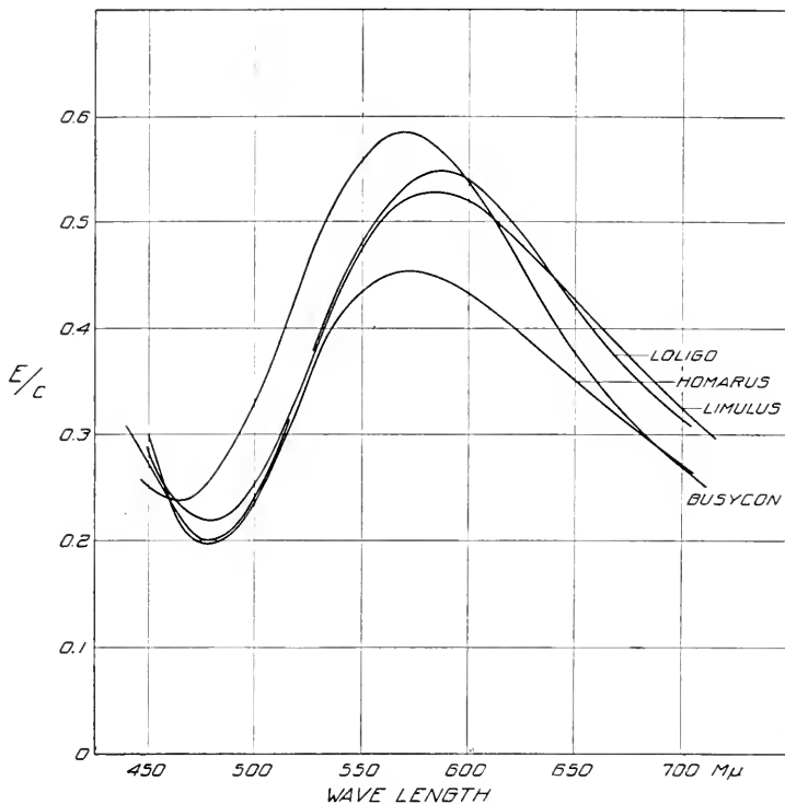
FIG. 10. Absorption spectra of chromatic groups of blood of Busycon , Limulus , Loligo and Homarus . For data see Figs. 3, 4, 5 and 6.
