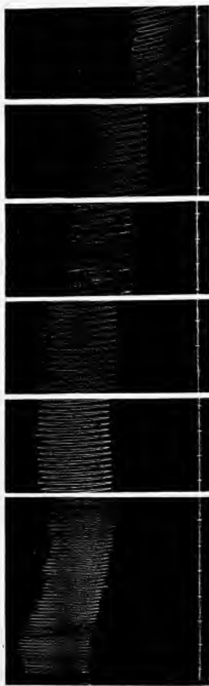
FIG. 4. Experiment 75. Cloacal strip in 125 cc. of sea water treated with carbon dioxide, pH 7.0. A , beginning at 10:00; B , 10:30; C , 11:00; D , 11:30; E , 12:00; F , 12:52. At the end, 12:56, pH 7.0.
