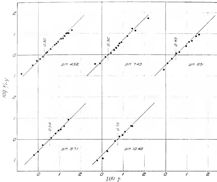
FIG. 2. Logarithmic plot of data of oxygen dissociation curve of hemocyanin of Limulus polyphemus at various pH values. Temperature, 25° C.; y , fraction of hemocyanin in oxygenated condition; p , oxygen pressure in mm. Hg.
