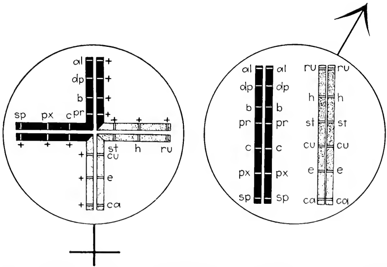
FIG. 2.—Determination of the points at which chromosomes are broken in translocations. A translocation carrying female heterozygous for a series of genes (left) is crossed to a male free from the translocation and homozygous for the respective genes (right).
