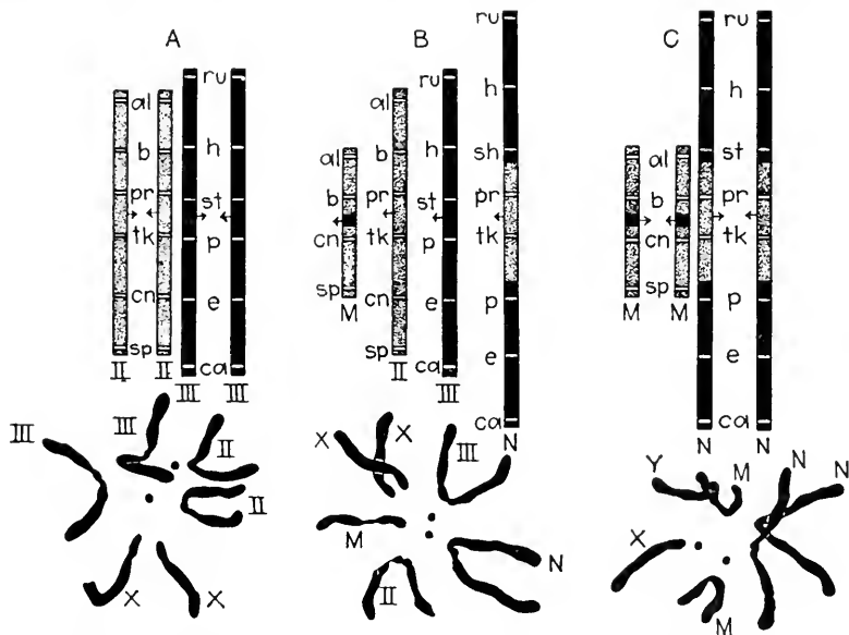
FIG. 3.—A, the second chromosome (stippled) and the third chromosome (black) of a normal Drosophila melanogaster ; B, the second and third chromosomes of an individual carrying a translocation in heterozygous condition; C, same of an individual homozygous for the same translocation. Below—chromosome plates of each of these three kinds of individuals.
