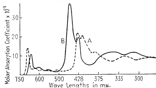
FIG. 3.—Absorption curves in benzene of A, chlorophyll a ; B, chlorophyll b . (Winterstein and Stein, 145.)
