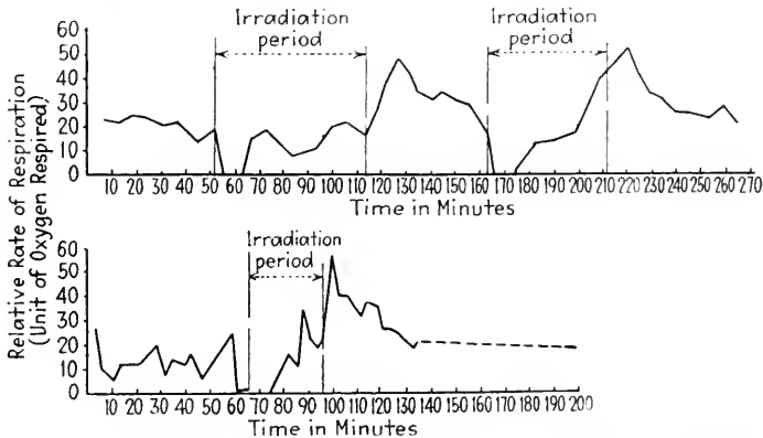
FIG. 1.—Effect of raying on the rate of respiration of etiolated pea seedlings. (After Masure, 11.)
