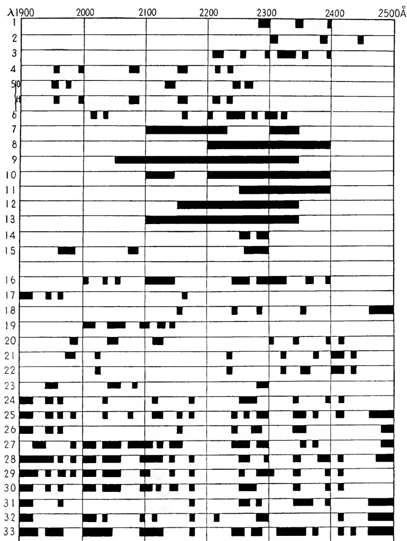
FIG. 6.—Mitogenetic spectra. 1. Reduction of \text{Cu}^{++} to \text{Cu} (electrochem.) (33). 2. Reduction of \text{Zn}^{++} to \text{Zn} (electrochem.) (33). 3. Reduction of \text{Hg}^{++} to \text{Hg} (electrochem.) (33). 4. Reaction, \text{HCl} + \text{Zn} , \text{HCl} + \text{Cu} , \text{HCl} + \text{Mg} , \text{HCl} + \text{Al} (33). 5a. Reduction of \text{O}_2 \rightarrow \text{O}^{\cdot-} ( \text{OH}^{\cdot} ) (electrochem.) (33). 5b. \text{H} \rightarrow \text{H}_2 (electrochem.) (33). 6. Redox reaction, \text{Fe}_2(\text{SO}_4)_3 + \text{FeSO}_4 (electrochem.) (33). 7. Reaction, \text{K}_2\text{Cr}_2\text{O}_7 + \text{FeSO}_4 (212). 8. Reaction, \text{FeCl}_3 + \text{NH}_2\text{OH} \cdot \text{HCl} (212). 9. Reaction, \text{KMnO}_4 + \text{H}_2\text{O}_2 (212). 10. Reaction, \text{HgCl}_2 + \text{SnCl}_2 (212). 11. Reaction, \text{HNO}_3 + \text{FeSO}_4 (+\text{H}_2\text{SO}_4) (212). 12. Reaction, \text{KClO}_3 + \text{Zn} + \text{NaOH} (212). 13. Reaction, \text{Pt} + \text{H}_2\text{O}_2 (212). 14. Reaction, \text{KOH} + \text{pyrogallol} (120). 15. Reaction, \text{NaOH} + \text{HCl} (212). 16. Photosynthesis (212). 17. Glycolysis, spectrum from blood radiation (also obtained from corneal epithelium) (152). 18. Phosphatase (action on phosphates) (126). 19. Breaking down of creatin phosphatase (34). 20. Protein digestion (18). 21. Reaction, amylase with maltose (160). 22. Reaction, cane sugar with yeast saccharase (160). 23. Reaction, urea with urease (160). 24. From resting nerve (151). 25. From nerve pulp (151). 26. Nerve mechanically stimulated (at point of stimulation) (151). 27. Nerve electrically stimulated between electrodes (151). 28. Nerve, traumatic stimulus about 20 mm. from the trauma (151). 29. Nerve, electric stimulus 20 mm. from electrodes (151). 30. Nerve, conduction of stimulus (20 min.) (111). 31. Small brain (111). 32. Large brain (111). 33. Optic nerve (111). (Collected and supplied by Gurwitsch.)
