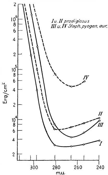
FIG. 3.—Sensitivity curve of B. prodigiosus and Staph. aureus : continuous lines represent 1 to 10 per cent killing, and broken lines 90 to 100 per cent killing. (From Ehrismann and Noethling, 45.)
