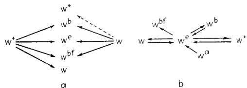
FIG. 3.—(a) Mutations from the wild type, and from white, to different intermediate allelomorphs; (b) mutations at the white locus to and from the intermediate allelomorph eosin ( w e ). [After Timoféeff-Ressovsky (183).]
