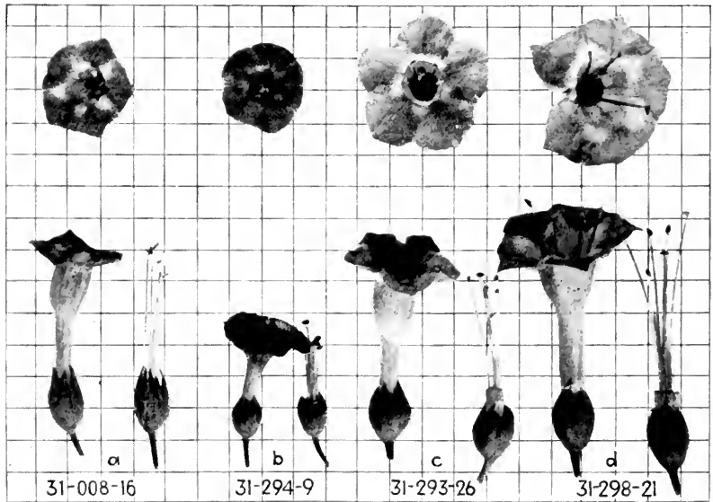
FIG. 4.—Flowers of N. Tabacum var. purpurea . (a) Control, (b), (c), and (d), types obtained in third generation after X-radiation from a "normal" in the first generation progeny, the extent of variation in which is shown in Fig. 3.
