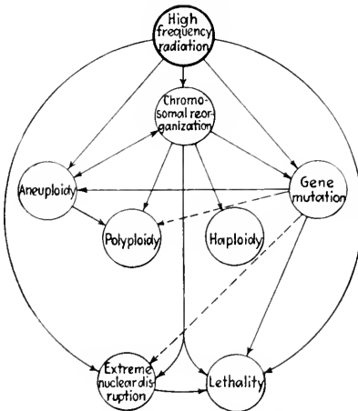
FIG. 1.—Chart illustrating primary and secondary effects of high-frequency radiation in inducing chromosomal alterations in plants.
