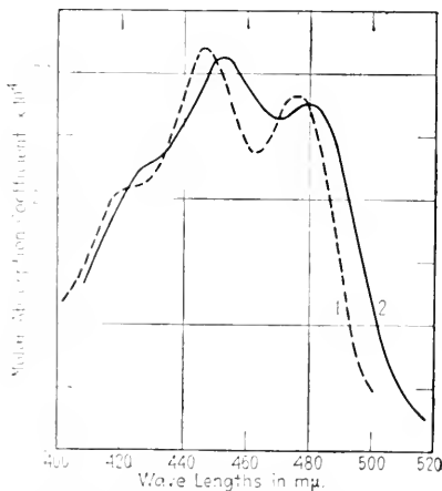
FIG. 6.—Absorption curves of 1, \alpha -carotene; 2, \beta -carotene in 95 per cent ethanol. Molar absorption coefficient,
