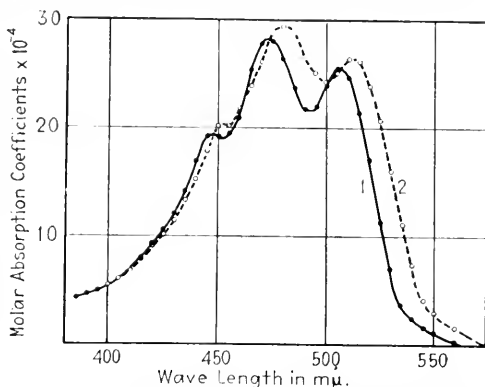
FIG. 5.—Absorption curves in carbon bisulphide of 1, lutein; 2, zeaxanthin. (Kuhn and Smakula, 60.)
