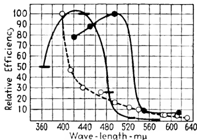
FIG. 4.—Graphs showing the relative efficiencies of different wave-lengths in their phototropic action on Phycomyces blakesleanus (horizontal lines), on Phycomyces nitens after Blaauw (solid circles), and on Pilobolus after Parr (open circles). (From Castle, 16.)
