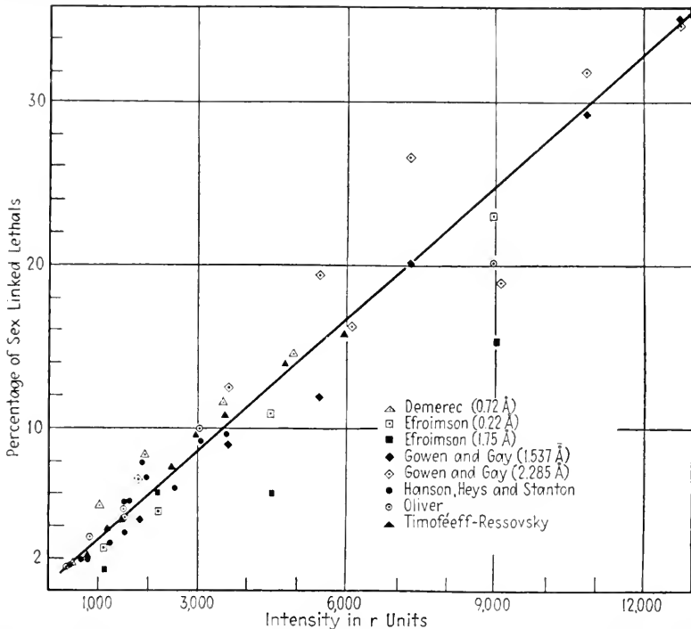
FIG. 6.—Percentage of lethals in the X-chromosome of Drosophila melanogaster in relation to the intensity of radiation. The data are taken from Tables 19 and 19a; for Demerec's values, the dosages of the table have been divided by 0.61. In the case of Gowen and Gay, the intensities have been divided by 2.44. The controls are not indicated; they may be found in Table 9.
