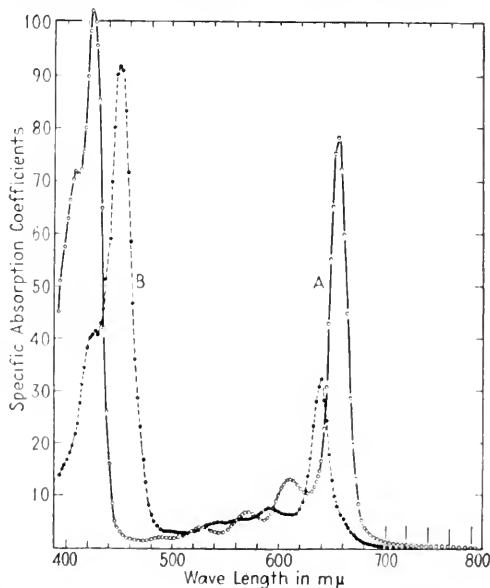
FIG. 4.—Absorption curves in ether of A, chlorophyll a ; B, chlorophyll b . (Zscheile, 153.)
