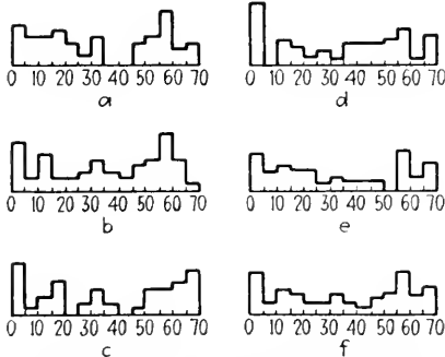
FIG. 5.—The distribution of lethal mutations in the X-chromosome of Drosophila melanogaster . The chromosome, whose genetic map is the abscissa, is divided into regions five units in length. The ordinates are numbers of lethals: (a) 47 lethals, dosage 385 r; (b) 57 lethals, dosage 770 r; (c) 46 lethals, dosage 1540 r; (d) 46 lethals, dosage 3080 r; (e) 37 lethals, dosage 6160 r; (f) 233 lethals, total. (After Oliver, 125.)
