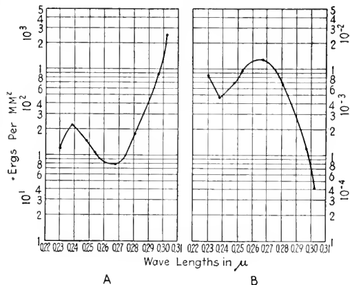
FIG. 1.—A, curve of incident energies involved in the destruction of 50 per cent of B. coli ; B, curve of the reciprocals of A. (From Gates, 60.)
