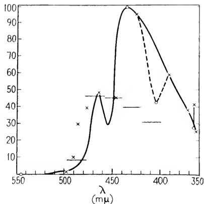
FIG. 3.—Graphs showing the sensitivity of Avena sativa to wave-lengths of light (continuous line) as compared with the corrected values of Blaauw (crosses), of Sonne (circles), and of Königsberger (horizontal lines). (From Bachmann and Bergann, 2.)
