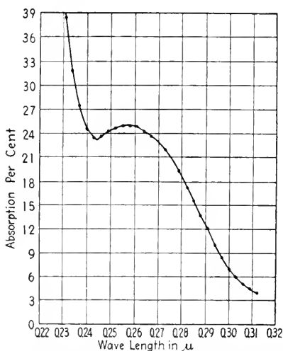
FIG. 2.—The coefficients of absorption of ultra-violet radiation by a layer of B. coli 0.8 μ in thickness. (From Gates, 60.)
