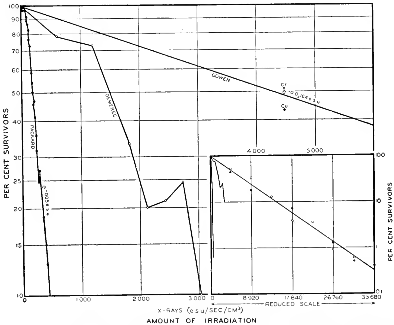
FIG. 4.—Survival curves for Drosophila eggs (at 1 to 3 hr. from laying), chromatin diploid, and sperm, chromatin haploid.
