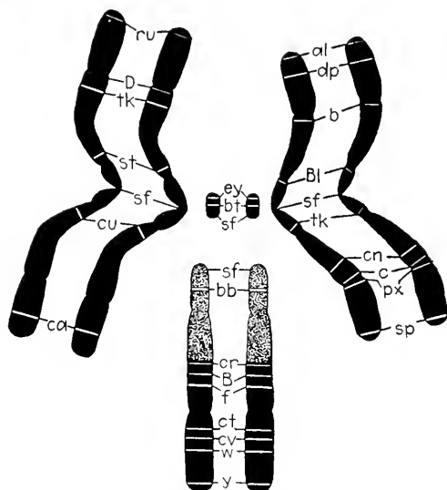
FIG. 4.—Cytological maps of the chromosomes of Drosophila melanogaster , showing the approximate location of various genes and of the spindle fibers ( sf ). The inert region of the X-chromosome represented by the stippled portion of the rod-shaped chromosomes. The longer V-shaped chromosomes (left) are the third chromosomes; the shorter V-shaped chromosomes (right) are the second chromosomes; the smallest pair, the fourth chromosomes.
