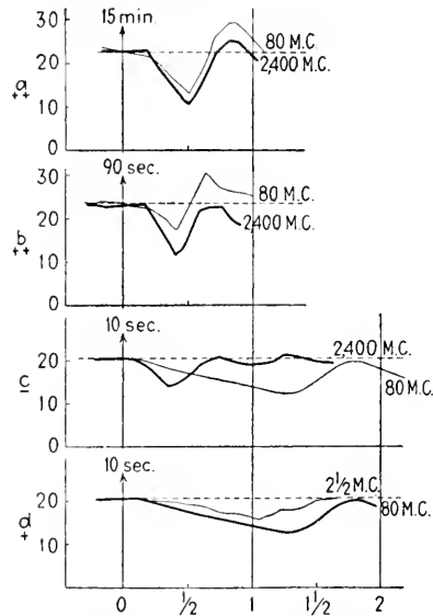
FIG. 1.—Graphs showing growth of Avena sativa . The abscissa represents time in hours and the ordinate rate of growth in microns per minute. The intensity of light is indicated in meter-candles. The light lines represent the growth response for \frac{1}{30} the light intensity of the response represented by the heavy lines. The arrow indicates the moment of illumination with the duration marked above. The predicted phototropic response is indicated by plus and minus signs. (From Dillewijn, 17.)
