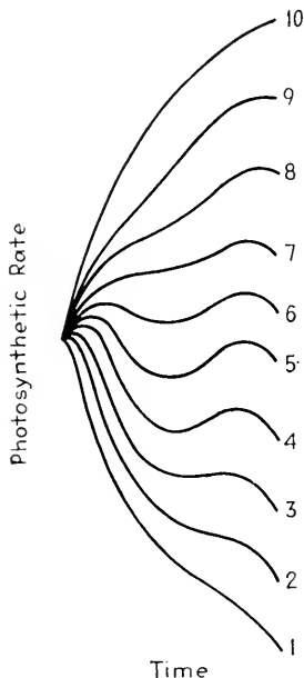
FIG. 8.—Schematic representation of possible curves of photosynthetic rates under constant external conditions, showing the effect of the light intensity under which plants were cultivated. The shape of the curve is dependent upon the ratio of the light intensity used in the cultivation of the plants to that in which the photosynthetic rates are determined. With low intensity of cultivation and high intensity of experiment, low ratio, curve 1 is obtained. With high ratio, curve 10 results. (Harder, 38a.)
