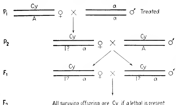
FIG. 2.—An experiment for the detection of lethals in the second chromosome of Drosophila melanogaster . The Cy chromosome eliminates the cross-overs in the female, and usually the homozygote does not survive. Either males or females may be treated, according to this technique; the diagram illustrates an experiment in which males are treated. It should be noted that, in this experiment, use is made of two dominant marking genes ( Cy and A , which may be any one of a number of different dominants).
