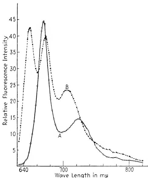
FIG. 7.—Fluorescence spectra in ether of A, chlorophyll a ; B, chlorophyll b . (Zscheile, 154.)
