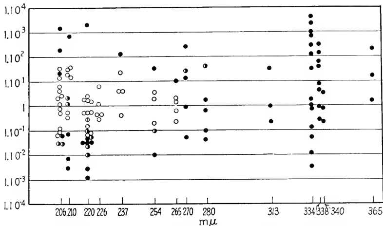
FIG. 4.—Graphic demonstration of the results using yeast as detector and monochromatic light as sender. Outlined circles designate positive effects; half-blocked circles, doubtful cases; blocked circles, zero effects. The ordinates express the intensities in arbitrary units; the abscissas, wave-lengths in millimicrons. (After Chariton, Frank, and Kannegiesser, 48.)
