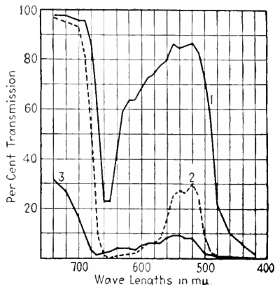
FIG. 1.—Comparative spectral transmission curves for: 1, dilute solution of chlorophyll in acetone; 2, concentrated solution of chlorophyll in acetone; 3, leaf, Sambucus nigra . (Seybold, 104c.)
