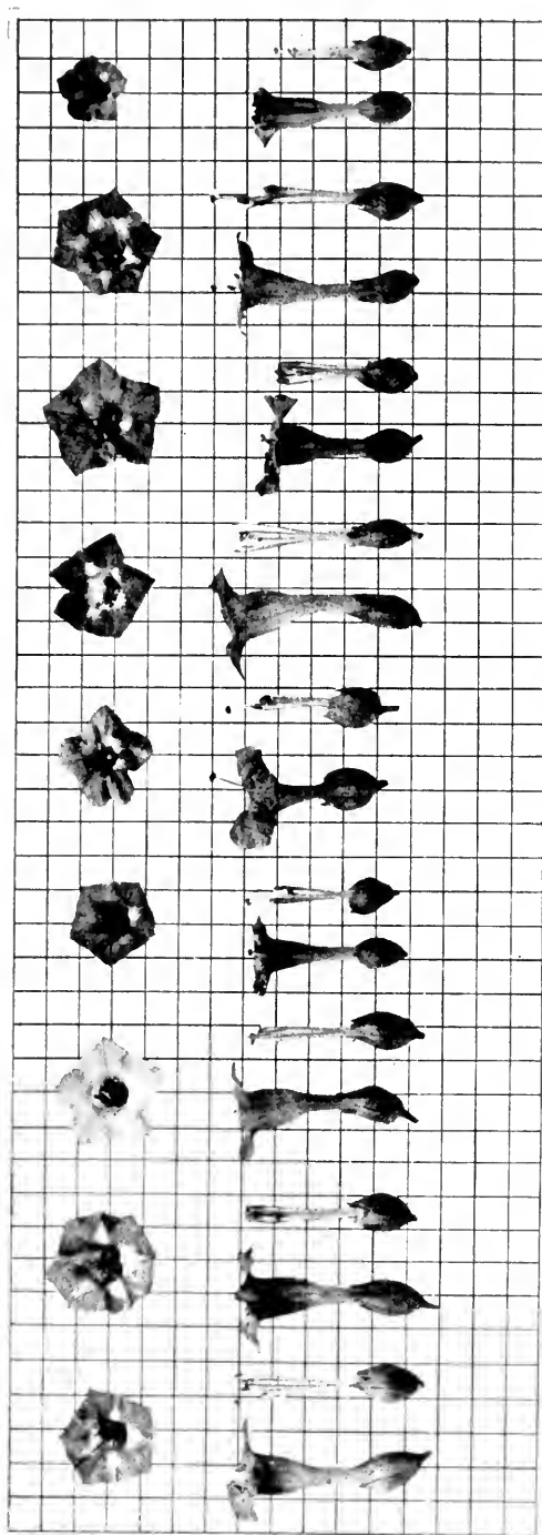
FIG. 3.—Extent of variation in first generation in X-raying of buds of N. Tabacum var. purpurea two days after anthesis, as illustrated by distinction from control (extreme left) in flower size, color, shape and insertion of parts. PMC of buds on the same parent plant at the time of X-raying were in meiosis and the extent of chromosomal alteration induced in them is shown in Fig. 2.
