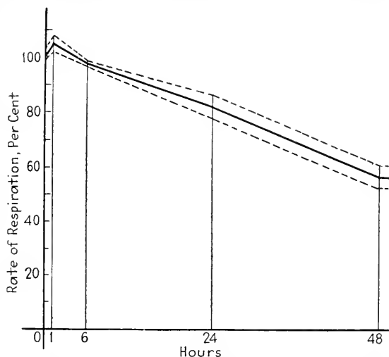
FIG. 2.—Root tips of Vicia Faba ; graphic representation of rate of respiration after radiation with X-rays at 1 H.E.D. Time in hours after irradiation is shown as abscissas and rate of respiration compared with the control (100) is shown as ordinates. Dotted lines represent averages of the probable error. (After Bersa, 1.)
