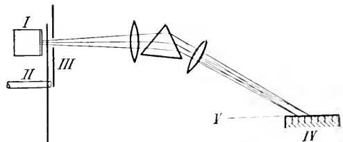
FIG. 5.—Arrangement for spectral analysis of mitogenic radiation. I, source of radiation, in chamber with quartz window; II, rotating disk; III, entrance slit of spectrograph; IV, agar blocks with surface layer of yeast—blocks separated from each other by celluloid strips. (After Gurwitsch, 108.) Newer experimental arrangements have a very well adjusted exit slit.
