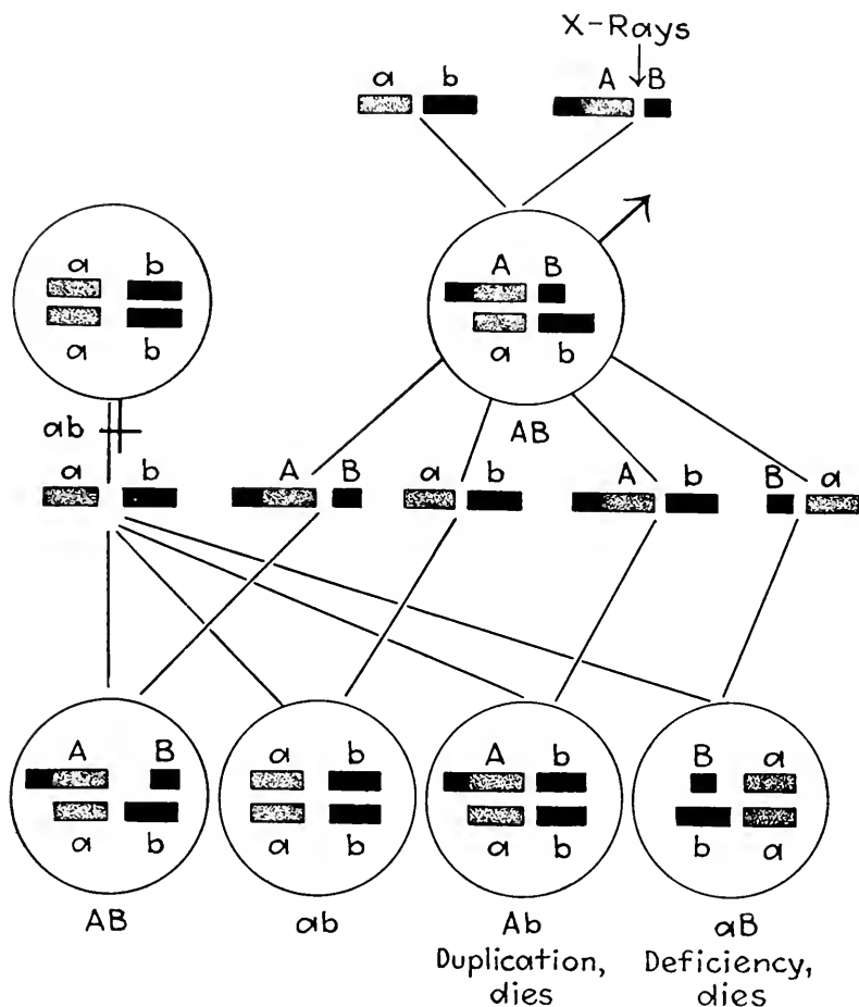
FIG. 1.—Scheme of the detection of a translocation. Genes A and B behave normally independently since they are located in different chromosomes (one of which is represented black and the other stippled). In individuals carrying a translocation involving these chromosomes the genes A and B exhibit linkage, since gametes Ab and aB produce no viable zygotes.
