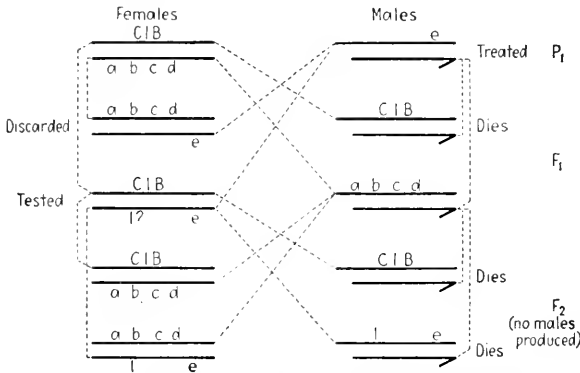
FIG. 1.—The Cl B technique for the measurement of lethal mutation rate in the X-chromosome of Drosophila melanogaster . This method is especially adapted for the detection of the effects of environmental agents on the male, since the tested X-chromosome is paternal. The lethal in the Cl B chromosome kills all males which carry it; the other X-chromosomes are generally distinguished by the use of marking genes, here denoted by the letters a, b, c, d, e .
