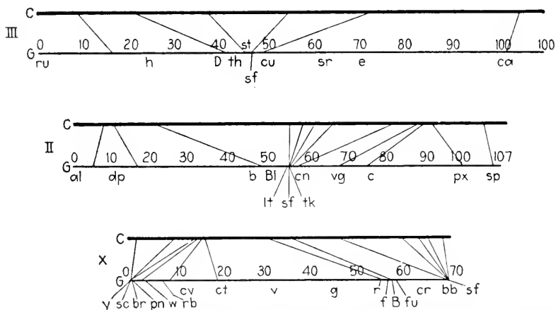
FIG. 5.—Comparison of the genetic and cytological maps of the third (III), second (II), and X -chromosomes ( X ) of Drosophila melanogaster . C , the cytological map; G , the genetic map. Figures indicate the genetic distances in map units.
