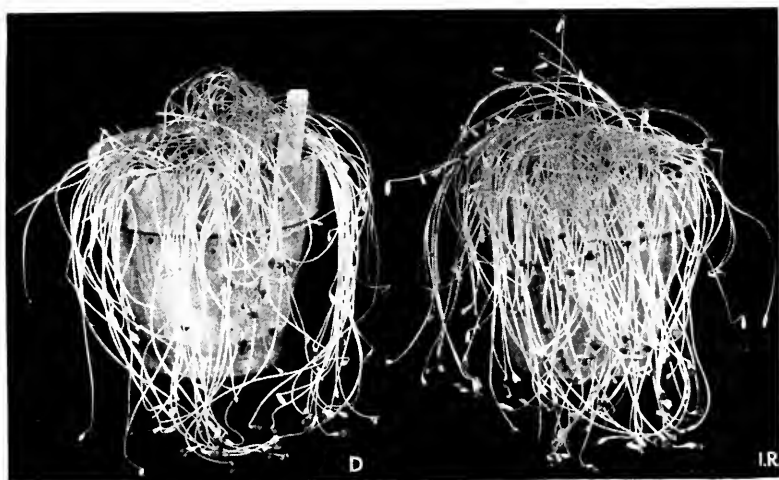
FIG. 1.—Buckwheat seedlings. D , at left, grown in darkness. I.R. , at right, received only the infra-red of sunlight. Note that there is no difference in the appearance of the two. The green pigment chlorophyll does not develop under infra-red.
