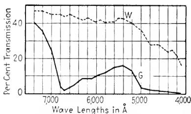
FIG. 2.—Transmission spectra of leaves, Acer negundo : W, white leaf; G, green leaf. (Seybold, 104c.)
