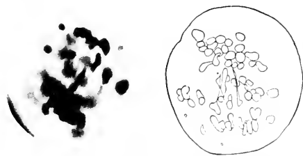
FIG. 2.—Chromosomal disruption appearing in first meiotic anaphase of PMC of Nicotiana Tabacum var. purpurea , 48 hr. after heavy X-radiation. (a) Photomicrograph; (b) camera lucida drawing of same PMC.
