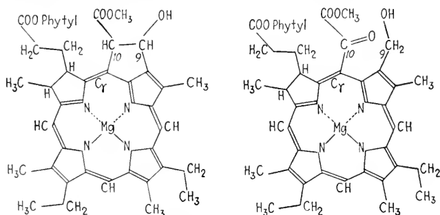
FIG. 9.—Structural formulas of chlorophyll a (left) and chlorophyll b (right). (Stoll and Wiedemann, 119.)
