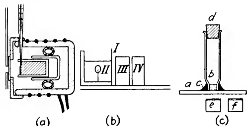
FIG. 2.—Three arrangements for gastight isolation of mitogenetic sources. (a) Incubator chamber with quartz window (after Baron); (b) chamber with quartz window: I, quartz plate; II, tumor; III, detector; IV, control; (c) chamber (after Blacher): a, quartz plate; b, radiating material; c, cement; d, stopper; e, detector; f, control. (Gurwitsch, 108.)
