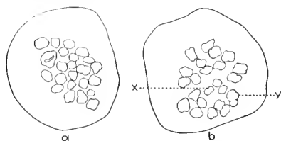
FIG. 5.—Cytological evidence of induced chromosomal interchange and reorganization in N. Tabacum var. purpurea . (a) Ring of four chromosomes at first meiotic metaphase in F_1 of type shown in Fig. 4b, crossed with control. (b) First meiotic metaphase in type shown in Fig. 4c: 21 bivalents, 1 fragment pair (x), and 1 trivalent (y).
