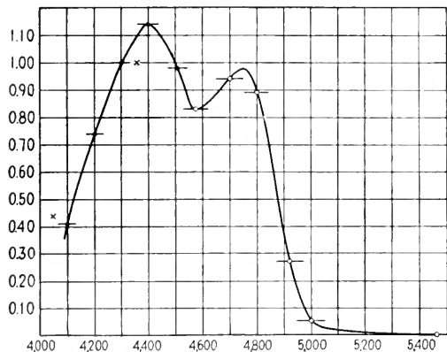
FIG. 5.—Graph showing phototropic sensitivity curve. The ordinates are relative sensitivity values, the abscissas, wave-lengths in Angströms, and the horizontal bars indicate the wave-length ranges of the balance points. Circles indicate points obtained with filters combined with the monochromator. The crosses show where mercury lines were used. (From Johnston, 23.)
