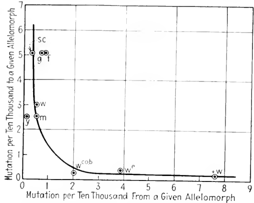
FIG. 4.—The relation between the frequency of mutation to a given allelomorph, and its own mutation rate to other allelomorphs. It should be noted that the probable errors of such low values are in themselves relatively large. Moreover, the data for the white locus (Table 4), from Timoféeff-Ressovsky (183); for the other loci (Table 5), from Johnston and Winchester (76), are in themselves subject to error which can not be properly evaluated. Different allelomorphs are not separated, and heterogeneous data are lumped. Each point on the curve represents the frequency of mutation to a given gene in all the available data. A full discussion of the questions involved cannot be given here; but the discovery of the possibility of a general rule for such occurrences seems interesting enough for presentation.
