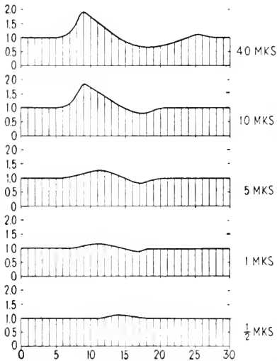
FIG. 2.—Graphs showing growth response of sporangiophores of Phycomyces for different light quantities indicated in meter-candle-seconds. The growth rate in darkness is taken as unity. (From Wiechulla, 45.)
