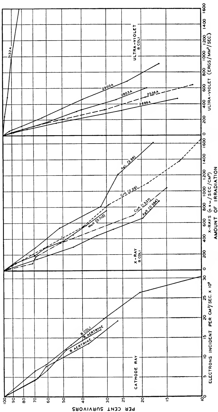
Fig. 1.—Survival curves of B. coli exposed to radiation, cathode, X-ray, and ultra-violet.
