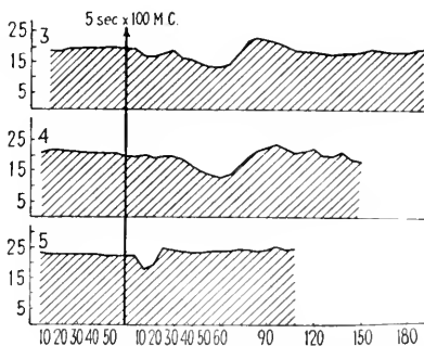
FIG. 6.—Graphs showing light-growth response of Arca . The ordinate represents growth in microns per minute, the abscissa time in minutes, the arrow the moment of illumination. Graph 3, illumination of entire coleoptile (12 mm. long); Graph 4, illumination of the tip (1.25 mm.); Graph 5, illumination of base (9 mm.) while the top (3 mm.) is kept in darkness. (From Went, 42.)
