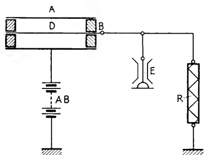
FIG. 3.—Diagram of Geiger-Müller counter. A, counting chamber; B, insulating stopper; AB, batteries; E, electrometer; R, resistance; D, anode wire. (After Rajewsky, 224.)
