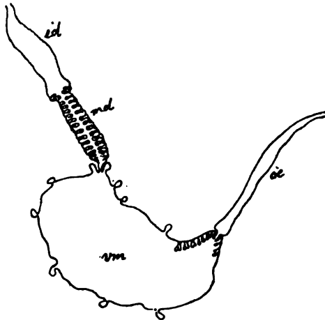
Darmtraktus eines jungen Exemplars von Xenogaster inflata (38: 1). oc = Oesophagus; vm = Vormagen; md = Mitteldarm; ed = Enddarm.
