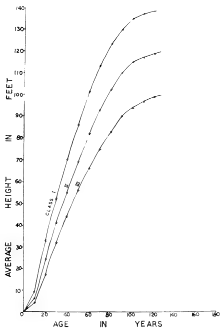
Figure 4. Average height growth of moist upper level blue pine class I (avg. ht. 120'-140'); II (avg. ht. 100'-120'); and III (avg. ht. 80'-100'), 90-year-old trees.
