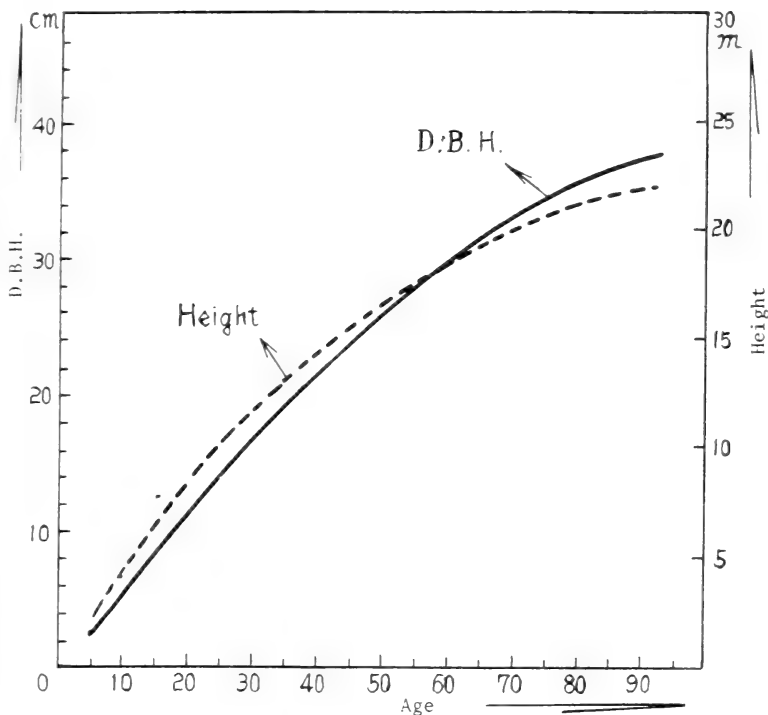
Figure 24. Height and diameter growth of an average Pinus armandii in a natural stand on Mt. Alishan, Taiwan. Drawn from data provided by Mr. Jih-Ching Liao, Assistant Professor of Dendrology, Taiwan University, Taipei, Taiwan.
