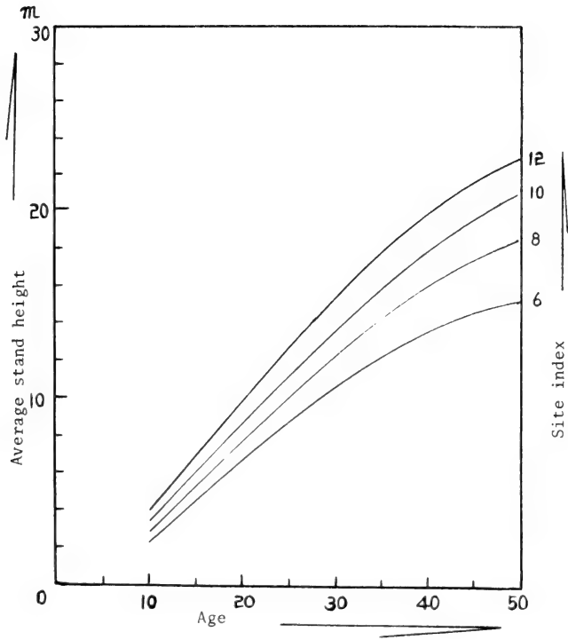
Figure 13. Relation between age, site index and average height for a well stocked stand of Pinus koraiensis .
