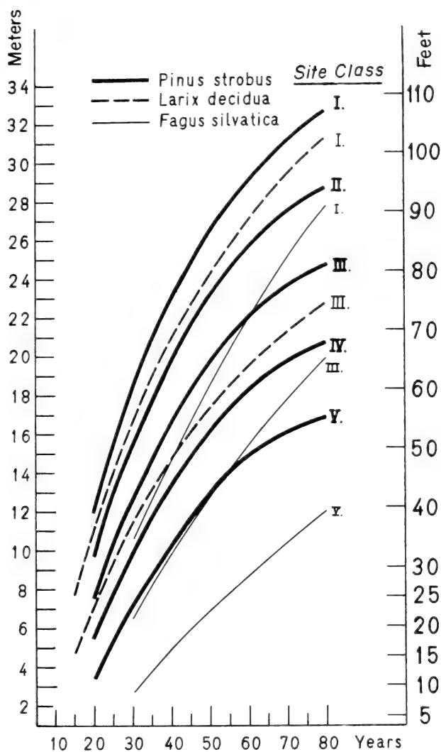
Figure 1. Average height of Pinus strobus on various sites, compared with that of Larix decidua and Fagus silvatica , Odenwald Mountains, state of Hesse, Germany (after Eckstein, in press).
