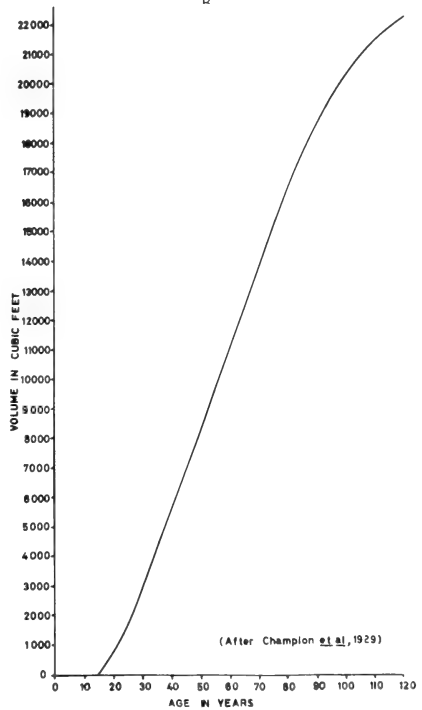
Figure 5. Growth curves for Pinus wallichiana on site quality I and II, in the Murree area of the mesic zone; A. height-age, B. diameter-age, C. basal area-age, and D. volume per acre-age.
