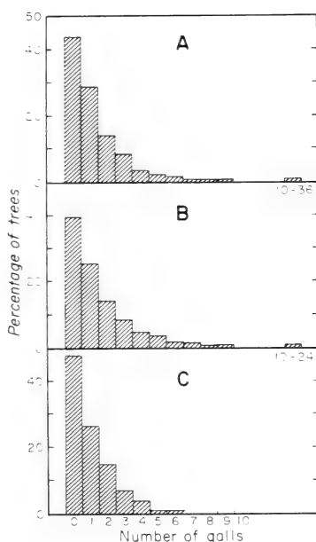
Figure 1.--Frequency distribution of individual loblolly pines into categories according to the number of separate infections (galls) sustained by each. (A) 7-year-old trees (total: 3,918) from 48 open-pollinated families; (B) 4-year-old trees (total: 1,376) from 54 controlled-pollinated families; (C) 4-year-old trees (total: 318) from bulk seedlot, unknown parentage. (Data for C courtesy of the U.S. Forest Service, Macon, Ga.)
