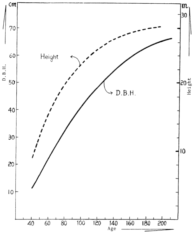
Figure 11. Height and diameter growth based on a single tree of Pinus koraiensis in a natural stand in northern Korea.
