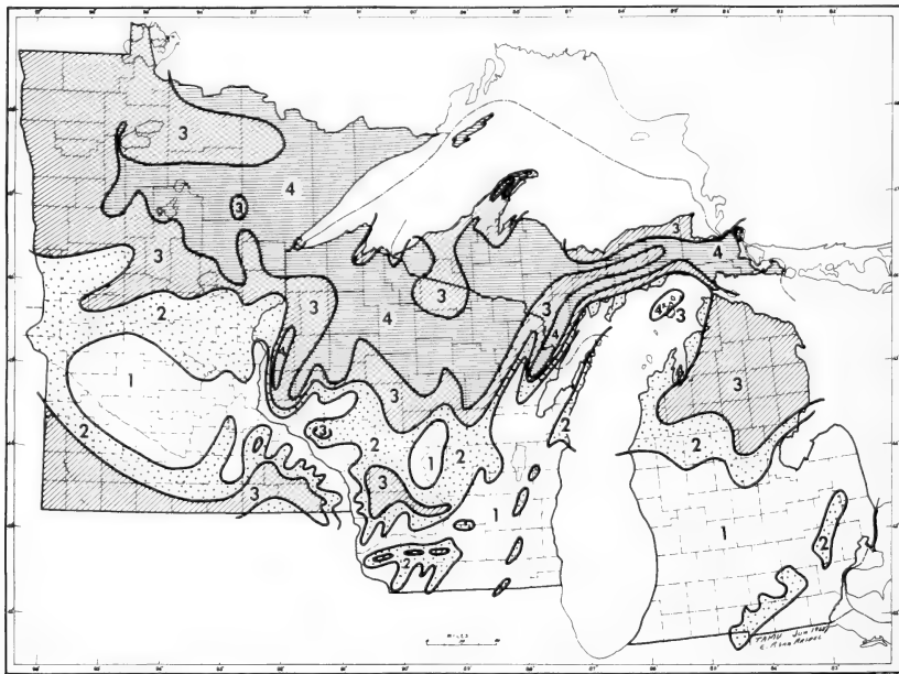
Figure 2. Map showing differences in quantity of blister rust spread to white pines in the Lake States. Rust in tops of emergent pines carried from distant ribs are characteristic of Zone 4. The cooler the summer weather, the more favorable for disease spread.
