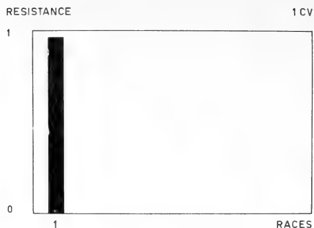
Figure 5. The "one race - one cultivar" interaction, with resistance nearly complete.
