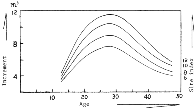
Figure 16. Current annual increment curve of major trees (volume per ha in cubic meters) of Pinus koraiensis .
