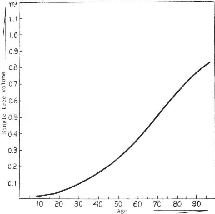
Figure 25. Volume growth of an average Pinus armandii in a natural stand on Mt. Alishan, Taiwan. Drawn from data provided by Mr. Jih-Ching Liao, Assistant Professor of Dendrology, Taiwan University, Taipei, Taiwan.
