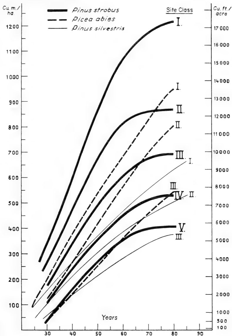
Figure 2. Wood yield of Pinus strobus on various sites, compared with that of Picea abies and Pinus silvestris , Odenwald Mountains, state of Hesse, Germany (after Eckstein, in press).
