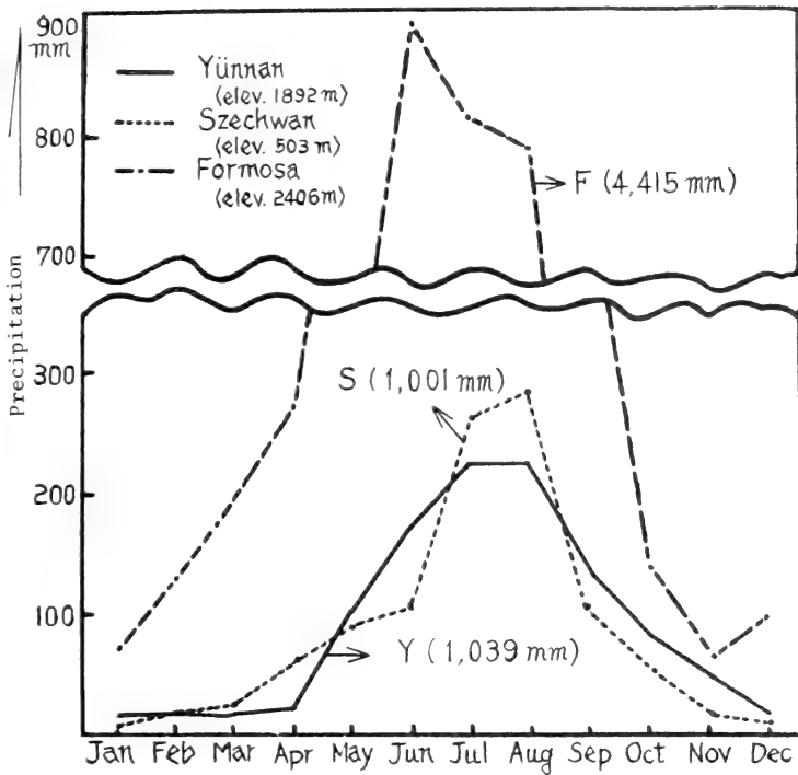
Figure 21. Distribution of precipitation over the range of Pinus armandii .
