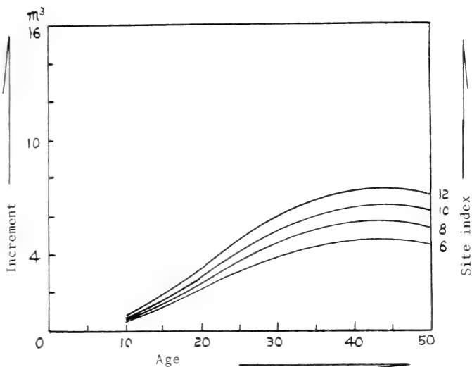
Figure 17. Mean annual increment curve of major trees (Volume per ha in cubic meters) of Pinus koraiensis .
