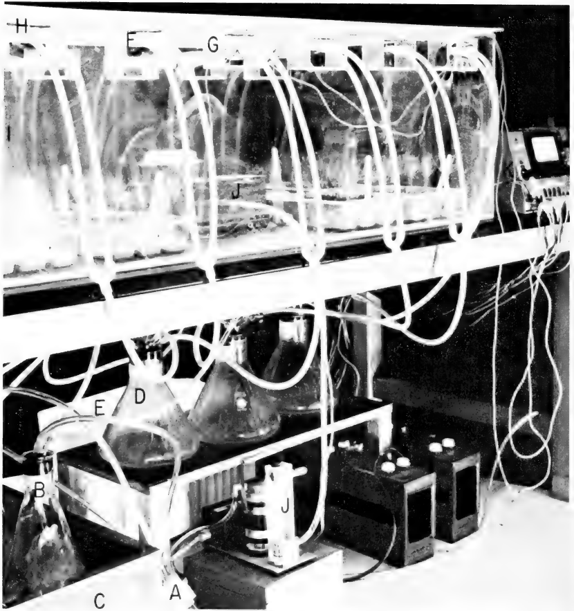
Figure 1. Apparatus for inoculating pine seedlings. Basidiospores of Cronartium fusiforme abjected from telia on oak leaves (H) suspended over the internal ports (G) are carried by a stream of moist air into the inoculation chamber (I) containing the pine seedlings. Other components of the system are the air-streams (A) to the humidification flasks (B) held in a constant temperature (34 C) water bath (C), air-mixing flasks (D), cold water bath (5-10 C) (E), modified Nalgene "T's" (F), Kramer-Collins spore sampler (J), and scanning tele-thermometer (K).
