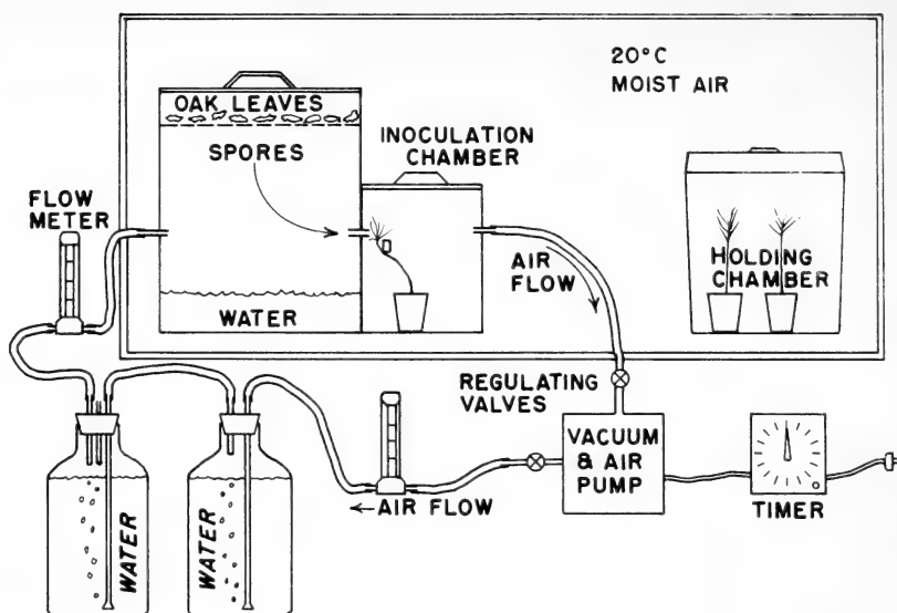
Figure 1. Apparatus for inoculating pine seedlings. Basidiospores of Cronartium fusiforme released from telia on oak leaves in the large compartment are carried by a stream of moist air through the connecting tube to the tree in the small compartment.
