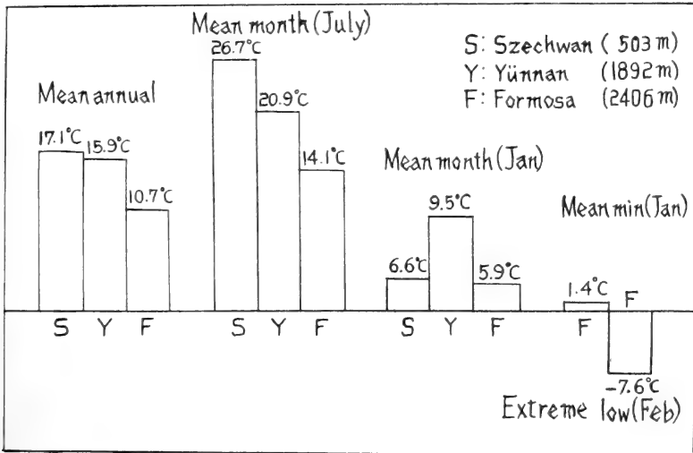
Figure 22. Range of temperature over the natural range of Pinus armandii .
