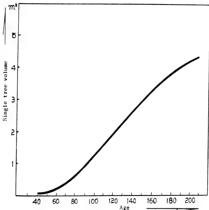
Figure 12. Volume growth based on a single tree of Pinus koraiensis in a natural stand in northern Korea.
