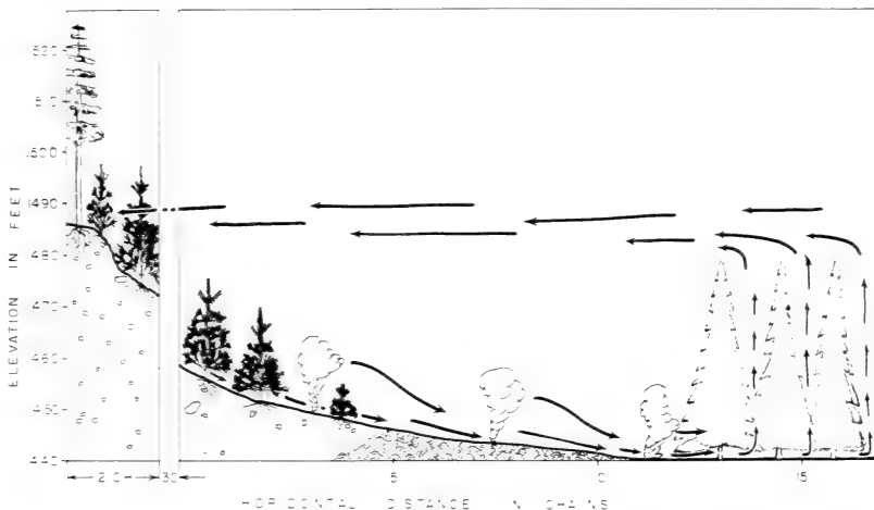
Figure 7. Pattern of airflow that controls rust spread around a swamp edge.
