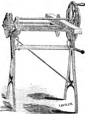
Hand Circular Ripping Saw, $50.
