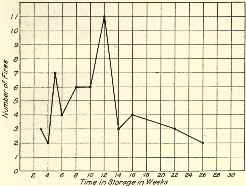
FIG. 33. GRAPH SHOWING LENGTH OF TIME COAL WAS IN STORAGE WHEN FIRE WAS DISCOVERED (CHICAGO COAL PILE FIRES, CLASS 3)
