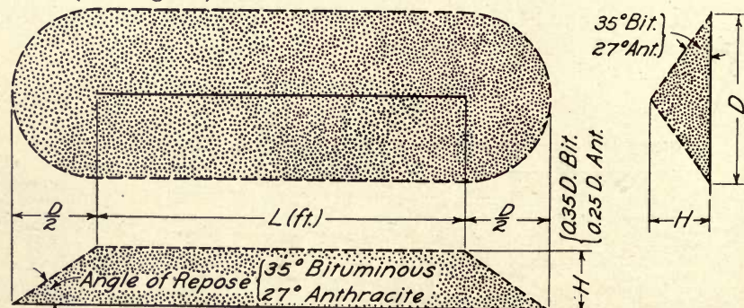
FIG. 75. DIMENSIONS FOR DETERMINING VOLUME AND WEIGHT OF COAL PILES
