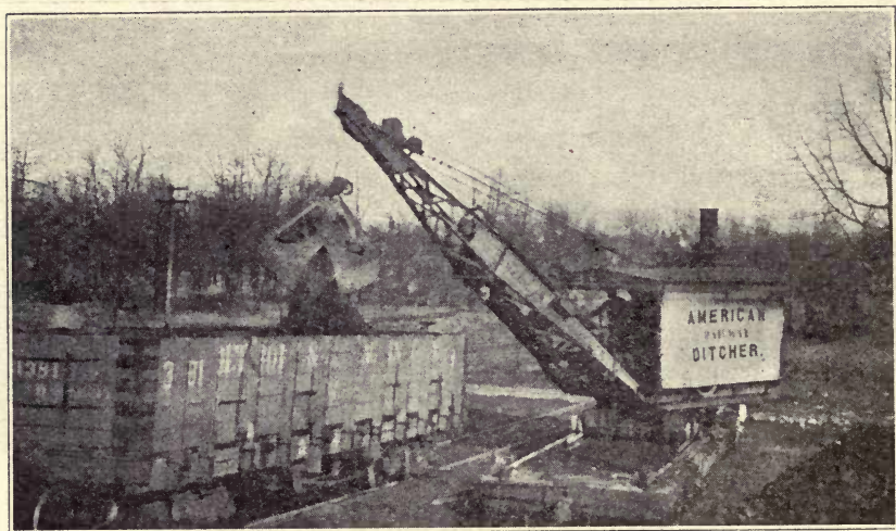
FIG. 39. DITCHER RECLAIMING COAL
