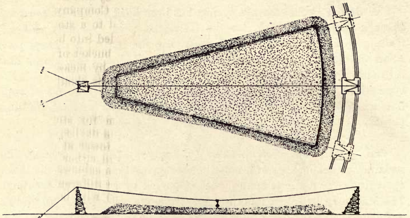
FIG. 66. CABLEWAY SYSTEM FOR HANDLING COAL—ONE END TOWER FIXED, THE OTHER MOVABLE
