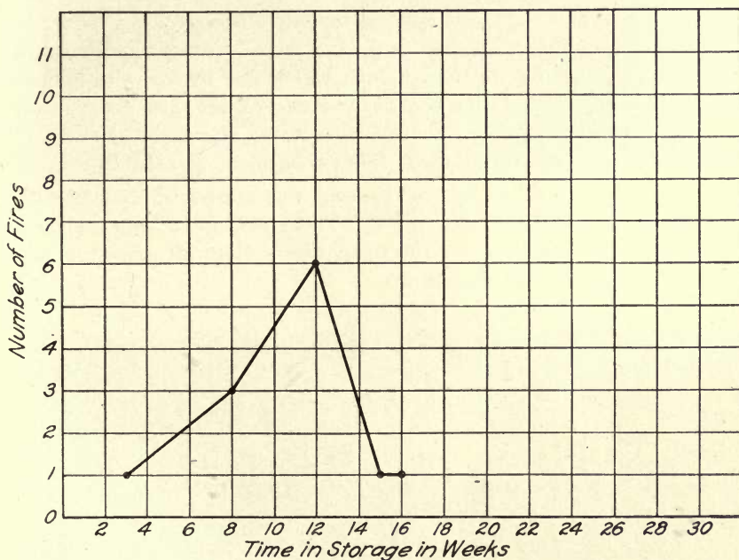
FIG. 15. GRAPH SHOWING LENGTH OF TIME COAL WAS IN STORAGE WHEN FIRE WAS DISCOVERED (CHICAGO COAL PILE FIRES, CLASS 1)
