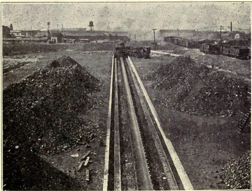
FIG. 61. VIEW OF COAL STORAGE PLANT OF THE ERIE RAILROAD, BUFFALO, NEW YORK, SHOWING LOADER AT END OF CONVEYOR NO. 2
