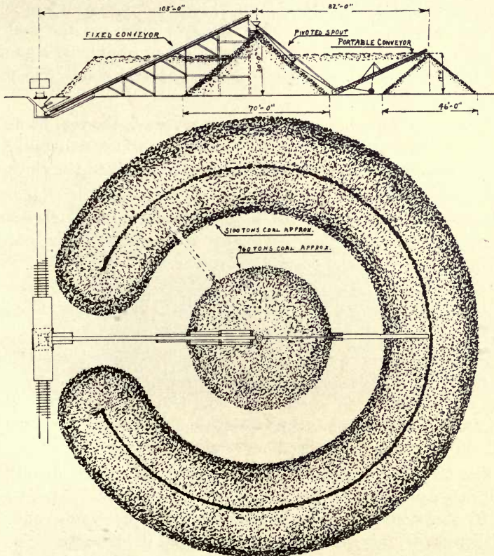
FIG. 48. CIRCULAR METHOD OF PILING COAL, USING BOTH PORTABLE AND SEMI-PORTABLE CONVEYORS — PLAN AND SECTION
