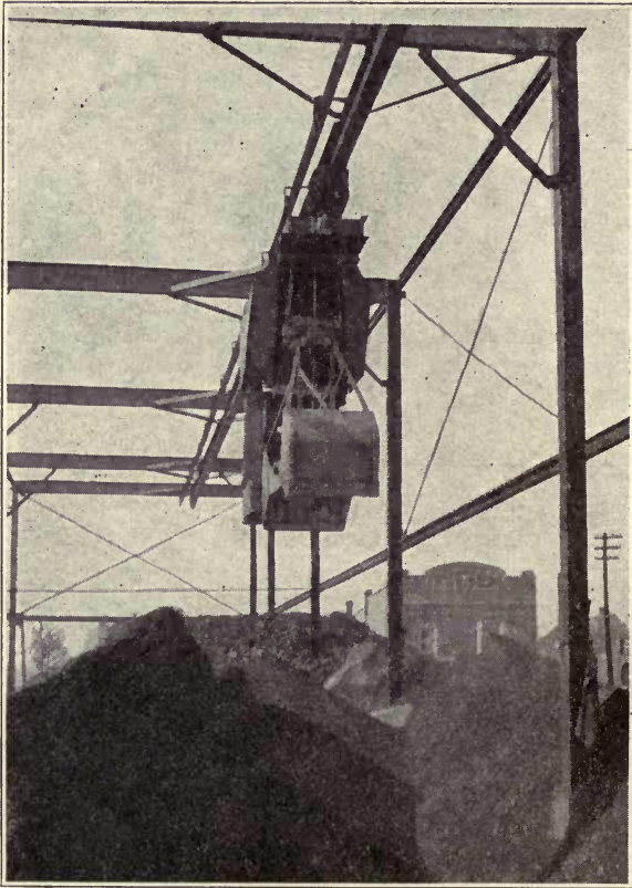
FIG. 63. MONORAIL SYSTEM FOR STORING AND RECLAIMING COAL
