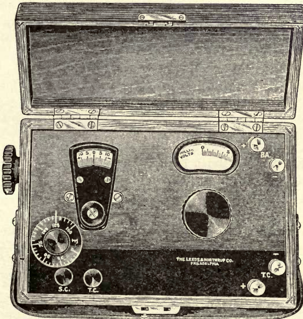
FIG. 8. INDICATING PYROMETER — POTENTIOMETER TYPE
