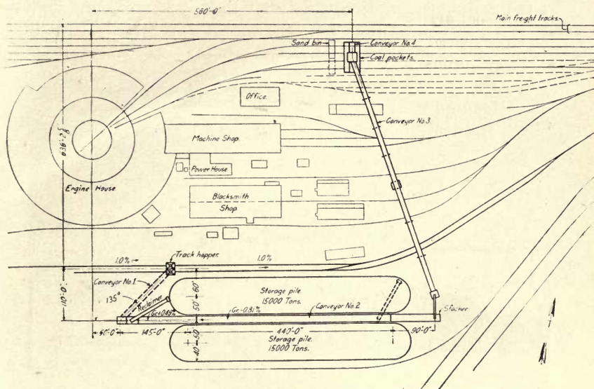
FIG. 59. PLAN OF COAL STORAGE PLANT OF THE ERIE RAILROAD, BUFFALO, NEW YORK
