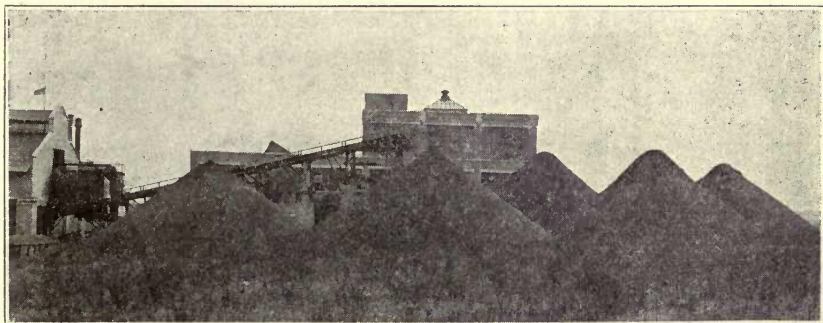
FIG. 49. COAL STORAGE PLANT USING FIXED AND PORTABLE CONVEYORS AT MOOSEHEART, ILLINOIS
