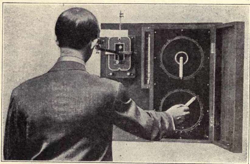
FIG. 5. ZELENY THERMOMETER SYSTEM—READING INSTRUMENT AND SWITCH BOARD
