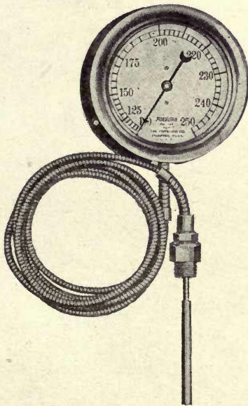
FIG. 4. INDICATING THERMOMETER — LONG DISTANCE TYPE
