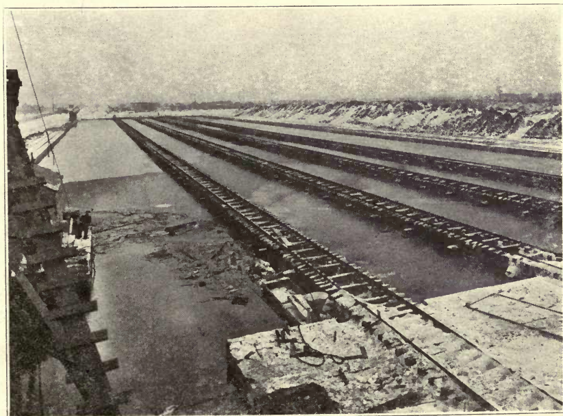
FIG. 72. UNDERWATER COAL STORAGE PLANT OF THE STANDARD OIL COMPANY, WHITING, INDIANA (100 000 TONS CAPACITY)
