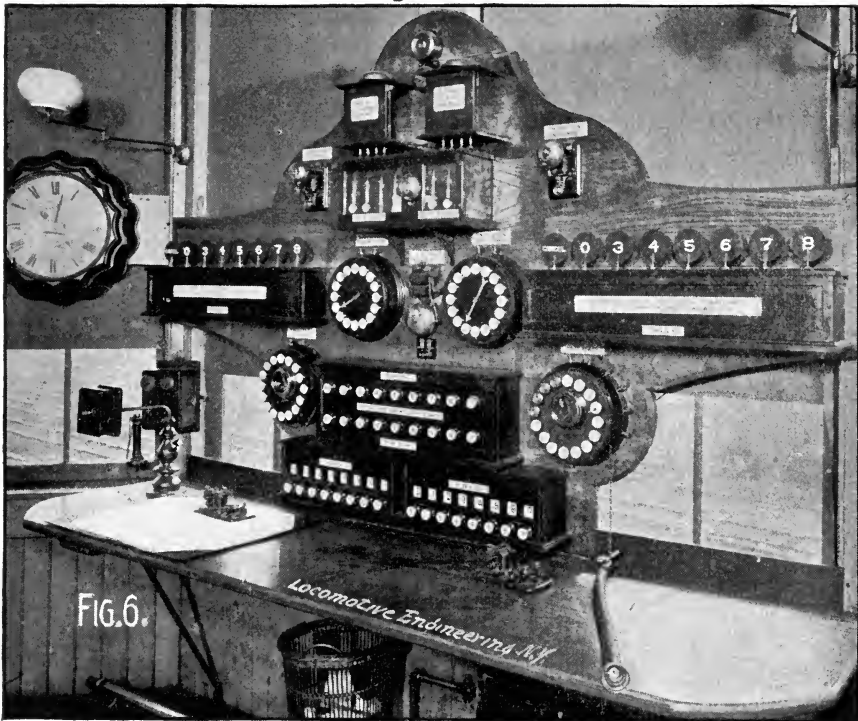
FIG. 6. ELECTRICAL ANNUNCIATOR AND INDICATOR INSTRUMENTS IN P. R. R. TOWER.
