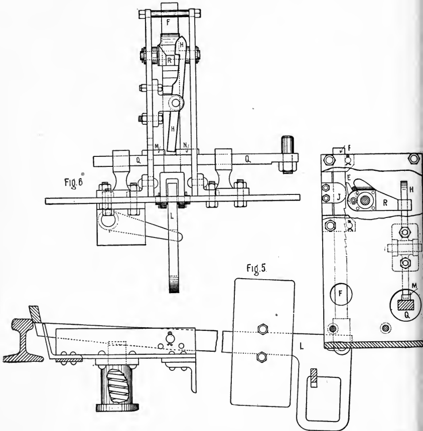
LATCHING DEVICE.
