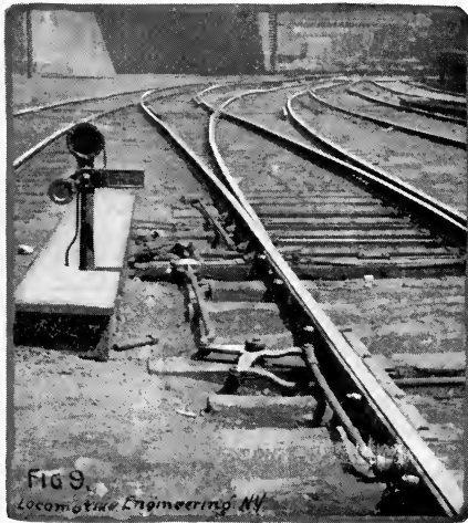
A DWARF SIGNAL.
