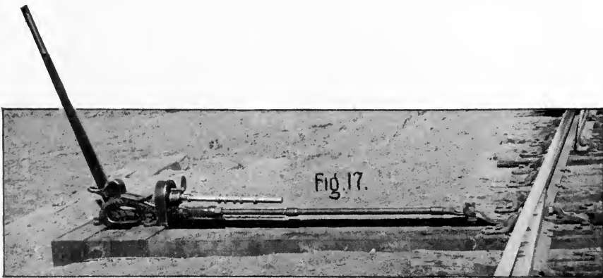
SWITCH UNLOCKED AND THROWN.
