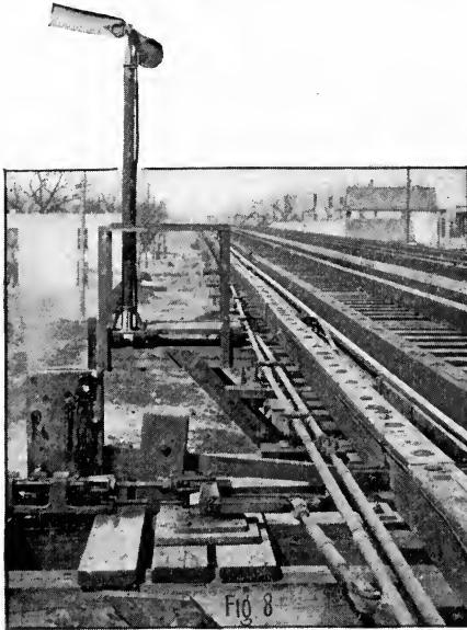
ROWELL-POTTER AUTOMATIC MECHANICAL SIGNAL AT "DANGER."
