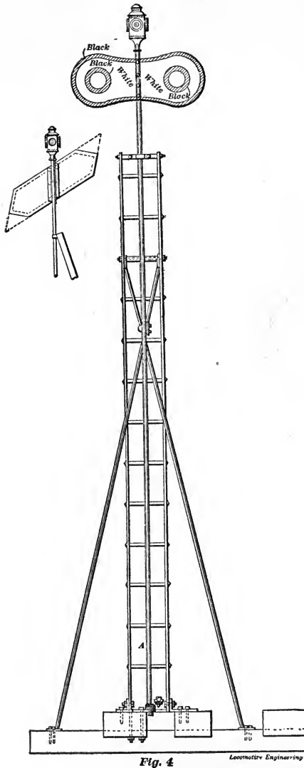
HIGH TARGET STAND GIVING TWO INDICATIONS.
