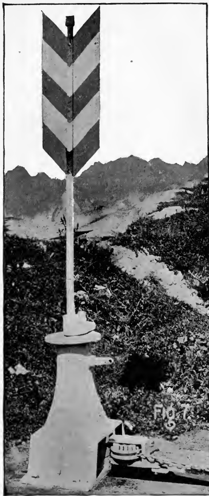
GIBBS' INTERLOCKING SWITCH STAND AT "DANGER."
