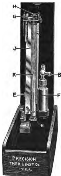
FIG. 6.—New Nicholson Princo sphygmomanometer. B , connection for nipple from cuff and inflation apparatus; F , steel mercury reservoir; G , metal stopcock; K , lower tube section; J , folded metal scale; H , clapper to close lower tube; N , metal cap to prevent escape of mercury; E , cam to lock scale at level of mercury.
