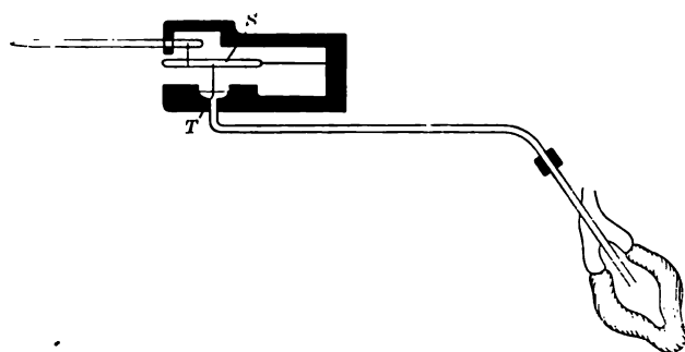
FIG. 4.—Diagram of Hürthle manometer. Tubing from heart or vessel to small tambour T , both filled with fluid. Movements of tambour magnified by compound lever S , and transmitted to writing pen. (From Howell.)
