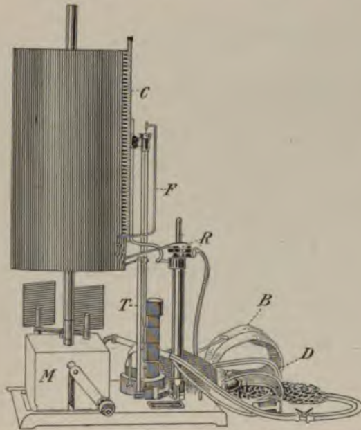
FIG. 42.—Silbermann's tonograph: B , brachial cuff; D , radial cuff; R , radial pulse recorder; T , time marker; F , float, indicating height of mercury in manometer; C , comb to mark 5 mm. spacings on kymograph; M , driving mechanism.
