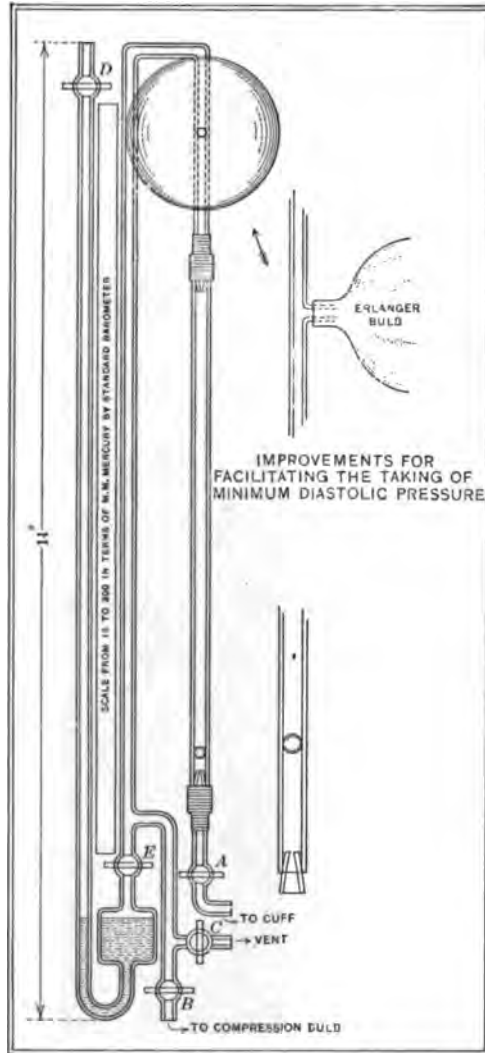
FIG. 53.—Fedd's oscillometer. This instrument has been modified by R. L. Hoobler by using two cuffs with a stopcock connection between them, in circuit with the pith-ball indicator. This permits the reading of the systolic as well as the diastolic pressure, and yields better results in infants (Nicholson). This oscillatory device may be used in conjunction with many types of instruments. It is furnished (at an extra cost) with the Nicholson and the Faught sphygmomanometers.
