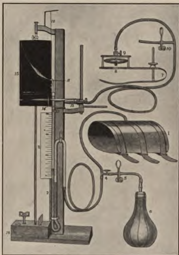
FIG. 36.—Gibson's sphygmomanometer. The recording sphygmomanometer described in the text: 1, armet; 2, manometer; 3, scale; 4, valve for regulating pressure; 5, clip, acting as a valve to syringe; 6, inflation syringe; 7, support for transmission sphygmograph; 8, pelotte; 9, screw for adjusting sphygmograph to artery; 10, clip for arranging pressure; 11, recording lever of manometer; 12, weighted thread for adjusting lever; 13, tambour recording movements of transmission sphygmograph; 14, arm marking abscissa; 15, revolving cylinder; 16, clock-work.
