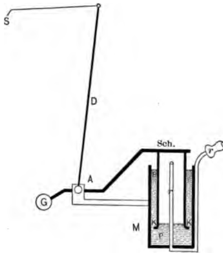
FIG. 48.—Strauss-Fleischer device for damping the force of the pulse wave.
