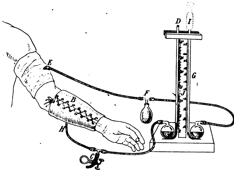
FIG. 67.—Howell's venous pressure apparatus. Upper and lower cuffs applied and attached to their respective water columns. E , light cuff for constricting upper arm and obstructing venous return; F , glass T and bulb, by means of which pressure is raised in E ; G , water column measuring pressure in E ; B , inelastic covering of light material encircling rubber bag; C , glass T, side tube, and clip, by means of which pressure can be raised; D , water column measuring pressure.
