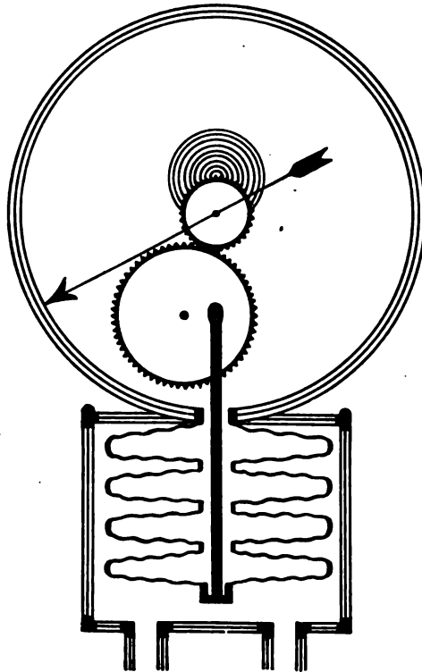
FIG. 59.—Showing the construction of the Faught aneroid.
