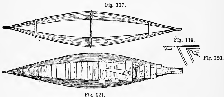
Fig. 121. Top view with sides in place, also reversed view showing how bottom boards are laid.
