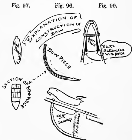
Fig. 98. Fig. 100. Figs. 97-100.—Show details of canoe bow.
