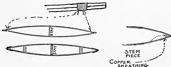
Fig. 118. Top views of dory and parts of dory.
