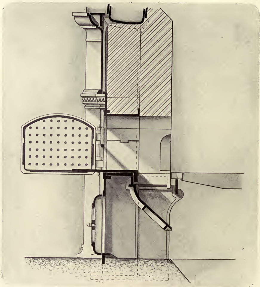
SECTION THROUGH FURNACE FRONT,
