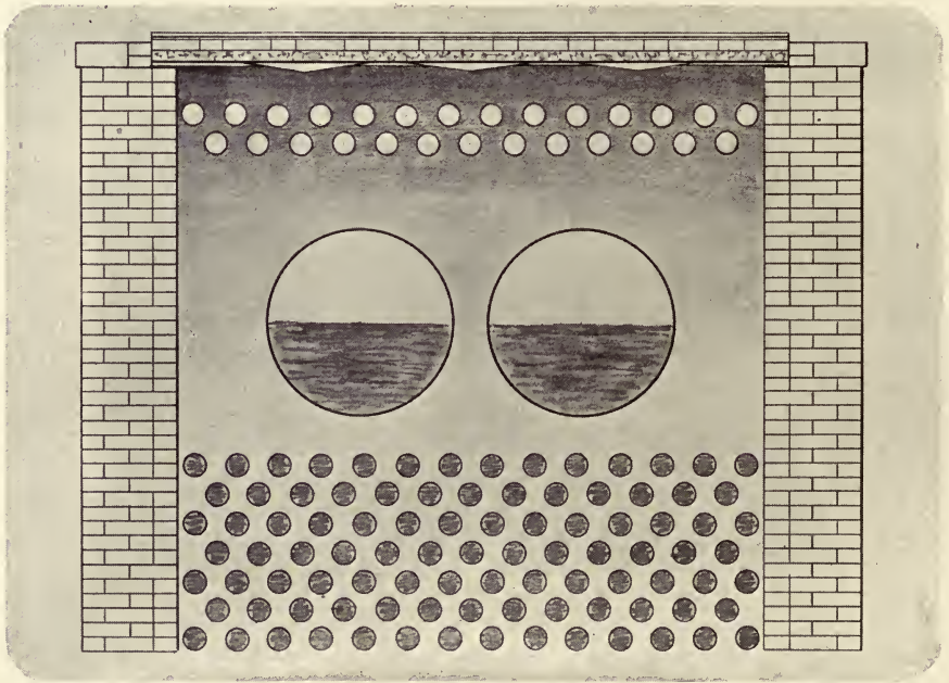
SECTION THROUGH BOILER SETTING.
