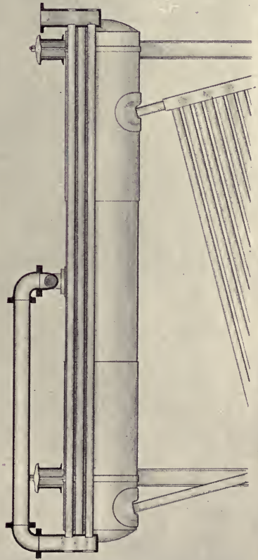
EDGE MOOR SUPERHEATER ATTACHED TO A WATER-TUBE BOILER.
