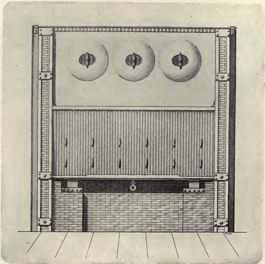
REAR ELEVATION, EDGE MOOR WATER-TUBE BOILER.
