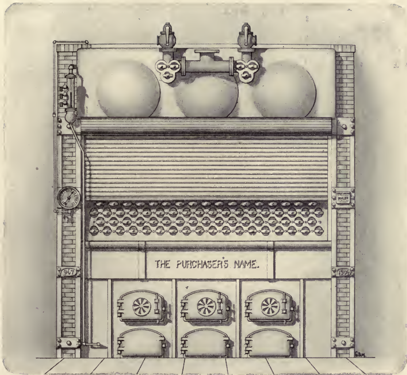
Front Elevation Three-Drum Boiler.
