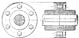
Skivkoppling.
