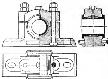
Normallager (stålager).
