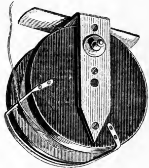
FIG. 4. NOTTINGHAM REEL WITH MOVABLE CHECK AND IMPROVED LINE-GUARD.
