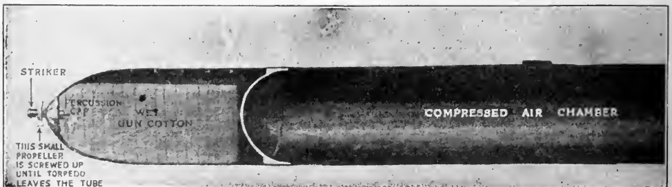
This diagram of a torpedo shows its two forward parts, the head containing the charge and the air-flask.
