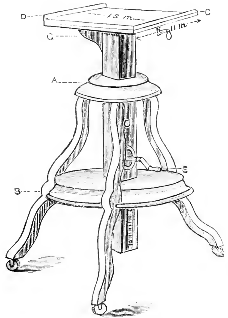
Fig. 100.—STUDIO CAMERA STAND.
