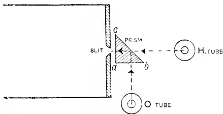
Fig. 707.—COMPARISON PRISM FOR COLLIMATOR.
