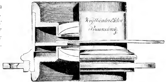
Fig. 756.—VOIGTLÄNDER'S WIDE-ANGLE EURYSCOPE.
