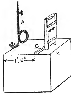
Fig. 321.—HOME-MADE DEVICE FOR RAPID PRINTING.
