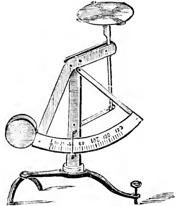
Fig. 387.—DARK-ROOM BALANCE.
