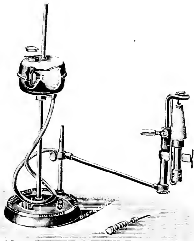
Fig. 457.—THE "SOL" SPIRIT LAMP.
