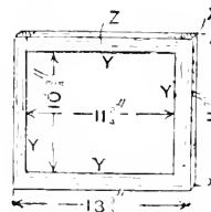
Fig. 62.—FOCUSING SCREEN FRAME.
