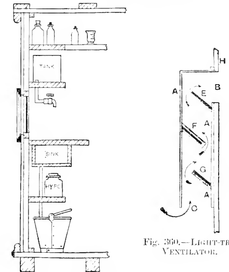
Fig. 359.—FITTINGS OF PORTABLE DARK-ROOM.
