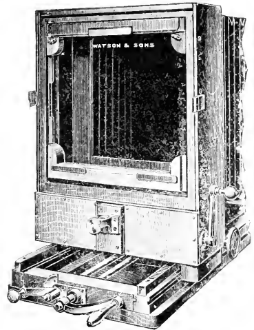
Fig. 898.—BACK VIEW OF WATSON'S PROCESS CAMERA, SHOWING SCREEN GEAR.
