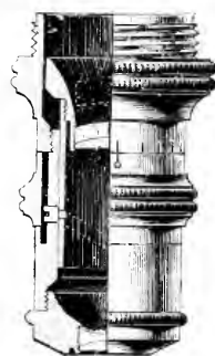
Fig. 692.—ZEISS OBJECTIVE WITH CORRECTION COLLAR.
