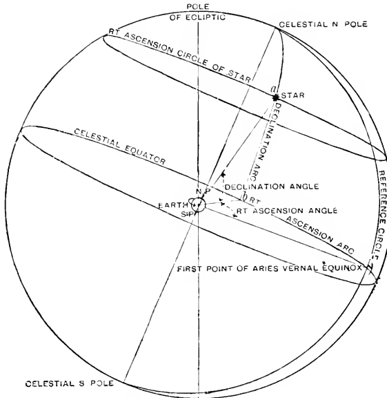
Fig. 803.—THE CELESTIAL SPHERE.
