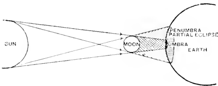
Fig. 812.—UMBRA CAUSED BY SOLAR ECLIPSE.
