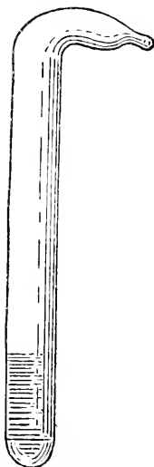
Fig. 554.—SILVER CHLORIDE IN SEALED TUBE.
