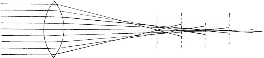
Fig. 489.—SPHERICAL ABERRATION.
