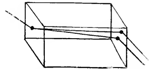
Fig. 717.—DOUBLE REFRACTION WITH ICELAND SPAR.
