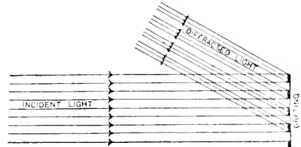
Fig. 774.—DIFFRACTION BY REFLECTION AT A PLANE GRATING.
