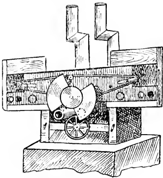
Fig. 550.—APPARATUS FOR D'ALMEIDA'S ECLIPSE SYSTEM.
