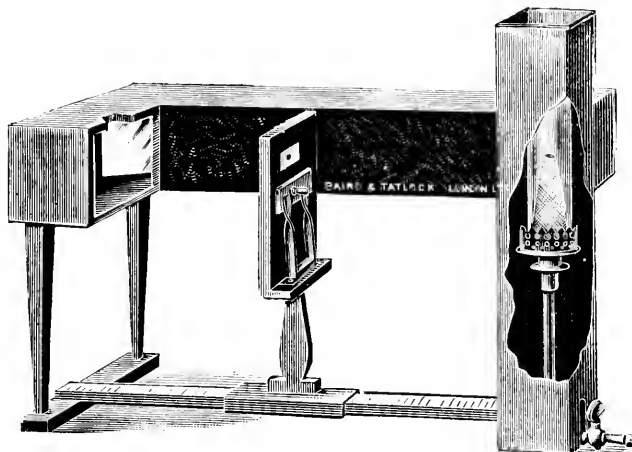
Fig. 566.—THE CHAPMAN JONES OPACITY METER.
