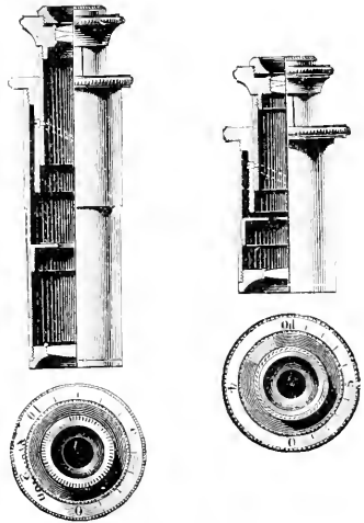
Fig. 698.—PROJECTION EYEPIECES.
