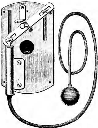
Fig. 115.—SEESAW SHUTTER.
