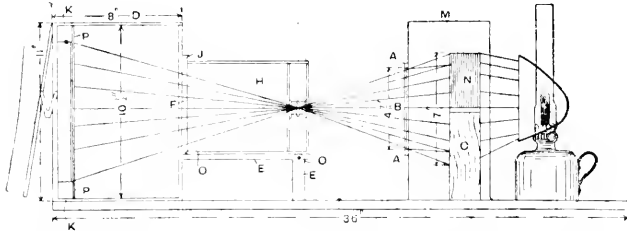
Fig. 447.—ENLARGING BY ARTIFICIAL LIGHT WITHOUT A LANTERN
