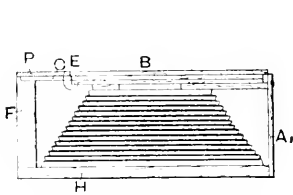
Fig. 70.—CAMERA CLOSED.
