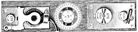
Fig. 116.—FOCAL PLANE SHUTTER (SIDE VIEW).
