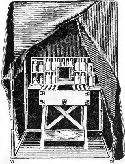
Fig. 355.—PORTABLE DARK-ROOM.
