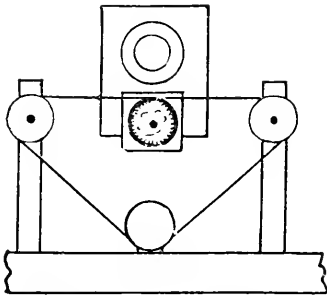
Fig. 733.—FOCUSsing DEVICE.
