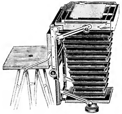
Fig. 113.—TILTING BOARD.
