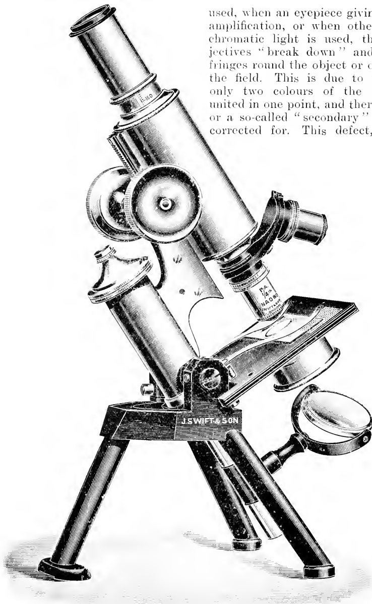
Fig. 691.—SWIFT'S STUDENT'S MICROSCOPE.
