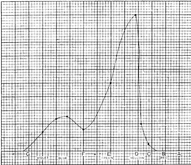
Fig. 593.—SPECTRUM CURVE ON ORTHOCROMATIC PLATE.
