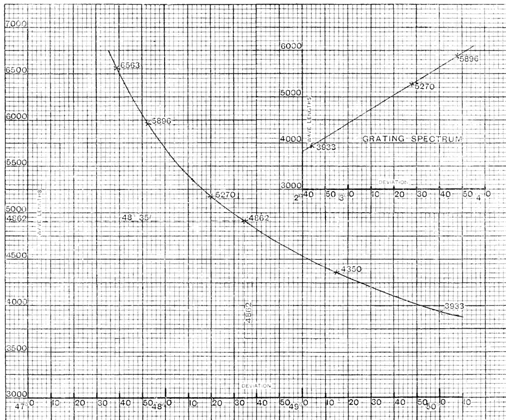
Fig. 763.—DEVIATION CURVES.
