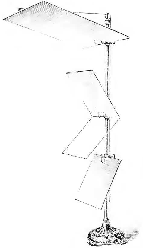
Fig. 605.—COMBINED HEAD-SCREEN AND REFLECTORS.
