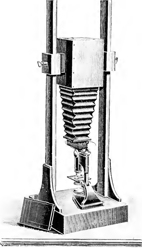
Fig. 732.—BECK'S VERTICAL CAMERA.
