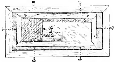
Fig. 838.—THE "UNIVERSAL" STEREOSCOPIC TRANSPOSER.
