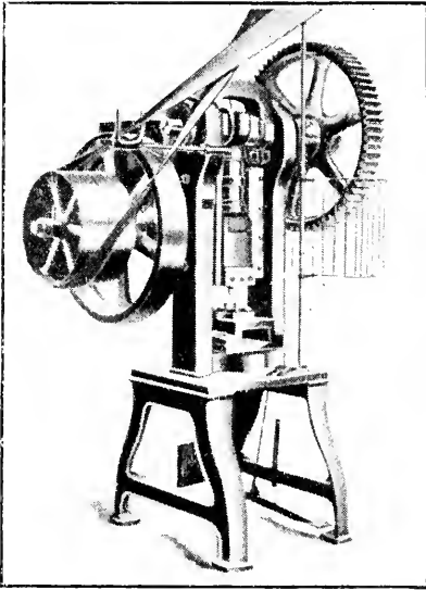
Fig. 542.—POWER PRESS.
