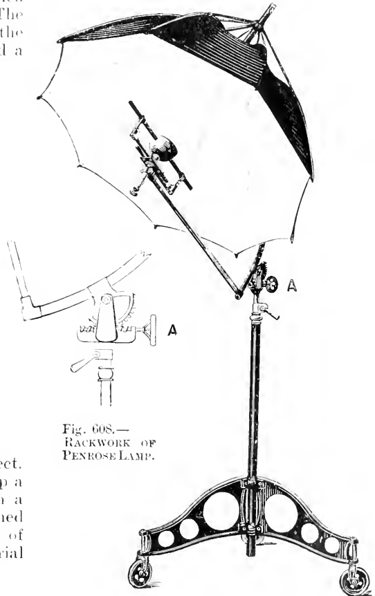
Fig. 607.—THE PENROSE STUDIO ARC LAMP.
