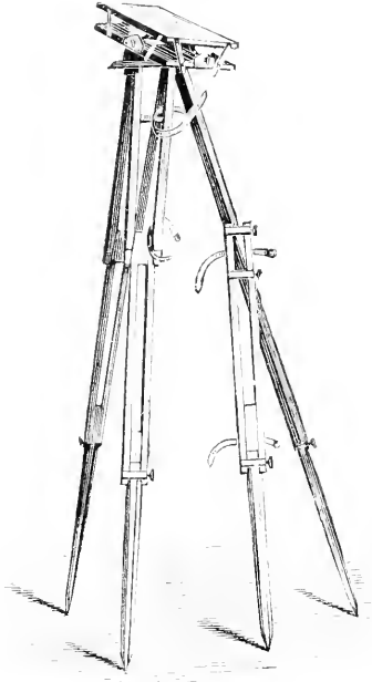
Fig 112.—STAND FOR ARCHITECTURAL WORK.
