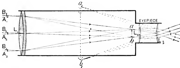
Fig. 797.—REFRACTING TELESCOPE.
