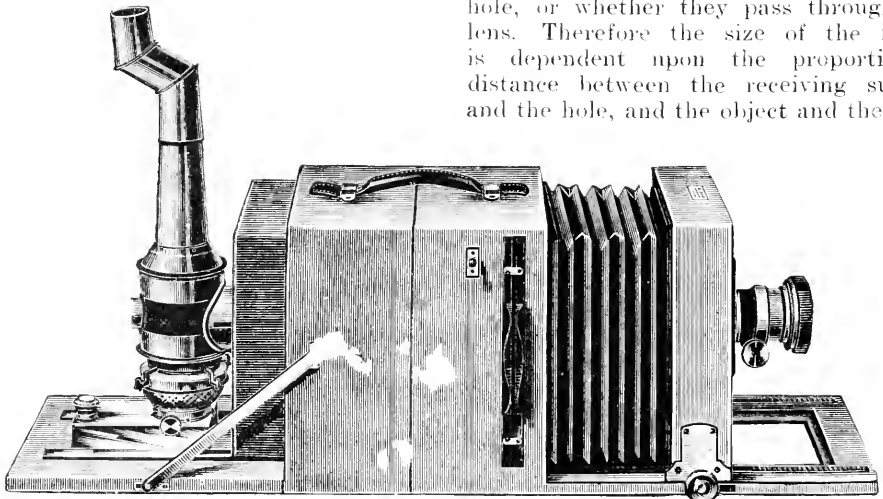
Fig. 434.—PORTABLE LANTERN FOR OIL.
