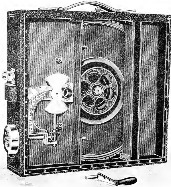
Fig. 881.—INTERIOR VIEW OF "KAMMATOGRAPH."
