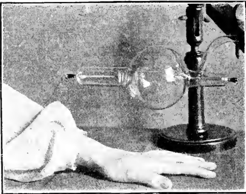
Fig. 918.—FOCUS TUBE.
