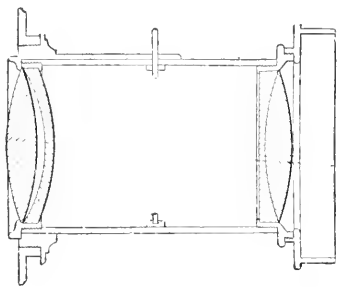
Fig. 43.—PETZVAL LENS IN SECTION.
