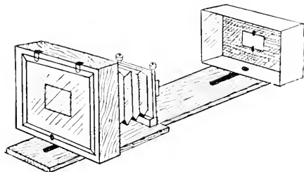
Fig. 456.—APPARATUS FOR MAKING SLIDES BY REDUCTION.
