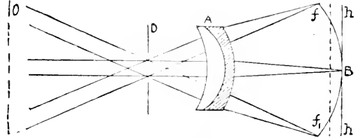
Fig. 491.—CURVATURE OF FIELD.
