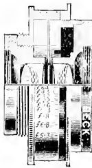
Fig. 521.—CINEMATOGRAPH LENS.
