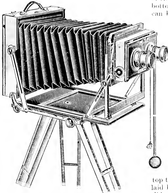
Fig. 74.—STEREOSCOPIC FIELD CAMERA, WITH ROLLER BLIND SHUTTER.
