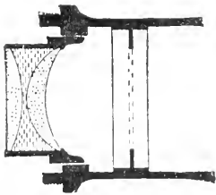
Fig. 517.—TELEPHOTO ATTACHMENT.
