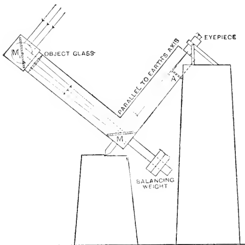
Fig. 805.—THE COUDÉ EQUATORIAL TELESCOPE.
