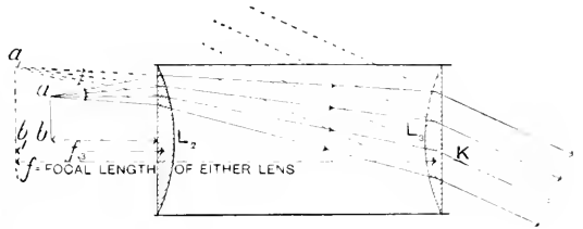
Fig. 798.—CALCULATING FOCAL LENGTH OF EYEPIECE.
