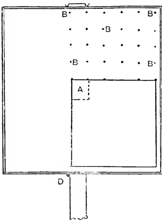
Fig. 320.—ARRANGEMENT FOR MULTIPLE PRINTING.
