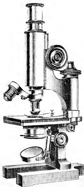
Fig. 690.—ROSS'S "STANDARD" MICROSCOPE.
