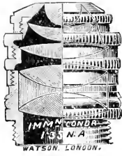
Fig. 709.—WATSON'S OIL IMMERSION CONDENSER.
