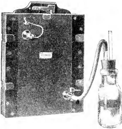
Fig. 567.—SPECIAL DARK-SLIDE FOR LIPPMANN PROCESS. (PENROSE.)
