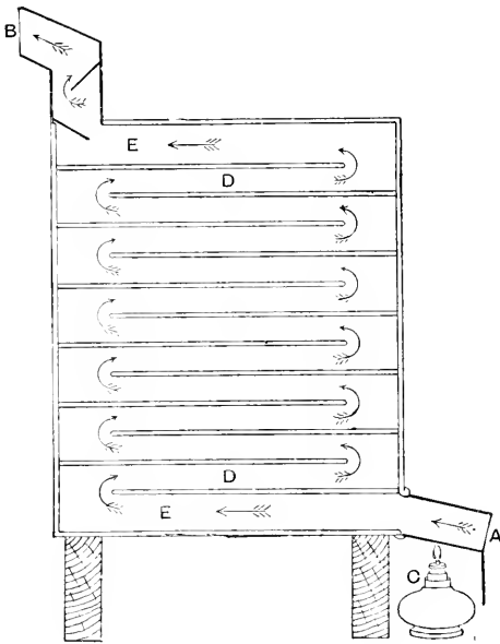
Fig. 299.—DRYING CUPBOARD.
