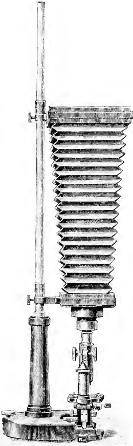
Fig. 729.—ZEISS'S VERTICAL CAMERA.
