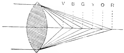
Fig. 486.—CHROMATIC ABERRATION.
