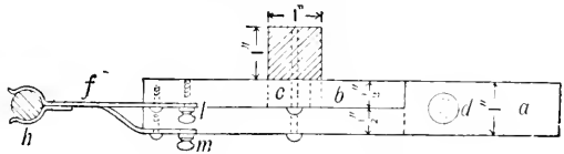
Fig. 789.—PLAN OF ARC LAMP.
