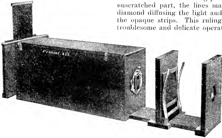
Fig. 773.—TALLET'S DIFFRACTION GRATING SPECTROSCOPIC CAMERA.
