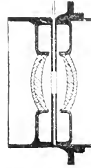
Fig. 506.—SECTION OF WIDE-ANGLE RECTILINEAR LENS
