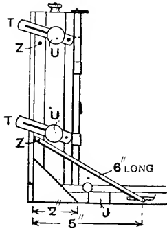
Fig. 85.—STEREOSCOPIC CAMERA WITH FRAMES CLOSED.
