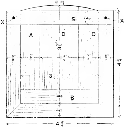
Fig. 91.—DARKSLIDE AND RAILS.
