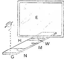
Fig. 630.—MONOCHROME VIEW METER IN USE.
