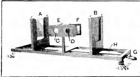
Fig. 811.—THE WHEATSTONE STEREOSCOPE.
