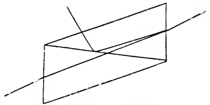
Fig. 718.—ACTION OF NICOL'S PRISM.
