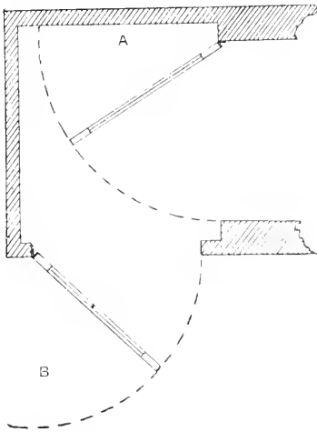
Fig. 361.—DOUBLE LIGHT-TRAP DOOR.
