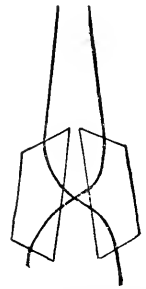
Fig. 741.—PATH OF RAYS THROUGH BINOCULAR PRISMS.
