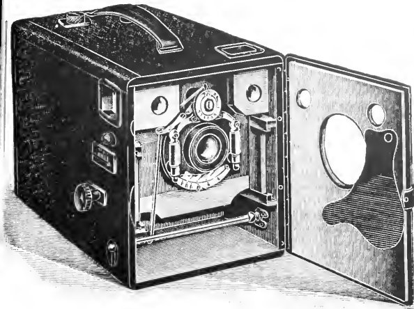
Fig. 30.—MAGAZINE HAND CAMERA.
