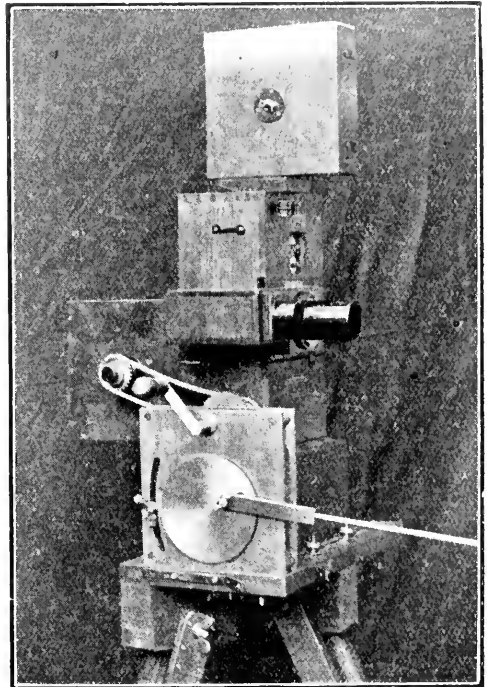
Fig. 854.—CINEMATOGRAPH CAMERA AND MECHANISM FOR OSCILLATING SUBJECT.
