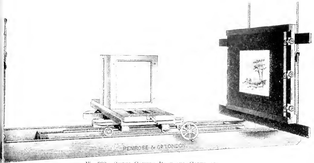
Fig. 900.—SWING CAMERA BASE AND COPYBOARD.
