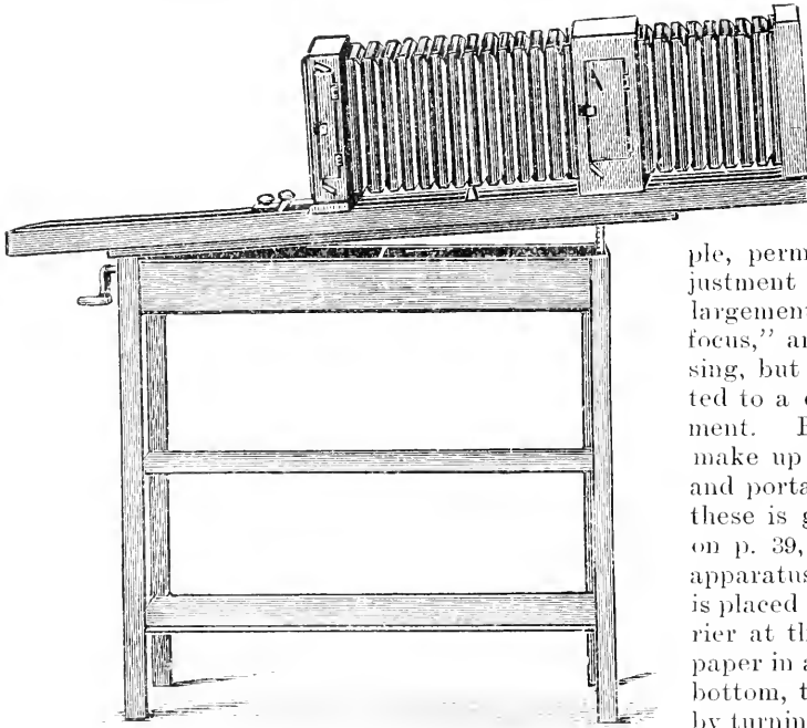
Fig. 66.—ENLARGING CAMERA AND STAND.
