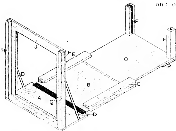
Fig. 68.—ENLARGING CAMERA WITH BELLOWS AND FRONT REMOVED.
