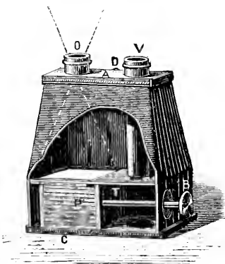
Fig. 661.—BINOCULAR HAND CAMERA.
