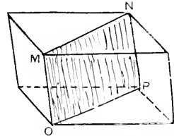
Fig. 716.—NICOL'S PRISM.
