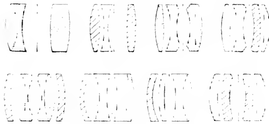
Fig. 509 —UN-SYMMETRICAL ANASTIGMATS.
