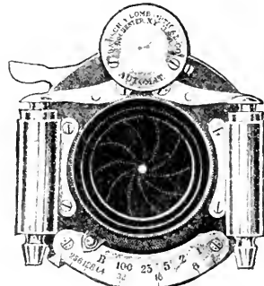
Fig. 118.—A TYPICAL EVERSET AUTOMATIC SHUTTER.
