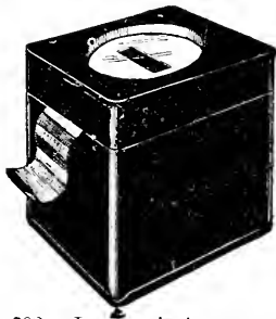
Fig. 292.—JOHNSON'S ACTINOMETER.
