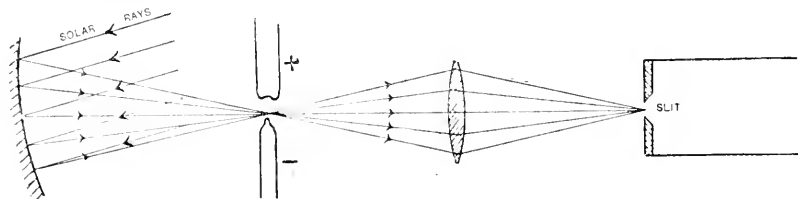
Fig. 768.—PROJECTION OF SOLAR RAYS ON COLLIMATOR SLIT.
