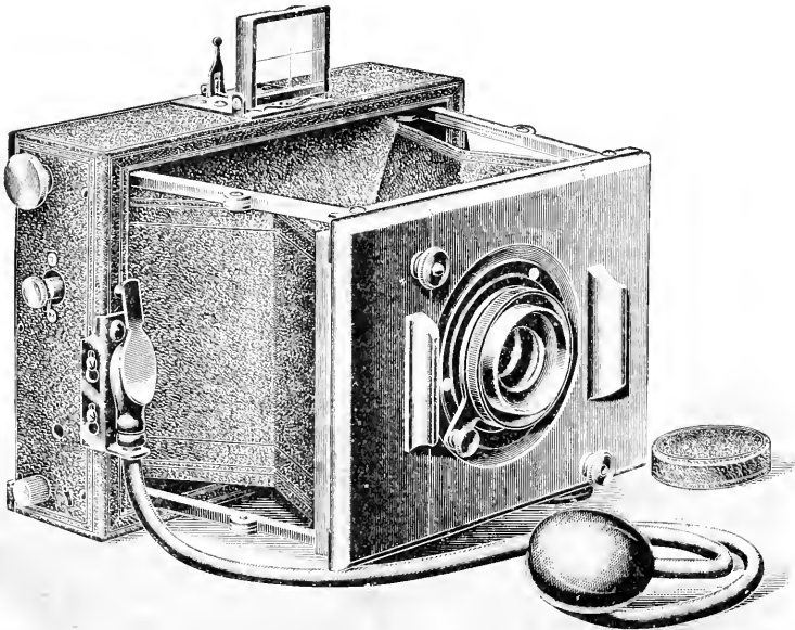
Fig. 665.—VOIGTLÄNDER'S "FAVOURITE" HAND CAMERA.
