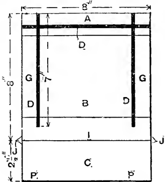
Fig. 78.—BASEBOARD FOR STEREOSCOPIC CAMERA.
