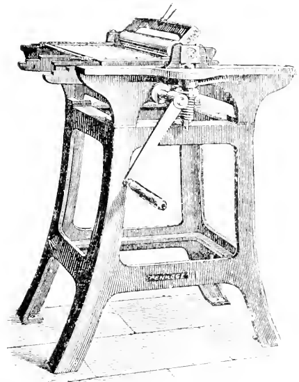
Fig. 888.—COLLOTYPE PRESS, WORKING WITH ROLLER AND ECCENTRIC.
