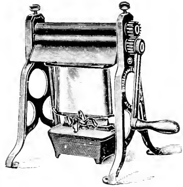
Fig. 411.—ROLLER BURNISHER FOR PARAFFIN.
