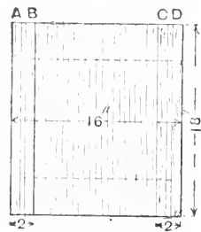
Fig. 52.—BASEBOARD.
