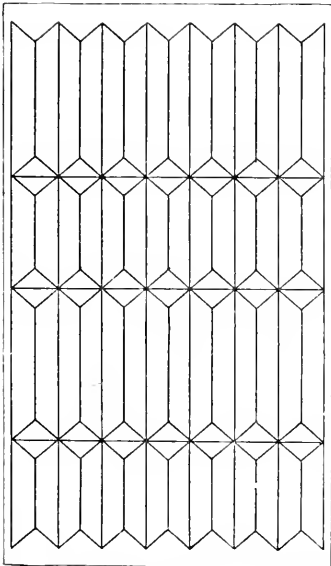
Fig. 929.—CARDBOARD STRIPS FOR SQUARE BELLOW.
