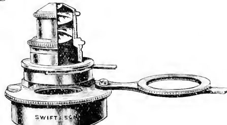
Fig. 706.—SWIFT'S "PAN-APLANATIC" CONDENSER.
