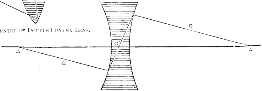
Fig. 494.—OPTICAL CENTRE OF DOUBLE CONCAVE LENS.
