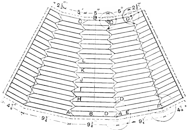
Fig. 930.—PATTERN FOR CONICAL BELLOW.
