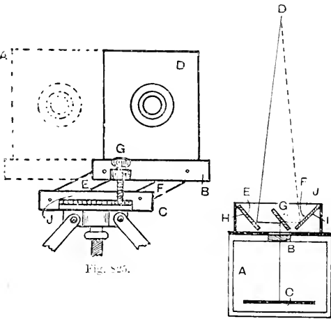
Fig. 825.—ADAPTER WITH ADJUSTABLE SEPARATION. Fig. 826.—THEODORE BROWN'S REFLECTING ADAPTER.
