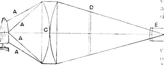
Fig. 435. - OPTICAL CONSTRUCTION OF ENLARGING LANTERN.
