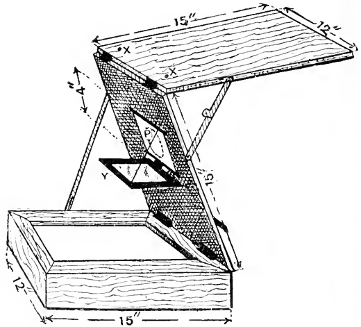
Fig. 227.—RETOUCHING DESK.
