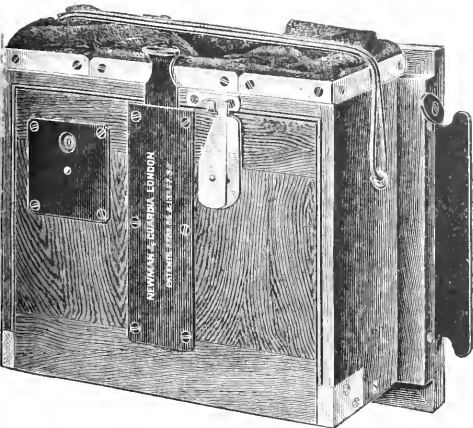
Fig. 37.—CHANGING BOX.
