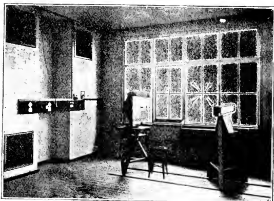
Fig. 552.—TRAMWAY CAMERA.
