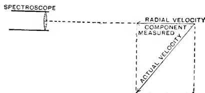
Fig. 810.—DOPPLER'S PRINCIPLE APPLIED TO MEASUREMENT OF VELOCITY.
