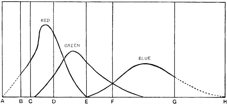
Fig. 568.—CLERK-MAXWELL COLOUR SENSATION CURVES.
