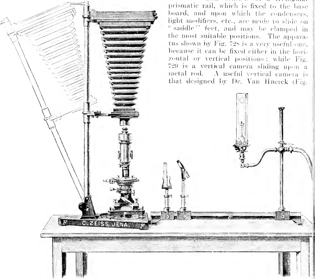
Fig. 728.—ZEISS'S VERTICAL AND HORIZONTAL CAMERA, ETC.
