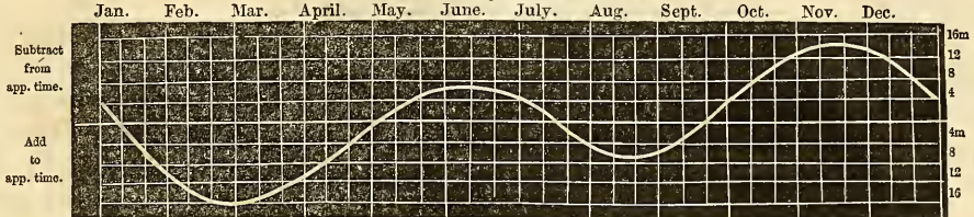
CURVE OF THE EQUATION OF TIME.
