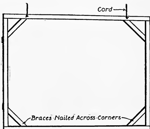
FIG. 328. — Frames for Drops.
