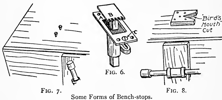
Some Forms of Bench-stops.
