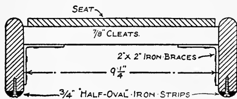
FIG. 316. — A Section through the Sled.
