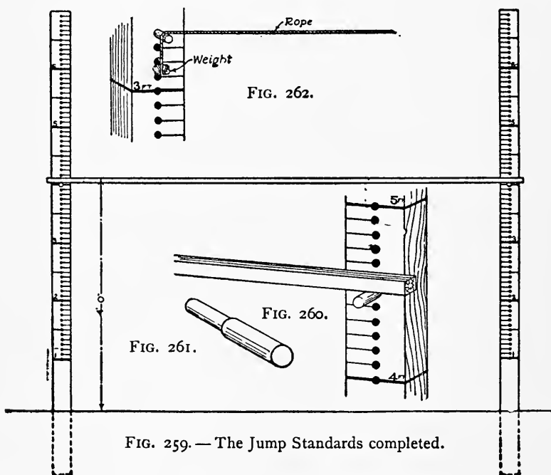
FIGS. 259-262. — Details of Jump Standards.
