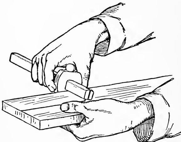
FIG. 41.— Using the Marking-gauge.
