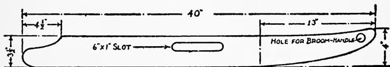
FIG. 315. — Pattern for Runners.
