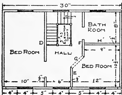
FIG. 99. SECOND FLOOR PLAN
