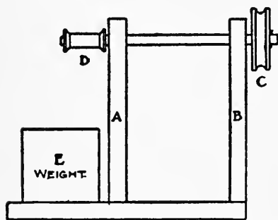
FIG. 356.—Support for Trolley-line.
