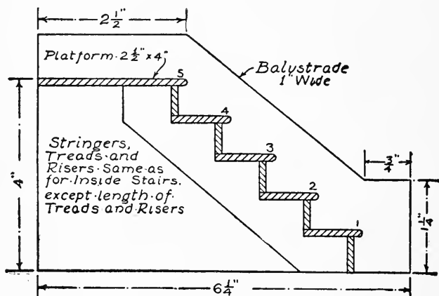
FIG. 76.—The Front Steps.
