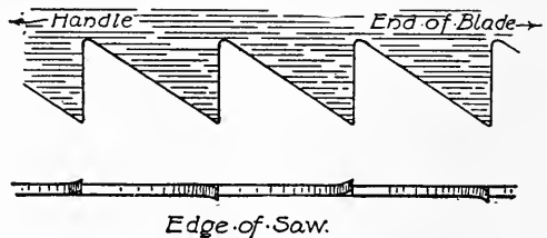
FIG. 20. — Teeth of Rip Saw.
