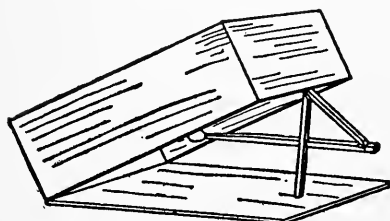
FIG. 216.—The Figure-four Trap set.
