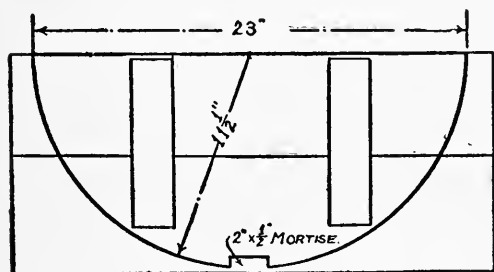
FIG. 204.—The Mould.
