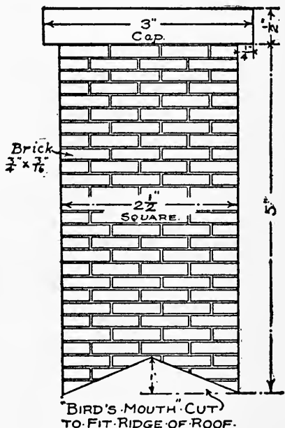
FIG. 92. — Construction of Chimneys.
