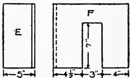
FIG. 102. SECOND FLOOR PARTITIONS
