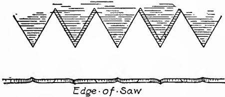
FIG. 19. — Teeth of Cross-cut Saw.
