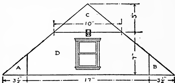
FIG. 116. — Front Gable-end.
