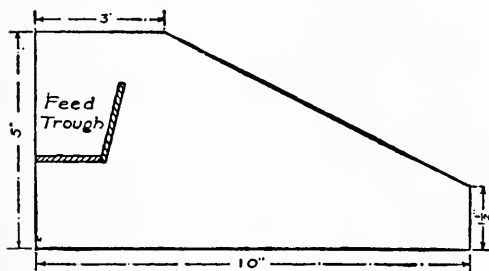
FIG. 117. — Stall Partitions.
