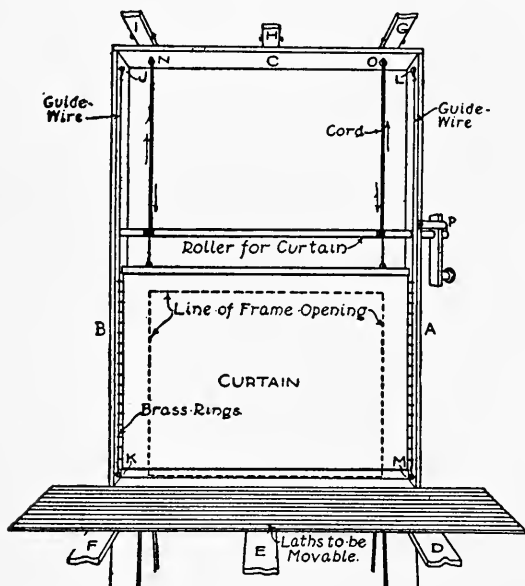
FIG. 318. — View of Curtain from Stage.
