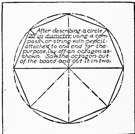
FIG. 77. — Make Gable-ends like This.
