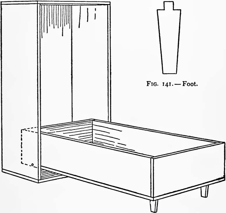
FIG. 140.—Folding-bed (open).
