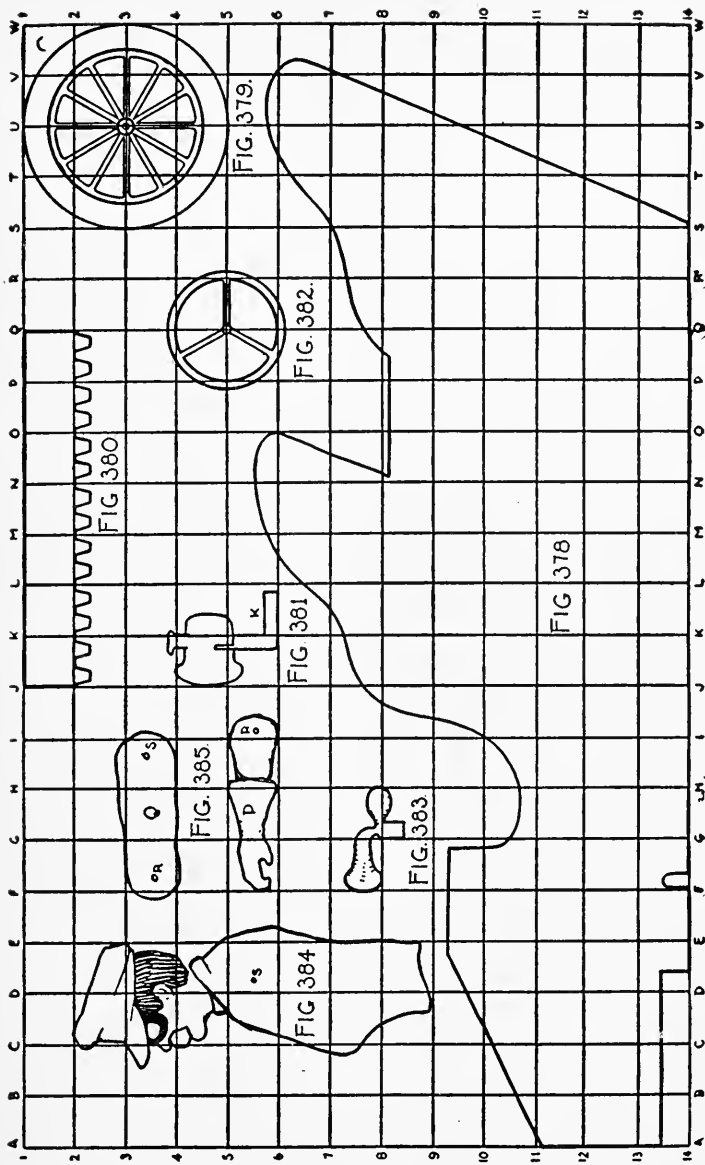
Figs. 378-385. — Patterns for the Automobile Touring-car.
