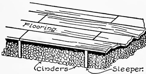
FIG. 186. — Construction of Floor.
