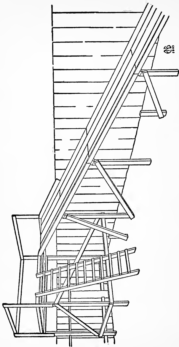
FIG. 310. — A Back-yard Toboggan-slide.
