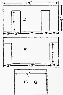
FIG. 69. PARTITIONS FOR SECOND FLOOR.
