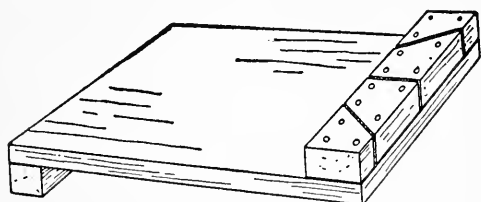
FIG. 11. — A Bench-hook.
