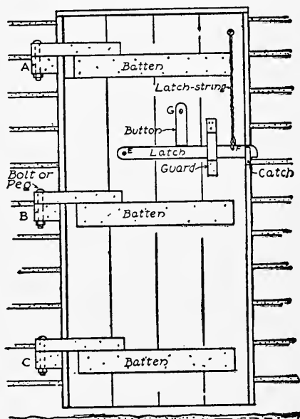
FIG. 194. — The Cabin Door.
