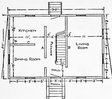
FIG. 65. FIRST FLOOR PLAN
