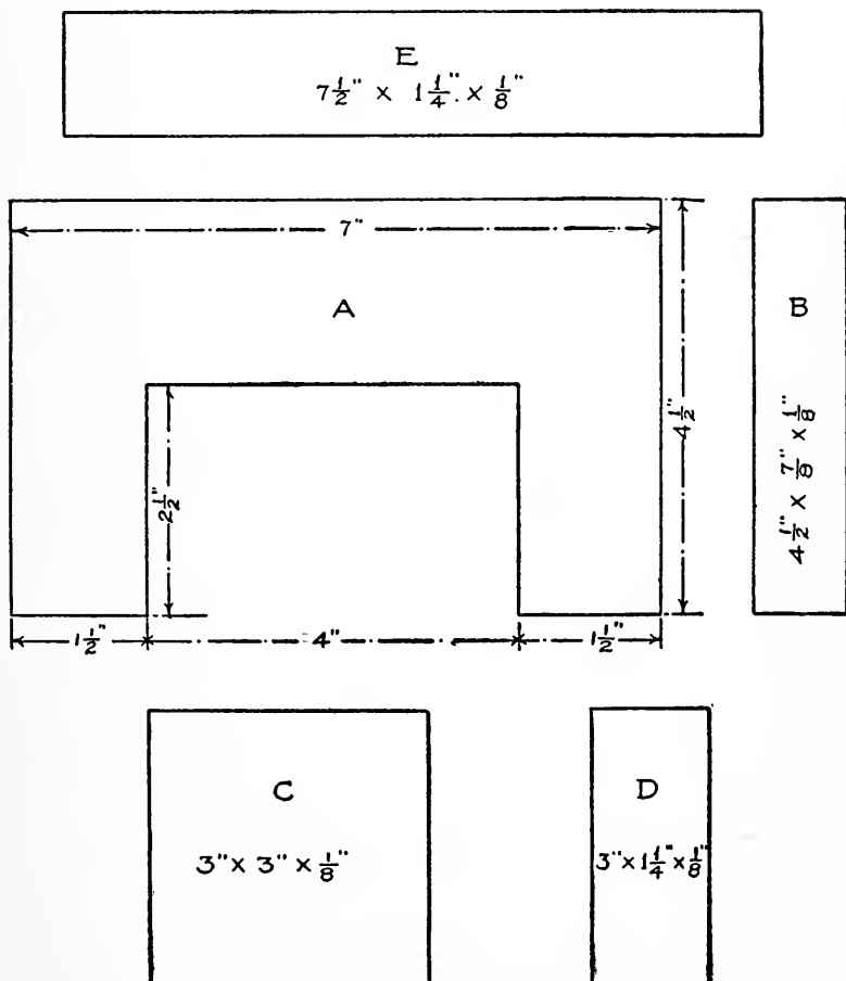
FIG. 94. — Construction of Mantel.
