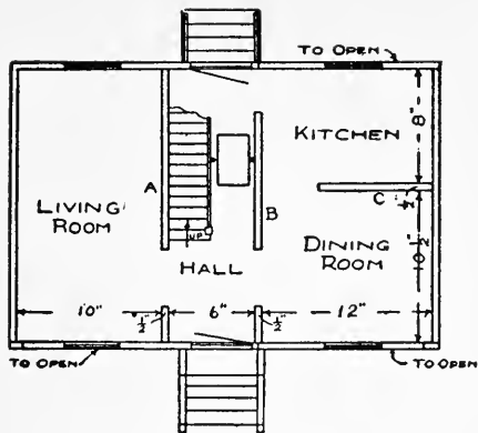
FIG 98 FIRST FLOOR PLAN
