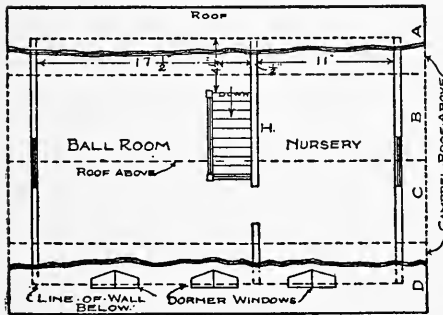
FIG. 67. THIRD FLOOR PLAN
