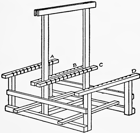
FIG. 173. — A Washing-rack.
