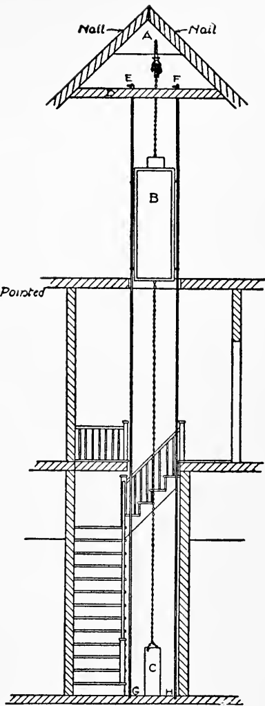
FIG. 104. — Front View of Elevator-shaft and Stairs.
