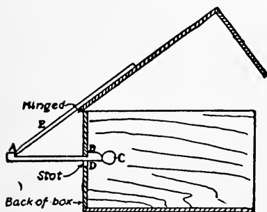
FIG. 218. — Cross Section of Trap.
