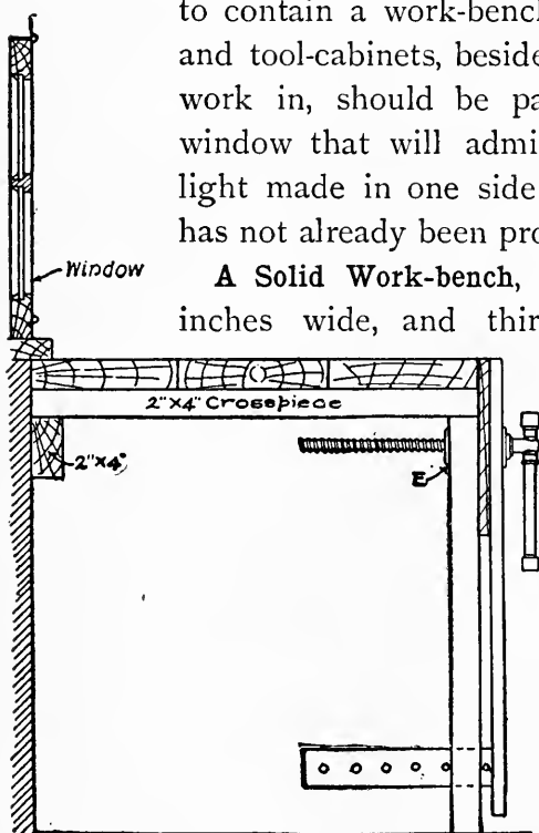
FIG. 1. — End View of Work-bench.
