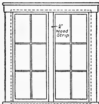
FIG.88 CASEMENT WINDOWS
