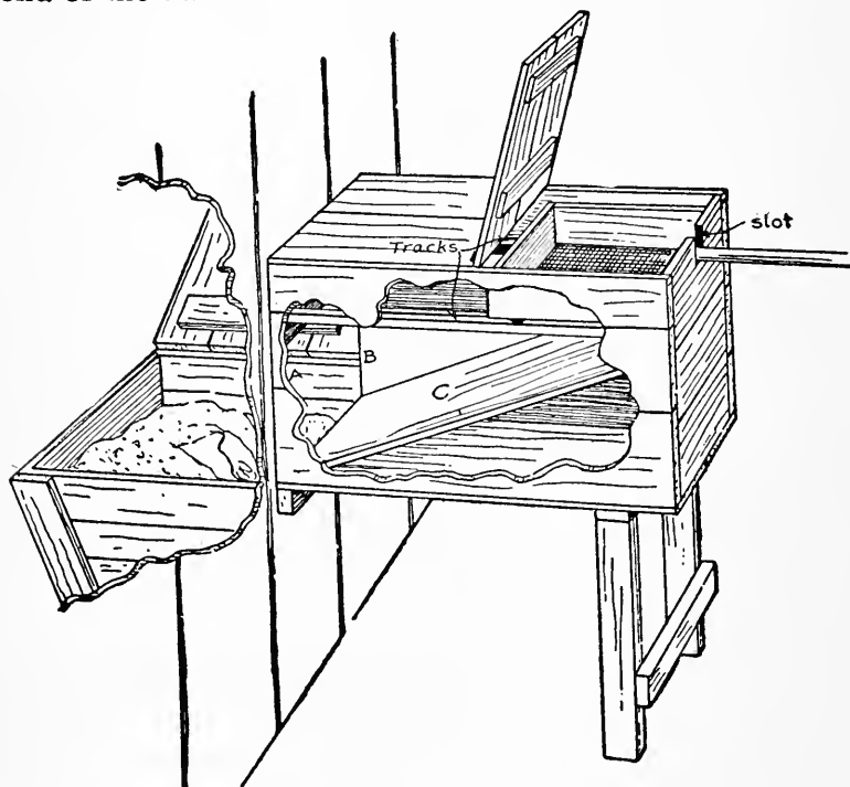
FIG. 48. — An Ash-sifter.
