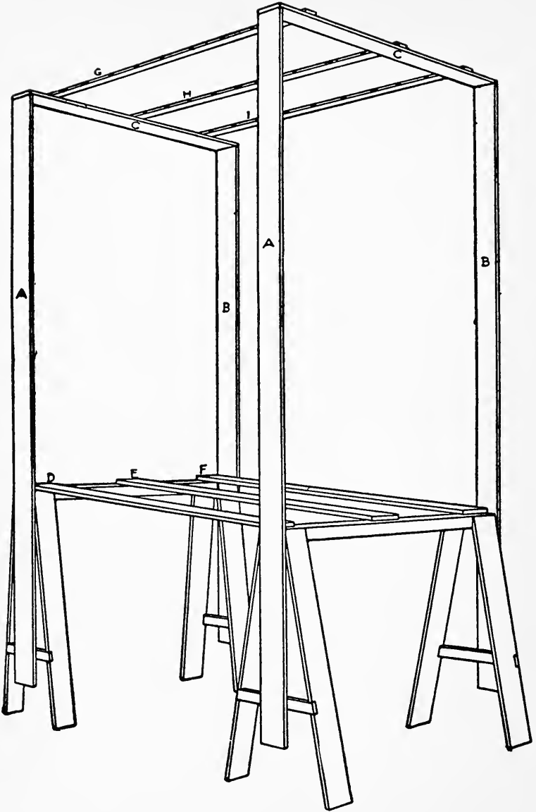
FIG. 317. — The Stage Framework.
