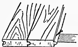
FIG. 32. — Blind-nailing.
