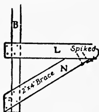
FIG. 255. — Corner Bracing.
