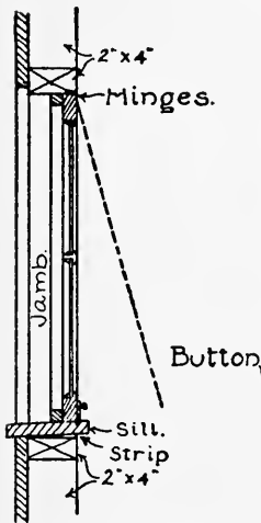
FIG. 188. — Section through Window.
