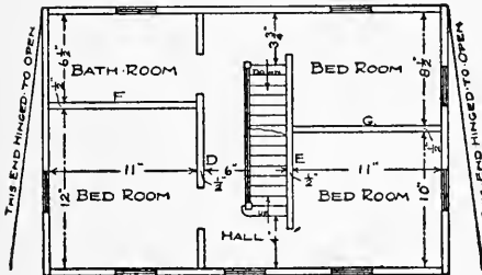
FIG. 66. SECOND FLOOR PLAN
