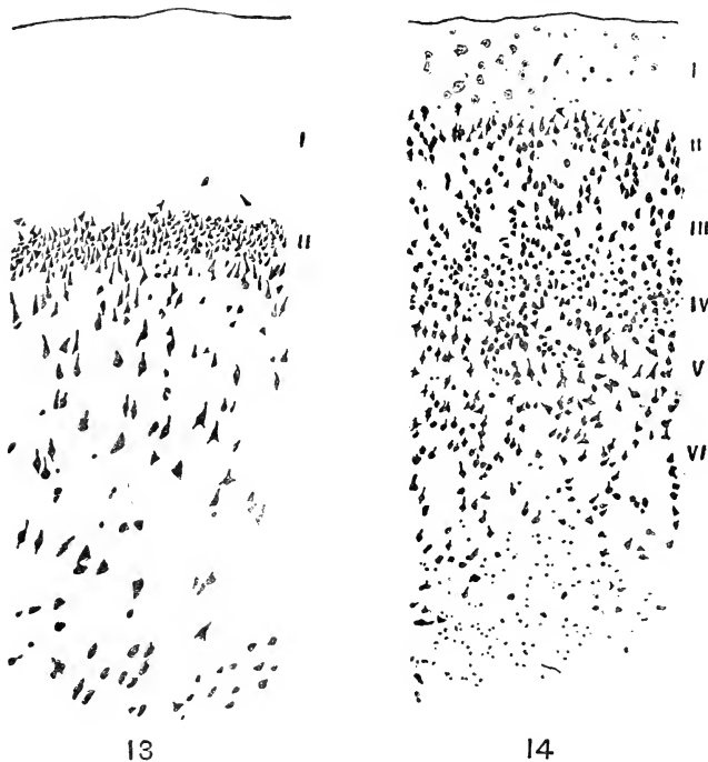
FIG. 13.—Archipallial cerebral cortex of the opossum from the middle of the pyriform lobe ( a. pir. med. of Fig. 36, p. 154). From an unpublished drawing kindly furnished by Dr. P. A. Gray. Magnification, 50 diameters.
