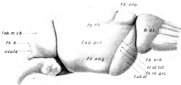
FIG. 32.—Lateral view of the brain of Orolestes inca , enlarged about four times. After Obenchain (1925). The olfactory bulb ( b. ol. ) is very large. The small cerebellum shows a large lobus medius ( lob. m. cb. ) bounded behind by the fissura secunda ( fs. s. ). The cerebral cortex shows two fissures. The orbital fissure ( fs. orb. ) cuts across the excitable motor field, and the rhinic fissure ( fs. rh. ) separates the neopallium above from the pyriform lobe ( lob. pir. ) below. The latter is separated from the amygdala by a shallow amygdaloid fissure ( fs. amg. ). The olfactory tubercle ( tub. ol. ) is a subcortical reflex center, separated from the cortex by the large lateral olfactory tract ( tr. ol. lat. ), which in turn is bounded above by the fissura endorhinalis ( fs. erh. ) and below by the fissura rhinalis arcuata ( fs. rh. arc. ).
