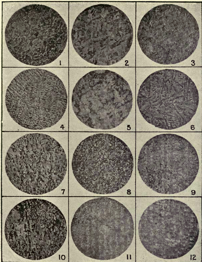
THE MICROSTRUCTURE OF BEARING METALS.
