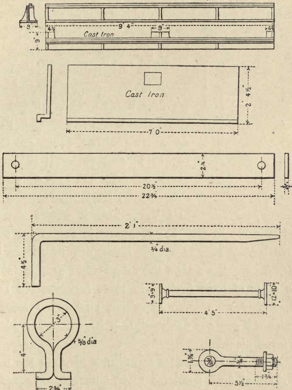
Fig. 5.—DETAILS.
