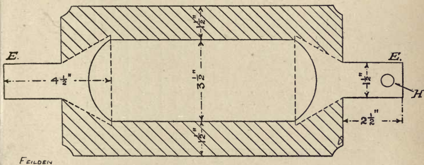
Fig. 10—TOP VIEW.
