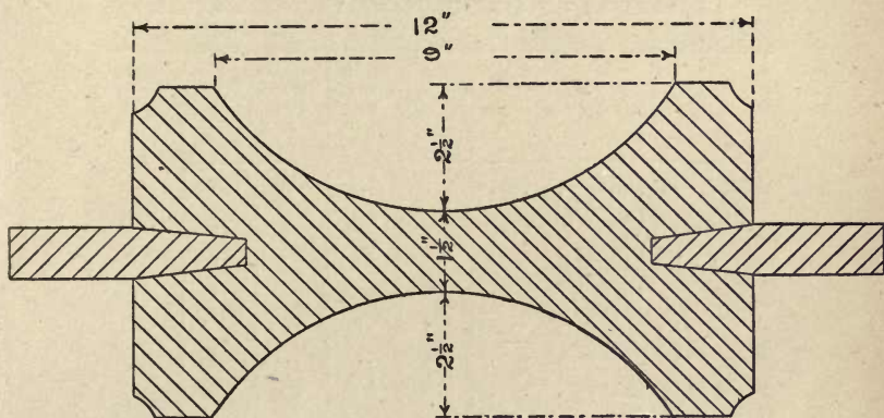
Fig. 9—SECTION OF INGOT-MOULD.
