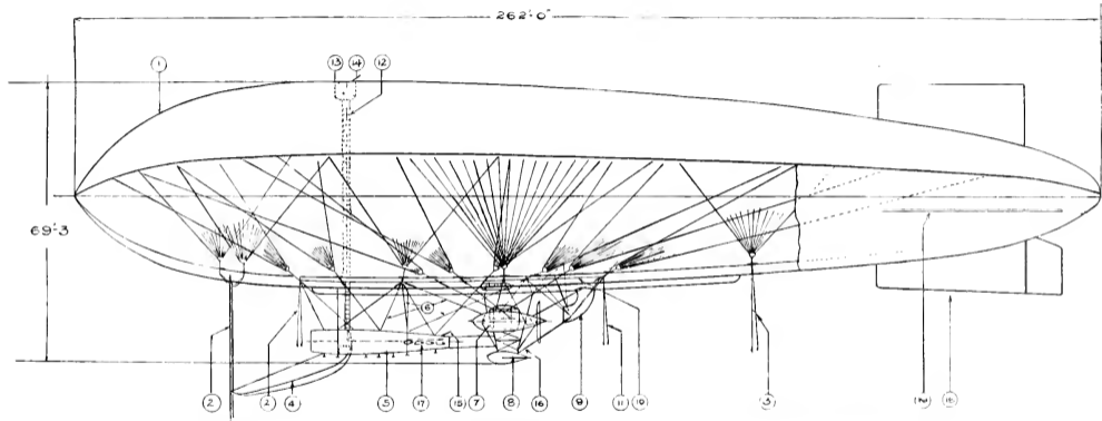
SECTIONAL ELEVATION OF SOUTH SEA AIRSHIP
