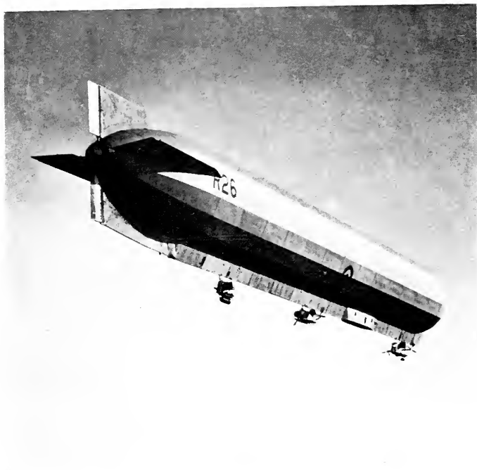
RIGID AIRSHIP NO. 26 (23 CLASS)
