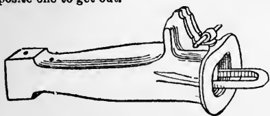
DEITZ FREIGHT DRAWBAR.
