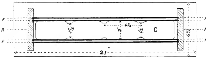
Upper Side of Bottom of Super.
