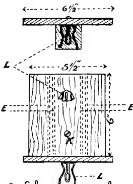
End Elevation of Super.
