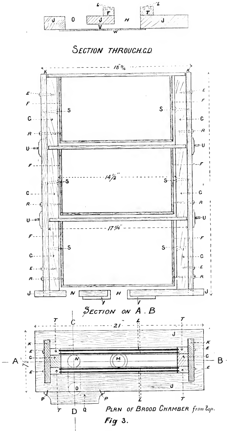
A.B., Longitudinal Section; C.D., Cross Section; E., Glass Frame Screws; F., Frame; G., Blocks; H., Entrance Hole; I., Turntable (upper half); J., Bottom; K., End Upright; L., Glass; M., Entrance Hole; N., Entrance Hole to Feeder; O., Feed Hole; P., Bracket Screws; Q., Bracket for Feeder; R., Frame Screws; S., Block Screws; T., Frame for Glass; U., Ventilators; V., Passage to Feeder; W., Perforated Zinc Bottom to Passage.
