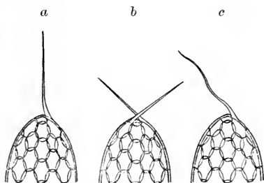
FIG. 115.—Types of spines of Euglypha cristata var. acicularis . × 450.
