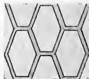
FIG. 127.—Hexagonal appearance occasionally seen in tests of Euglypha compressa . \times 1000 .
