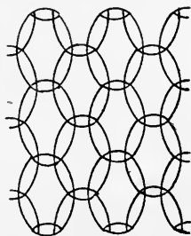
FIGS. 112–114.— Euglypha tuberculata . 112, circular type of body-scales. \times 1000 . 113, oval type. \times 1000 . 114, aperture-scale \times 2000 .
