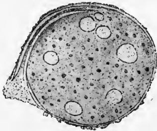
FIG. 156.— Lieberkuehnia wageneri , without its pseudopodia. \times about 250. (After Penard, as L. fluvialis .)
