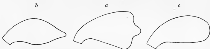
FIG. 148.—Outlines of tests of Cyphoderia trochus and two varieties. \times 240 . a, C. trochus (type); b, var. palustris ; c, var. amphoralis .
