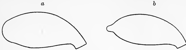
FIG. 144.—Outlines of tests of Cyphoderia ampulla var. vitrea . \times 260 . a, normal form. b, with papillose fundus.
