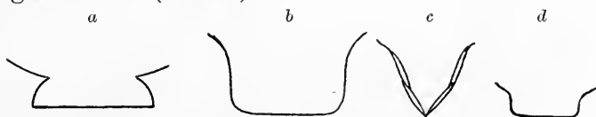
FIG. 133.—Types of apertures of Sphenoderia lenta . \times 1000 . a . Length of test 48\mu : Pilmoor. b . Length of test 42\mu : New Forest. c . Narrow view of same. d . Length of test 32\mu : Isle of Wight.
