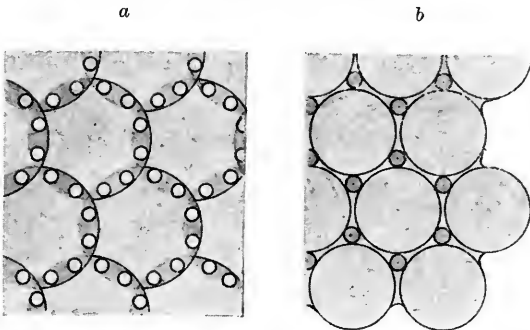
FIG. 147.—Portions of test of Cyphoderia ampulla var. major . \times 4000 . a , from Port Erin, Isle of Man; b , another specimen from same locality showing line of a fracture.
