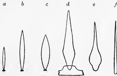
FIG. 129.—Various types of spines of Placocista spinosa . a-c , \times 800 ; d-f , \times 1040 (after Penard); f , side view.
