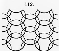
FIGS. 112–114.— Euglypha tuberculata . 112, circular type of body-scales. \times 1000 . 113, oval type. \times 1000 . 114, aperture-scale \times 2000 .
