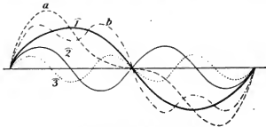
Fig. 6 I. a = \bar{1} + \bar{2} , b = \bar{1} + \bar{3} .
