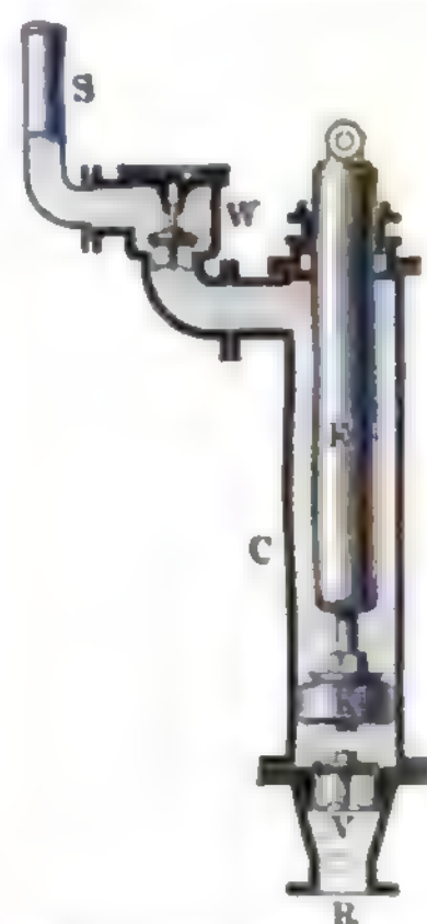
Fig. 7. Differentialpumpe.
