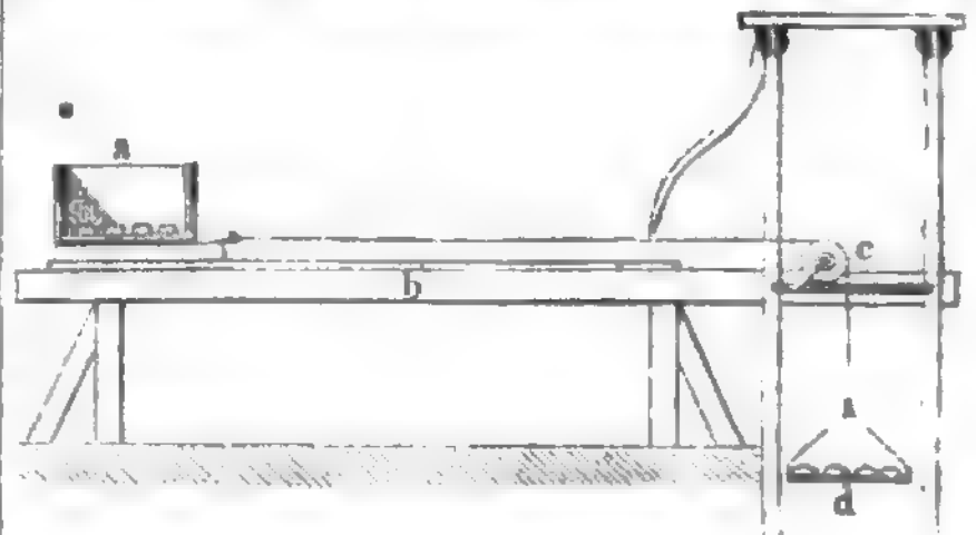
Coulombs Tribometer.
