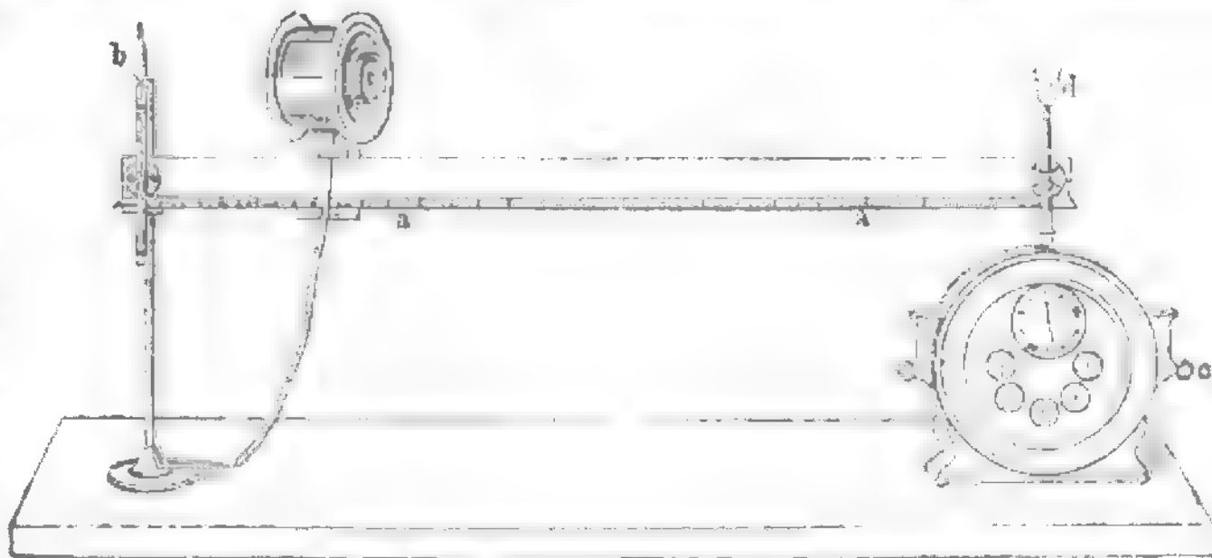
Fig. 3. Bunsens Photometer.
