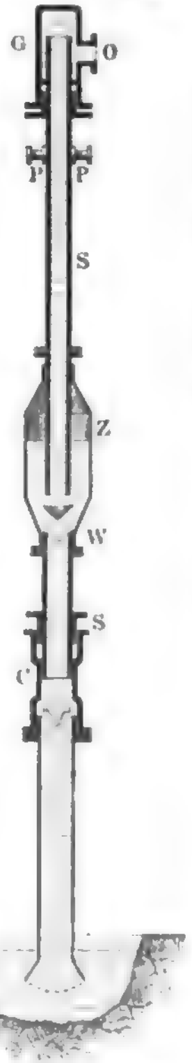
Fig. 8. Rittinger-Schachtpumpe.
