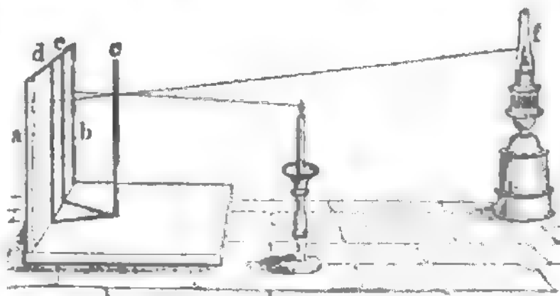
Fig. 1. Rumfords Photometer.
