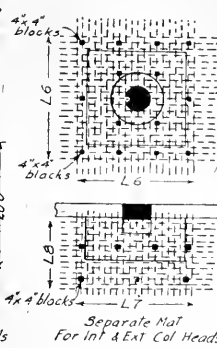
Details of flat slab reinforcement featuring short bars without bends
