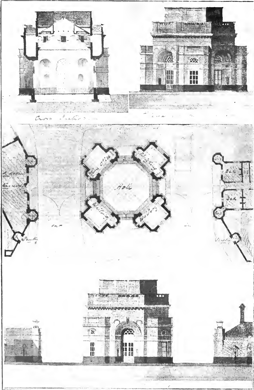
ENTRANCE BUILDING, LARGE MUNITION FACTORY, BIRMINGHAM. Messrs. B. LAND, HAYWOOD and FARMER, F.F.R.I.B.A., Architects.
