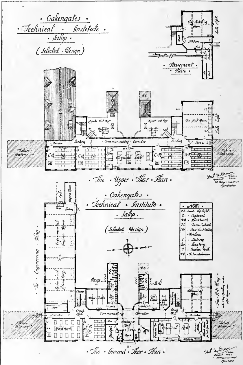
OAKENGATES TECHNICAL INSTITUTE, SHROPSHIRE. Mr. HERBERT H. BROWN, F.R.I.B.A., Architect.
