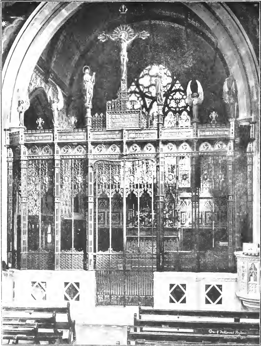
BRONZE AND WROUGHT IRON ROD SCREEN, CHRIST CHURCH, EPSOM. MR. G. H. FELLOWES-PYRENE, F.R.I.B.A., ARCHITECT.
