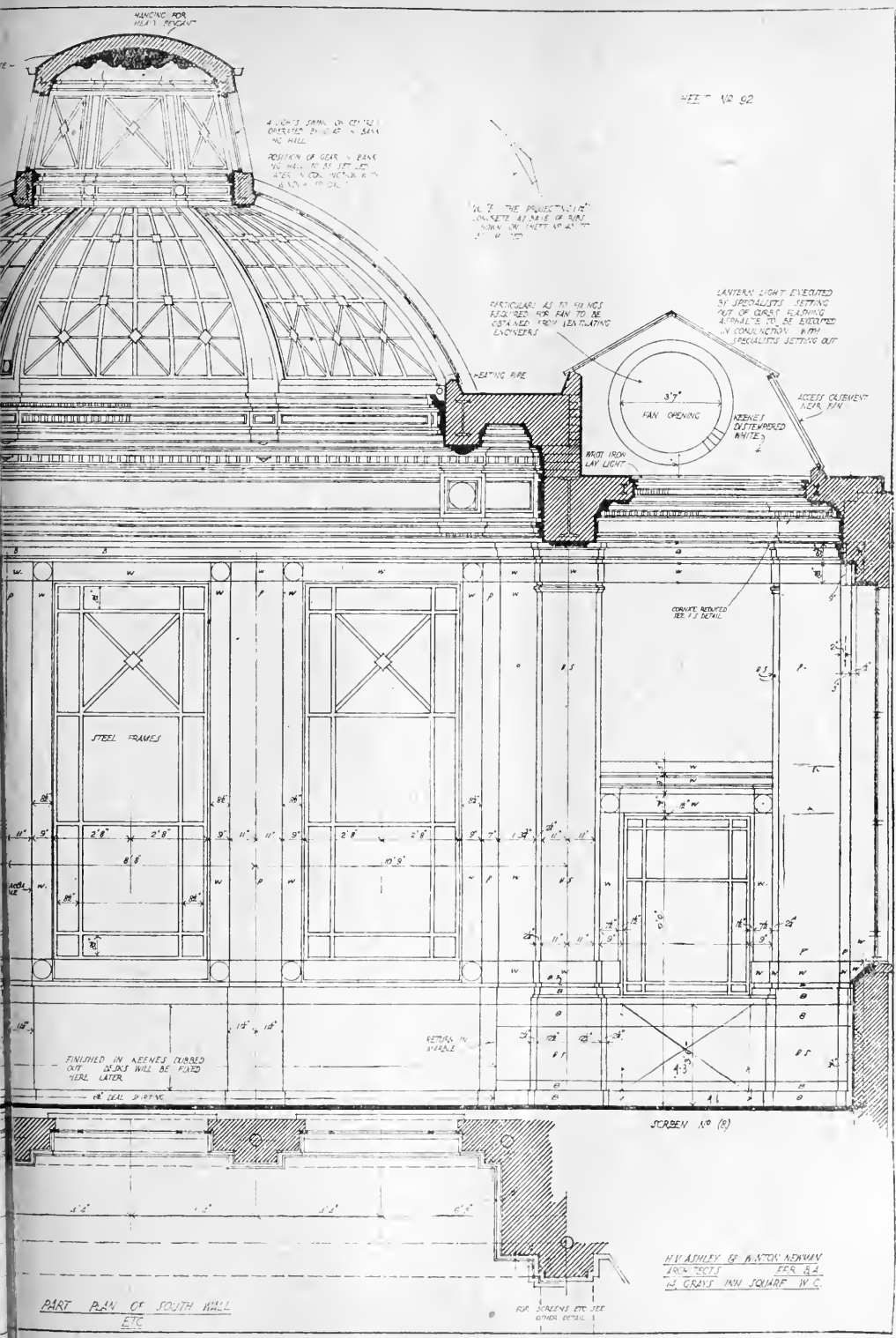
WING SECTION.—Messrs. H. V. ASHLEY and WINTON NEWMAN, F.F.R.I.B.A., Architects.
