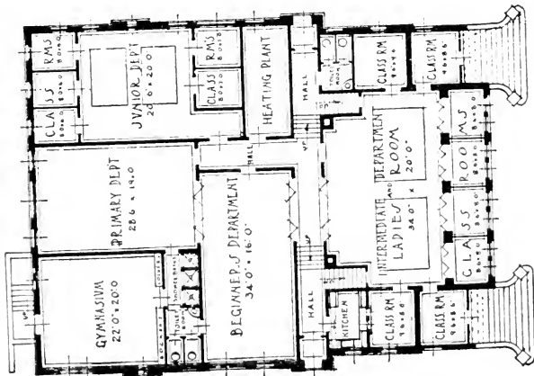
MAIN FLOOR
