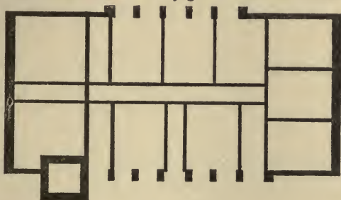
Foundation Plans
