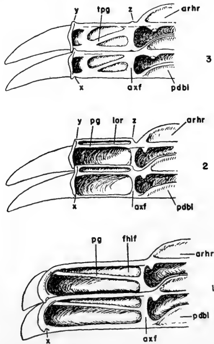
Figure 3. Idealized sketch of the thoracic articulation devices of (1) Tesselacauda depressa , n. gen. and sp., (2) Protopliomerops superciliosa , n. sp., and (3) Ceraurus pleurexanthus , the last after Størmer. All greatly magnified and showing the ventral side of the right half of each segment.
