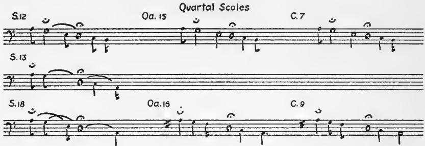
FIGURE 23.—Quartal scales.
