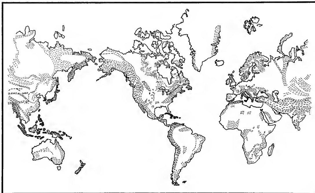
Structural trends of the rocks in orogenic belts. Blank areas include those where there is insufficient data and also where flat lying strata cover the deformed rocks of the crust, such as in Illinois. Greenland is nearly all under ice. The shaded areas are the young mountain ranges formed within the last 100 million years, mainly during the latter half of this period.
