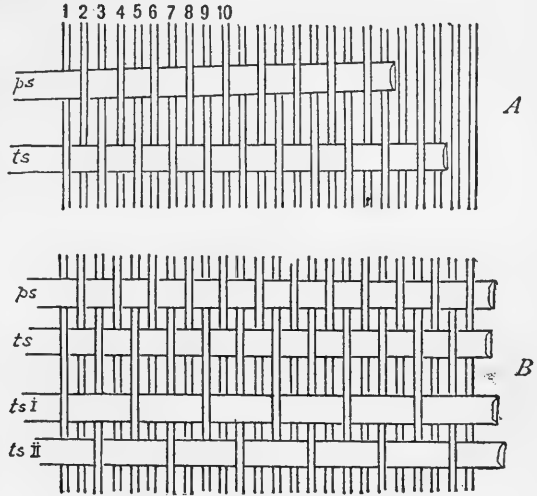
FIGURE 61.—Manufacture of a 6-weft Atorai hammock. (Sec. 473 A.) A , The first two wooden slips ( ps , ts ) picking up strings 2, 4, 6, 8, 10, etc., and 1, 3, 5, 7, 9, etc., respectively. B , The second two wooden slips ( ts I , ts II ) picking up strings 1, 5, 9, 13, 17, etc., and 3, 7, 11, 15, 19, etc., respectively
