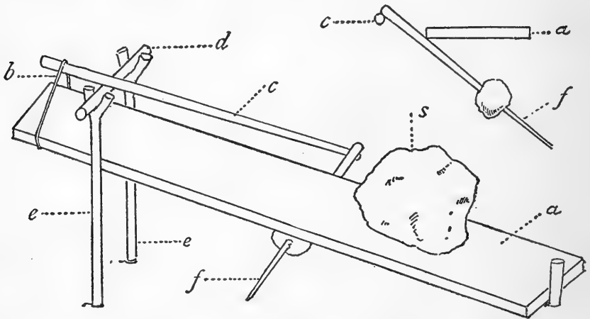
FIGURE 8.—Fall-trap for labba, etc., on the Demerara River. (Sec. 161.) a , Heavy plank, weighted with a stone; b , loop; c , catch stick; d , crossbar; ee , vertical forks; f , bait stick
