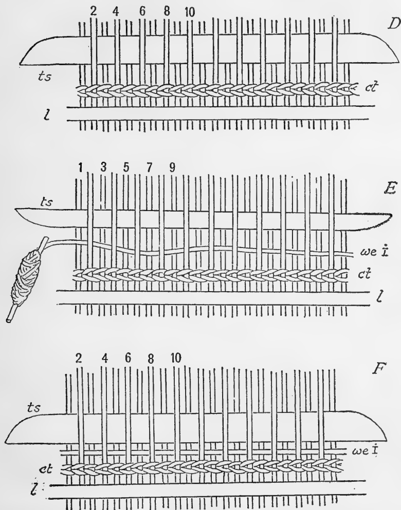
FIGURE 63.—Manufacture of a 6-weft Aorai hammock, continued (sec. 473 A), showing how the first weft ( we i ) is placed and fixed in position
