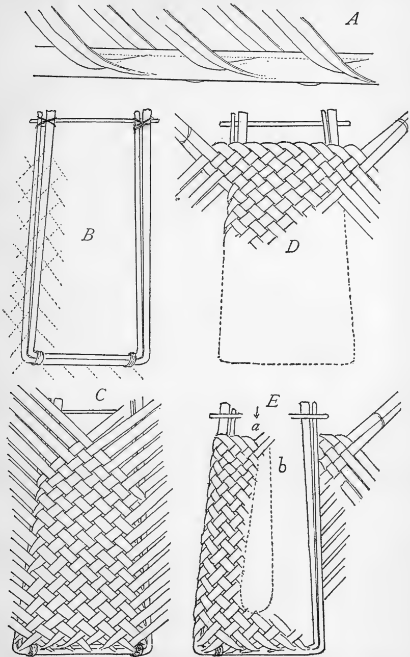
FIGURE 59.—Manufacture of the Waiwai temporary pimpler-palm shoulder basket. (Sec. 456 B)
