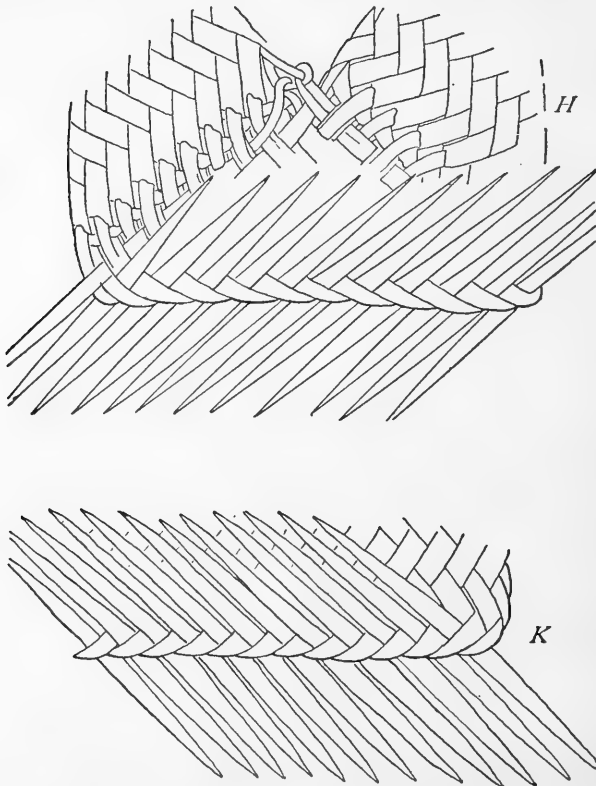
FIGURE 49.—Manufacture of the ite-leaf close-work knapsack, continued. (Sec. 455 C.) H , Starting at the base of the triangle from left to right break the upper layer of projecting strands one-under-one. K , View of the lower portion of the back of the article
