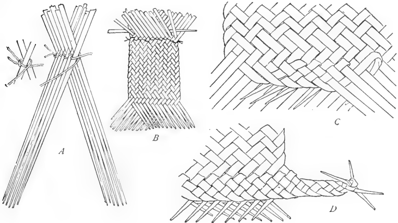
b, Diagram explaining manufacture of the pimpler-palm knapsack cover. (Sec. 452)
