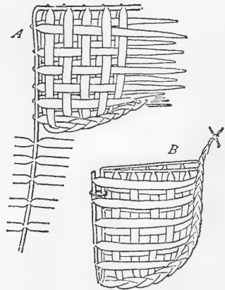
FIGURE 57.—Temporary bush basket, No. 1. (Sec. 456 A)
