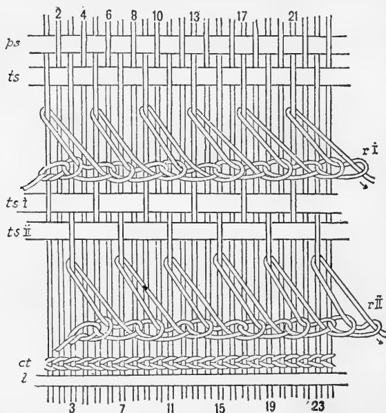
FIGURE 62.—Manufacture of a 6-weft Atoral hammock, continued (sec. 473 A), showing insertion of the level ( l ) and the commencing chain twist ( ct ). In actual practice the lower three slips ( ts , ts I, ts II) are, however, previously removed
