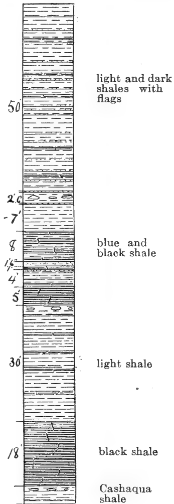
FIG. 2 Section in Buck run ravine at Mt. Morris, above Cashaqua shale. Stations 4, 5
