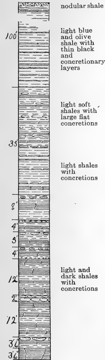
FIG. 10 Section on Big Sister creek from Evans Center to Pontiac. Station 52
