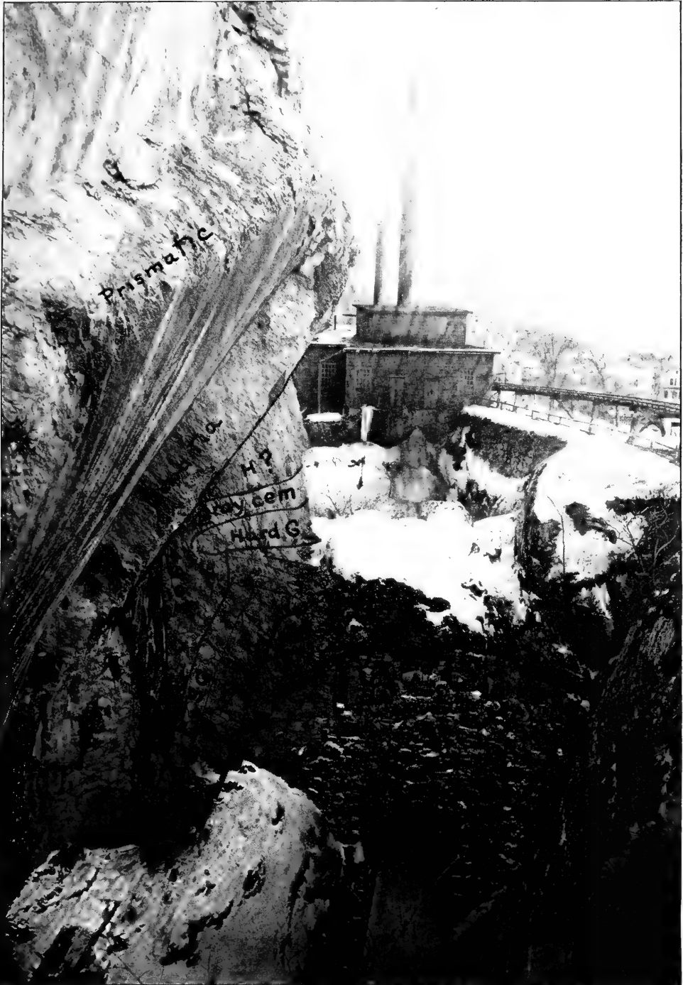
North end of Glory Hole cut, looking from top of second pillar northeast toward the engine house. Note the folded and faulted gray cement in left side of first pillar, and the striated and scaly thrust plane at the bottom of the Prismatic cement in the hanging wall. The foot wall is Wilbur limestone.
