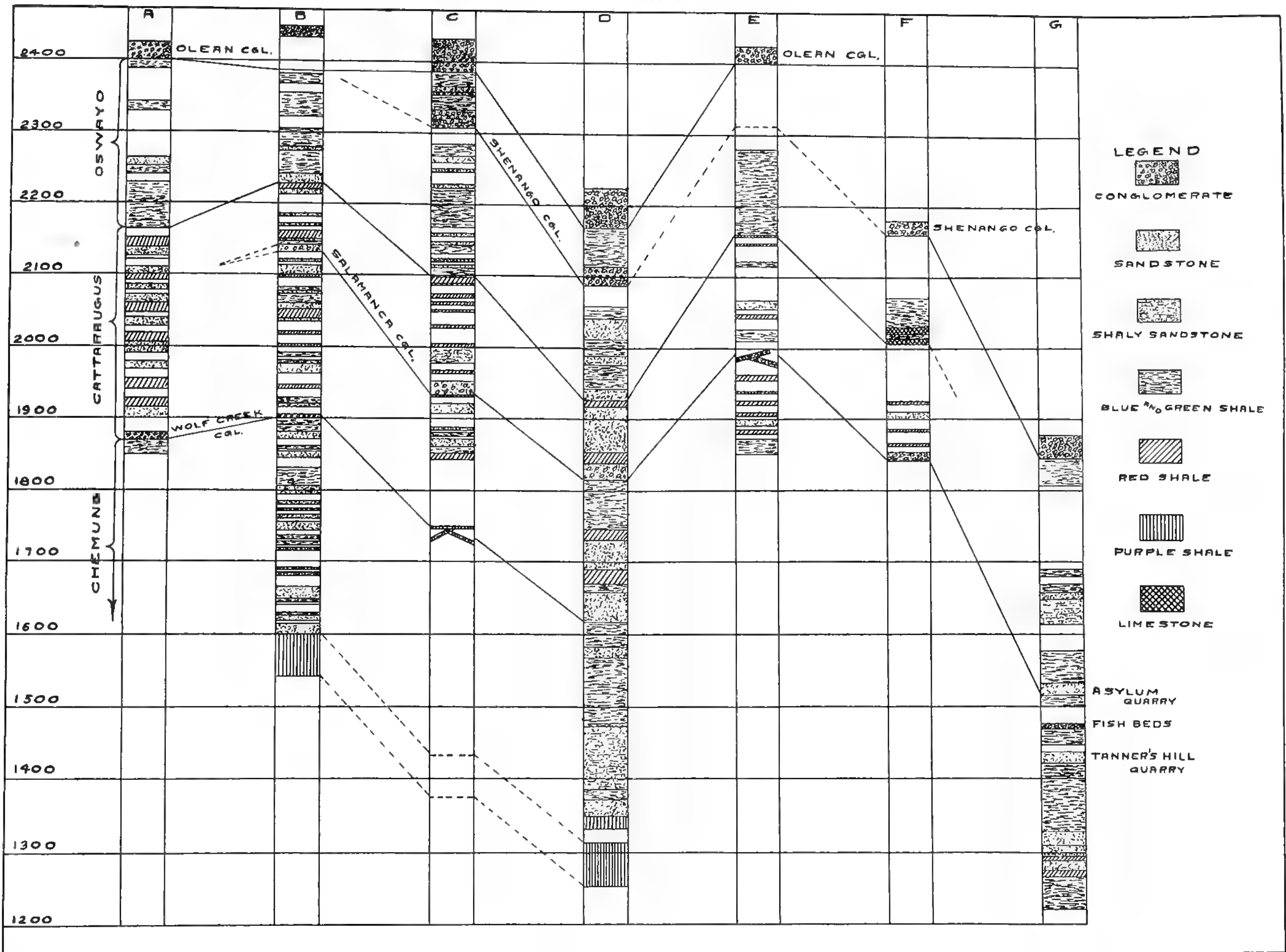
Columnar sections: A, Genesee rock city; B, Mt Hermon-Flatiron; C, Knapp's creek; D, Dennis well, Bradford; E, Limestone; F, Wolf run east of Corydon; G, Warren Pa. (the last after Randall)
