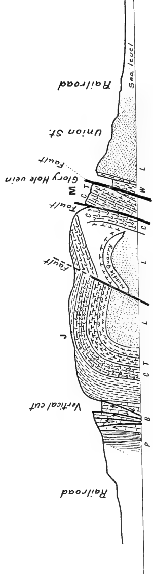
Section I, through middle of Vlightberg.
