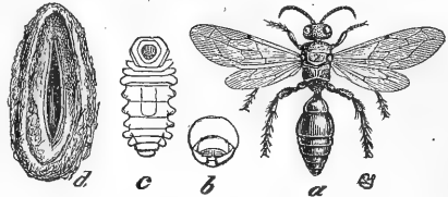
FIG. 4.—The white grub parasite, TIPHIA INORNATA .
