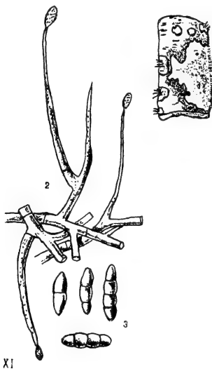
Fig. 46 Monacrosporium carestianum . Reproduced from Ferraris (1904).
