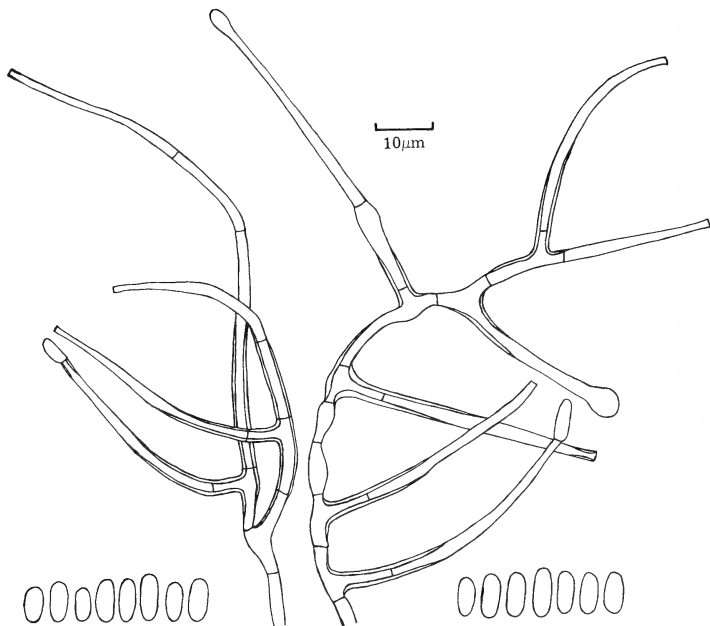
Fig. 27 Monocillium state of Niesslia cladoniicola (CBS 960.73). Reproduced from Hawksworth (1975b : 195).
