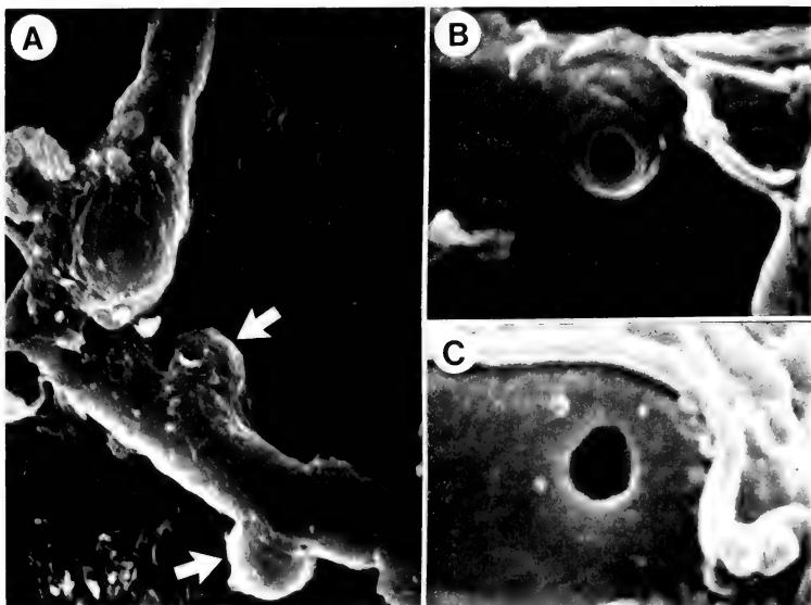
Fig. 13 Dictyophrynella bignoniacearum (URM 28007—holotype). A, Mycelium with hyphopodia (arrows) and conidium ( \times 3500 ). B-C, Scars left by the secession of conidia ( \times 12\ 000 ). A-C Scanning electron micrographs.
