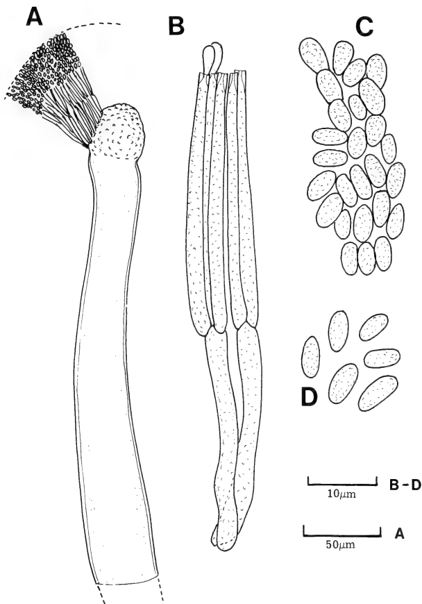
Fig. 45 Glioscephalis pulchella (PAD—holotype), A, Conidiophore apex. B, Arrangement of conidiogenous cells. C-D, Conidia.
