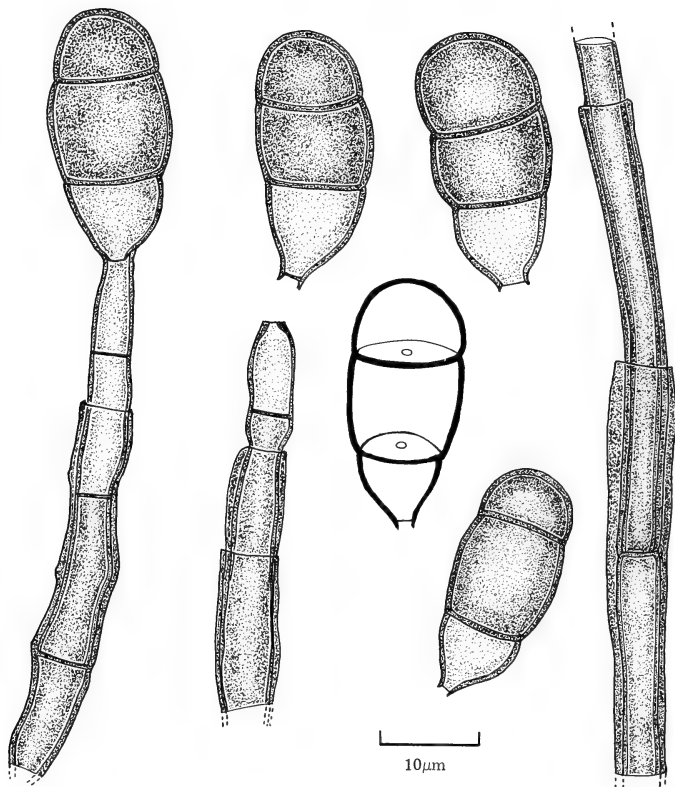
Fig. 14 Endophragmiella hughesii (IMI 217271—holotype).
