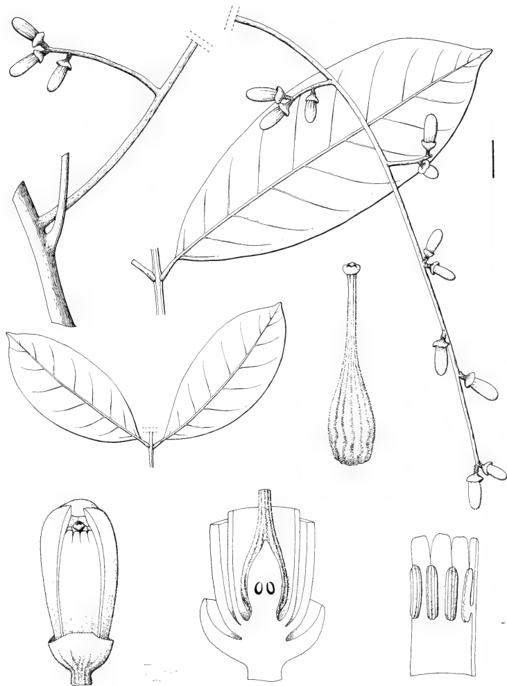
Fig. 7 Chisocheiton vindictae Mabberley. From Pringgo Atmodjo 428: leaf apex, lateral leaflet and inflorescence (scale = 2 cm), flower (scale = 5.0 mm), half flower: base, pistil and part tube (scale = 2.5 mm).
