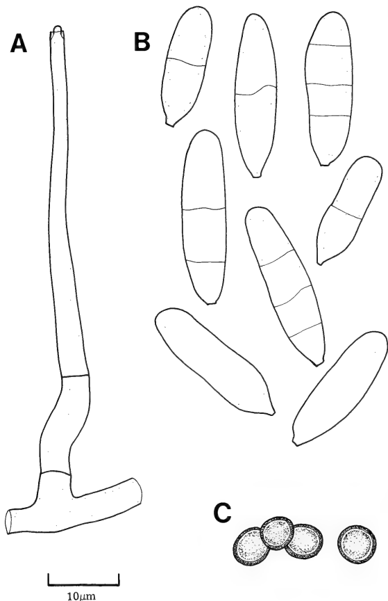
Fig. 44 Cyliandrocarpon lichenicola (PAD—holotype). A, Conidiophore. B, Conidia. C, Chlamydozooids.
