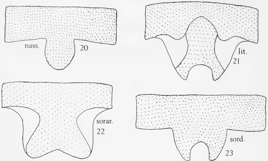
FIGS. 20-23. Tenthredopsis hypopygia : 20, nassata ; 21, litterata ; 22, soraria ; and 23, sordida .
