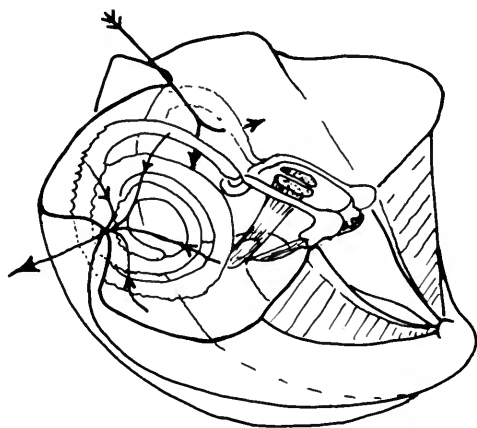
Fig. 94 Diagrammatic reconstruction of the musculature of Cyrtina hibernica sp. nov., viewed laterally. C = crura, with the stump of the jugum; Ad = dorsal adductor muscle scar; Dd = dorsal diductor muscle point of attachment, the cardinal process; Pd = dorsal attachment, on the inner socket ridge, of the pedicle adjustor muscle, with its origin from the pedicle capsule, Pc; Del = part of the delthyrial cover; T = tichorhinum, accommodating the ventral ends of the diductor muscles; P = the distal end of the pedicle; Pc = pedicle capsule, from the ventrolateral margin of which extend short adjustor muscles attached to the inner surfaces of the dental plates; Av = ventral attachment area of the adductor muscle; Ms = posteriorly high median septum, accommodating the muscle; V = floor of the ventral valve.
