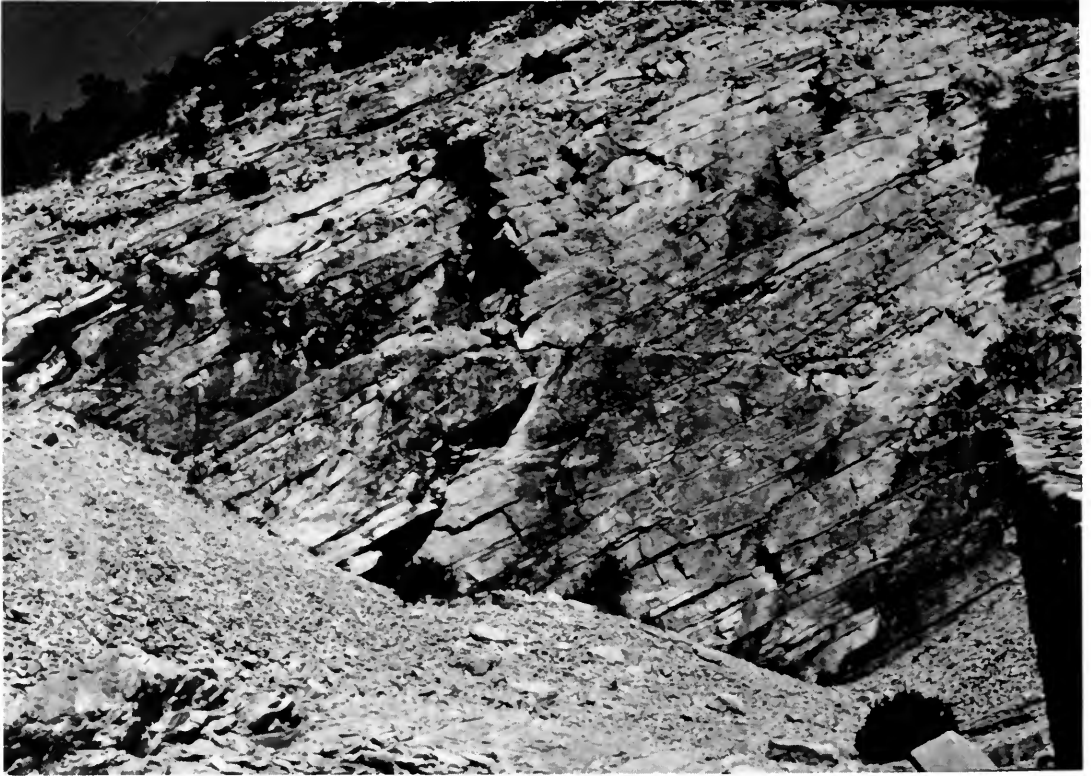
Fig. 1 Rubies Quarry, Lérida Province, Spain: general view. Photograph: H. W. Ball.
