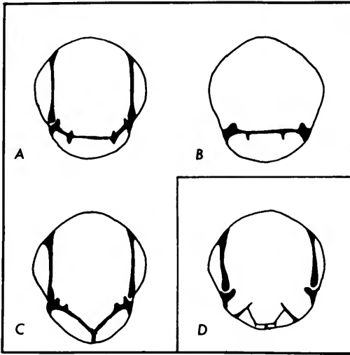
Fig. 171 Stylized cross sections of Cryptonella (A), Alwynia (B), Girtyella (C) and Beecheria (D); A–C are cryptonellaceans while D is a dielasmatacean. Ventral valves are drawn uppermost. The sections illustrate the differences in the disposition of the crural bases to the outer and inner hinge plates – they project dorsally and ventrally in Cryptonella , dorsally in Alwynia and ventrally in Girtyella . In Beecheria the crural bases are supported by thickened outer hinge plates, the inner hinge plates forming an almost sessile septalium containing muscle scars.
