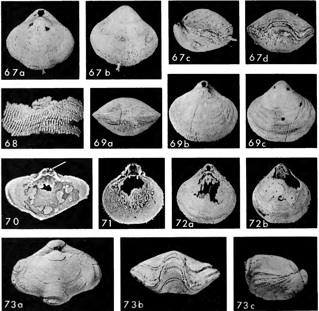
Figs 67–73 Cleiothyridina deroissyi (Léveillé). Fig. 67a–d, complete shell viewed dorsally, ventrally, laterally and anteriorly. BB63461, \times 2 . Fig. 68, fragment of a ventral valve with well-preserved ornamentation. BB63466, \times 4 . Fig. 69a–c, young shell viewed anteriorly, dorsally and ventrally; the radially-aligned spinose lamellae can be seen, and the ventral valve is bored medially. BB63462, \times 2.5 . Fig. 70, dorsal valve interior, looking posterodorsally to show the cardinal process, foramen (arrowed), and sockets. BB63464, \times 2.5 . Fig. 71, juvenile dorsal valve interior with teeth and umbo of the ventral valve remaining attached; the crura extend from the edge of the hinge plate. BB63465, \times 6 . Fig. 71a, b, incomplete young shell viewed dorsally and ventrally; the ventral valve is bored medially. BB63463, \times 3 . Fig. 73a–c, adult shell from the Tournai region of Belgium, viewed dorsally, anteriorly and laterally. BM(NH) 65002, \times 1 .
