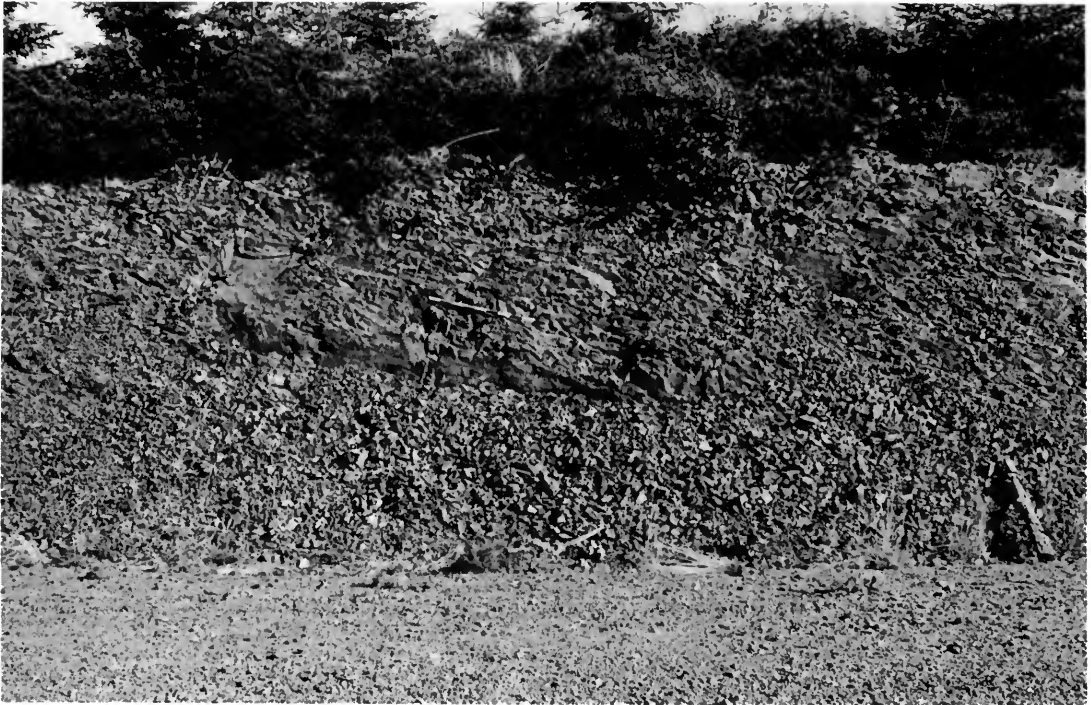
Fig. 61 Stratotype base of the Aeronian Stage, Trefawr track, base of Loc. 72, Grid Reference SN 8380 3953, northern Llandovery area. The Trefawr track has continuous rock exposures for several hundred metres either side of this locality (see Figs 59 and 60).
