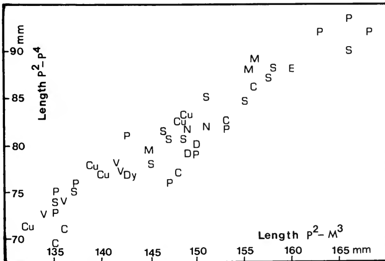
Fig. 6 P^2 - P^4 length plotted against P^2 - M^3 length. C: Concud, Cu: Cucuron, D: Diavata, Dy: Dytko, E: Eppelsheim, M: Maraghe, N: Nea Mesimvria, P: Pikermi, S: Samos, V: Vathylakkos.
