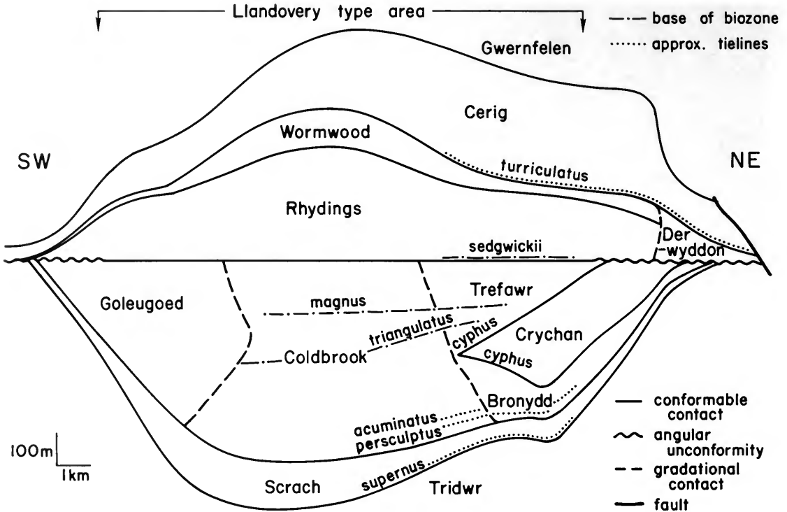
Fig. 68 Graptolite zones in relation to lithostratigraphy in the type Llandoverly area.
