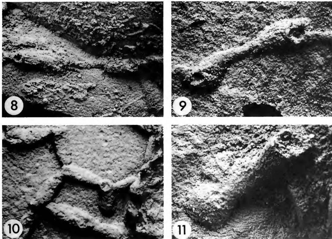
Figs 8–11 Origins of colony growth and ancestrulae in Corynotrypa . Fig. 8, C. voigtiana (King), NMC Schaubroth Collection 3541c; Zechstein Dolomite, Upper Permian; Pössneck, E. Germany. Two zooids growing in opposite directions, \times 52 . Fig. 9, C. inflata (Hall), BMNH D5851a; Lorraine Group, U. Ordovician; Cincinnati, Ohio, U.S.A. Two zooids growing in opposite directions, \times 54 . Fig. 10, C. dissimilis (Vine), BMNH D36468; U. Silurian; Gotland. Ancestrula with protoecium just right of centre, \times 20 . Fig. 11, C. dissimilis (Vine), BMNH R1900a; Wenlock Limestone, Silurian; Dudley, England. Ancestrula with long peristome and bulbous protoecium (lower left), \times 67 .
