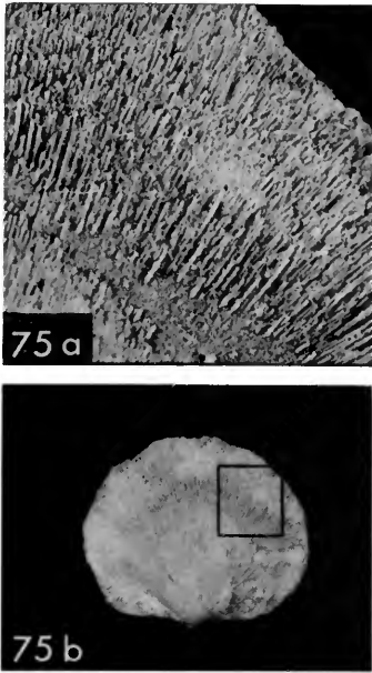
Fig. 75 The external microspinose ornamentation on the dorsal valve of Nucleospira concinna Hall, from the mid-Devonian of Wadsworth, New York, U.S.A. BB19736, (a) \times 10 , (b) \times 1.5 .
