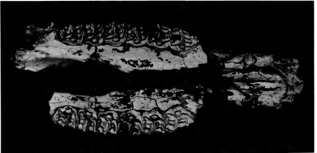
Fig. 2 Hipparion sp. BM(NH) M.11585a-c. Diavata, Thessaloniki, Greece. \times 0.4 . Photo. BM(NH).
