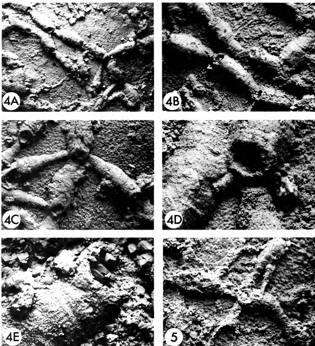
Figs 4–5 Corynotrypa voigtiana (King). 'Middle Zechstein', U. Permian; Pössneck, E. Germany. Fig. 4, BMNH PD6226. 4A, zoids encrusting a crinoid columnal, \times 28 ; 4B, two subparallel branches, \times 52 ; 4C, distolaterally-budded zoids initiating lateral branches with narrower proximal parts than distally-budded zoids, \times 66 ; 4D, incompletely formed bud (kenozoid) terminating against the side of an existing zoid, \times 160 ; 4E, zooidal aperture and non-pseudoporous frontal wall, \times 260 . Fig. 5, BMNH PD6225, typical poorly-preserved colony showing curved zooids and paired lateral branches, \times 58 .
