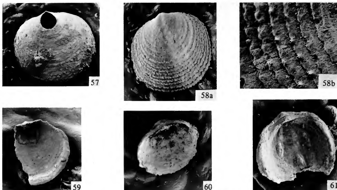
Figs 57–61 Karnotreta adnata gen. et sp. nov. Fig. 57, holotype BB 95414, exterior of pedicle valve, \times 9 ; Fig. 58a, b, paratype BB 95415, exterior of brachial valve: a, \times 9 ; b, enlargement of ornamentation, \times 36 . Fig. 59, paratype BB 95416, interior of incomplete brachial valve, \times 9 ; Fig. 60, paratype BB 95606, interior of brachial valve, \times 8 ; Fig. 61, paratype BB 95417, interior of incomplete brachial valve, \times 9 .
