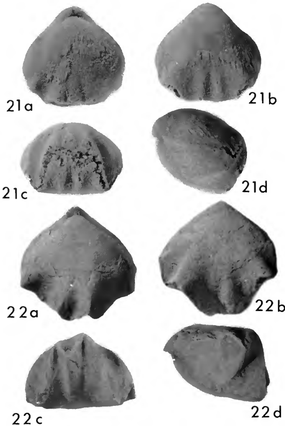
Fig. 21 Coledium seminulum (Phillips). Lectotype, selected Brunton & Champion (1974), viewed dorsally, ventrally, anteriorly and laterally. Viséan of Bolland, Yorkshire. B355, \times 6 .
