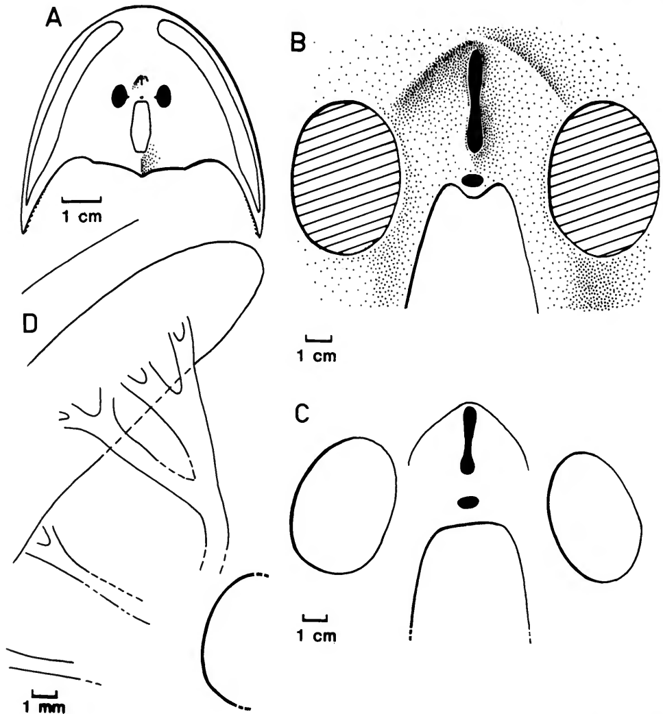
Fig. 17 Mimetaspis glazewskii sp. nov., 'Old Red' I or Ivanie horizons, Ustečko, Podolia, Ukrainian S.S.R. A, reconstruction of the shield based on the holotype (P.20958-9), dorsal view. B, C, orbitopineal and nasohypophysial regions of the shield, based on the holotype (B) and P.20961-4 (C). D, first 's.e.l' canal of the left side in P.20961.
