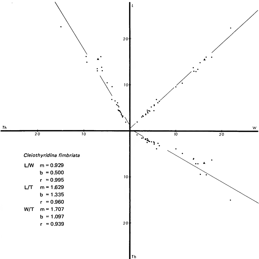
Fig. 66 Cleiothyridina fimbriata (Phillips). Length, width and thickness plots of 28 specimens from Co. Fermanagh, plus the lectotype ( \blacktriangle ) also from Co. Fermanagh. m = slope of regression line; b = intersection point of m with the axis; r = coefficient of correlation.
