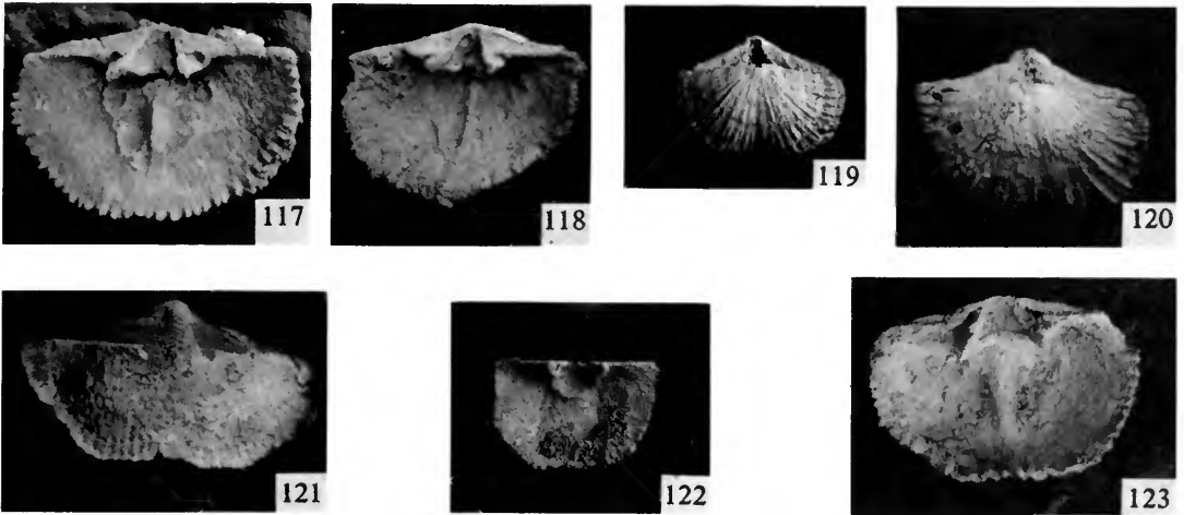
Figs 117–123 Notoscaphtidia revelata gen. et sp. nov. Fig. 117, holotype BB 95476, interior of brachial valve, \times 8 ; Fig. 118, paratype BB 95484, interior of brachial valve, \times 8 ; Fig. 119, paratype BB 95483, dorsal view of conjoined valves, \times 4 ; Fig. 120, paratype BB 95481, dorsal view of conjoined valves, \times 8 ; Fig. 121, paratype BB 95477, interior of incomplete pedicle valve, \times 8 ; Fig. 122, paratype BB 95480, interior of incomplete pedicle valve, \times 4 ; Fig. 123, paratype BB 95479, interior of brachial valve, \times 12 .
