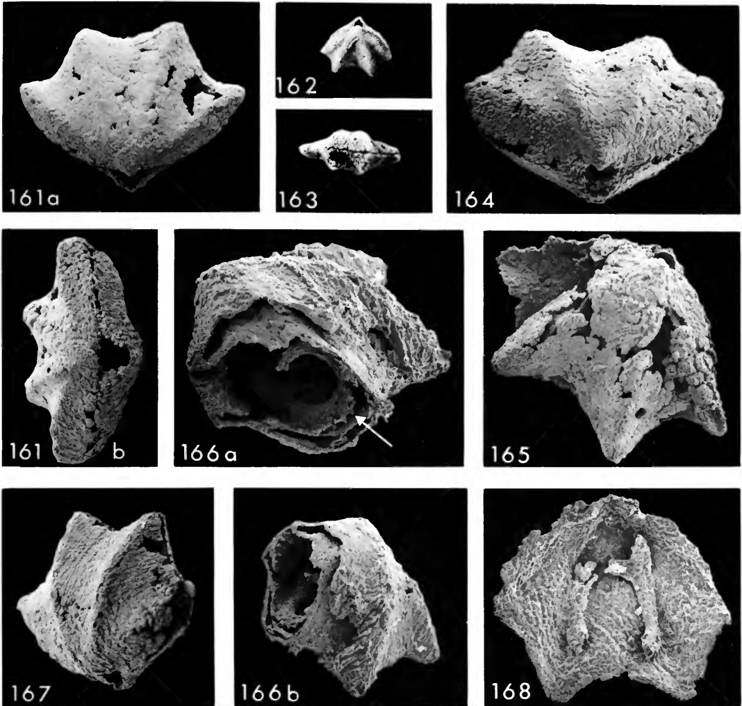
Figs 161–168 Minythyra lophata gen. et sp. nov., from Co. Fermanagh. Fig. 161a, b, holotype, posterodorsal and posterior views. BD147, S.E.M. \times 20 . Fig. 162, dorsal view of complete specimen. BD137, \times 7 . Fig. 163, posterior view of complete specimen. BD135, \times 7 . Fig. 164, posterodorsal view of complete specimen. BD144, S.E.M. \times 28 . Fig. 165, dorsal view of incomplete shell. BD141, S.E.M. \times 27 . Fig. 166a, b, incomplete shell seen laterally, S.E.M. \times 29 , and anterolaterally, S.E.M. \times 22 ; the ventral valve is uppermost and part of a spiralium can be seen on which spinose outgrowths (arrowed) developed on the anterior part of the whorls. BD145. Fig. 167, shell viewed dorsolaterally. BD142, S.E.M. \times 21 . Fig. 168, dorsal valve interior showing shallow sockets (arrowed) and initial sections of the spiralia, including the incomplete jugum; the silica of the internal surface appears to have replicated a mosaic of secondary shell fibres. BD146, S.E.M. \times 26 .
