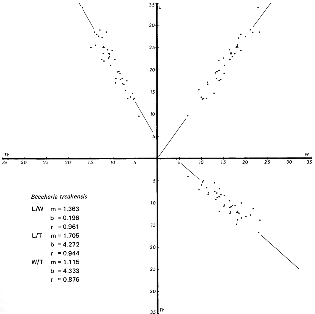
Fig. 211 Beecheria treakensis sp. nov. Length, width and thickness plots of 38 specimens from Treak Cliff, Derbyshire; holotype = ▲. m = slope of regression line; b = intersection point of m with axis; r = coefficient of correlation.
