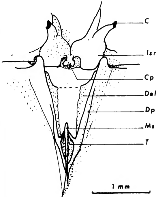
Fig. 93 Drawing of the internal umbonal structures of Cyrtina hibernica sp. nov. (see Figs 101, 102). The dorsal valve is uppermost. C = crura; Isr = inner socket ridge, articulating with a tooth laterally; Cp = cardinal process; Del = deltidial plate; in adulthood, these met medially as a complete cover; Dp = dental plate, descending to fuse with the median septum Ms; T = tichorhinum, developed as a pair of chambers, one each side of the median septum.
