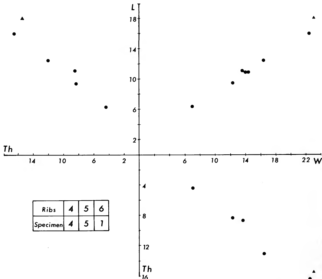
Fig. 5 Pleuropugnoides pleurodon (Phillips). Length, width and thickness plots of seven specimens from Co. Fermanagh, plus the lectotype ( \blacktriangle ) from Bolland, Yorkshire. Only five of the silicified specimens could be measured for thickness. The table shows the number of ribs counted in the sulcus of ten silicified specimens (cf. Ferguson 1966: 363, table 1).
