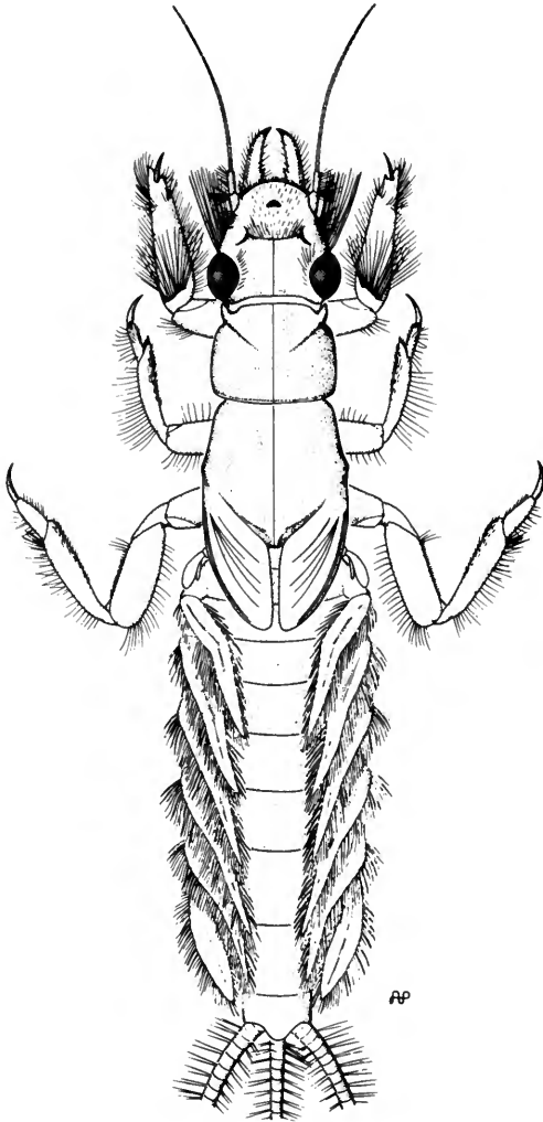
Fig. 5 Tusk-bearing Recent Ephemeroptera nymph, Campsurus sp., \times 4 . After Edmunds et al. 1976: fig. 432.
