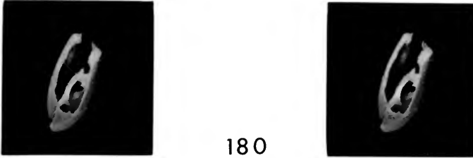
Fig. 180 Cryptonella minranensis sp. nov. Stereoscopic pair of an incomplete shell from Carrick Lough, viewed laterally to show the immature (cryptacanthiiform) brachial loop inside. BB64023, \times 4 ; see also Fig. 173.
