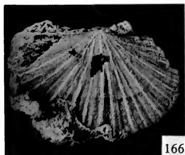
Figs 166–168 Orthidina, gen. et sp. indet. Fig. 166, BB 95588, ventral view of conjoined valves, \times 4 ; Fig. 167, BB 95590, exterior of pedicle valve, \times 4 ; Fig. 168, BB 95589, exterior of brachial valve, \times 4 .
