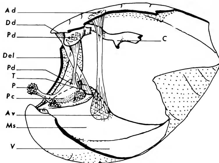
Fig. 94 Diagrammatic reconstruction of the musculature of Cyrtina hibernica sp. nov., viewed laterally. C = crura, with the stump of the jugum; Ad = dorsal adductor muscle scar; Dd = dorsal diductor muscle point of attachment, the cardinal process; Pd = dorsal attachment, on the inner socket ridge, of the pedicle adjustor muscle, with its origin from the pedicle capsule, Pc; Del = part of the delthyrial cover; T = tichorhinum, accommodating the ventral ends of the diductor muscles; P = the distal end of the pedicle; Pc = pedicle capsule, from the ventrolateral margin of which extend short adjustor muscles attached to the inner surfaces of the dental plates; Av = ventral attachment area of the adductor muscle; Ms = posteriorly high median septum, accommodating the muscle; V = floor of the ventral valve.
