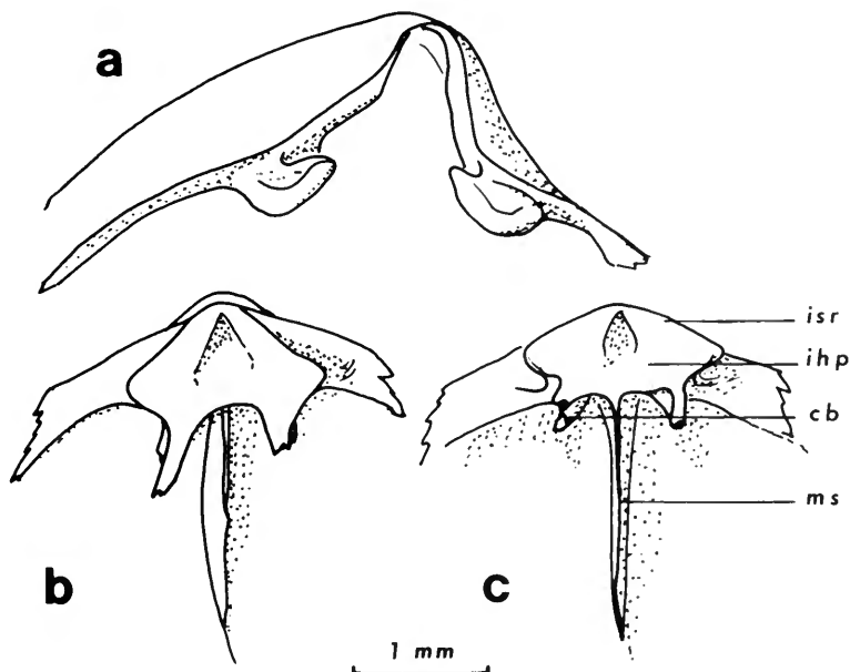
Fig. 9 Drawings from silicified specimens of Tretorhynchia trilatera . Fig. 9a, ventral valve umbo showing the cryptomatodont teeth and open delthyrium (see also Fig. 20). Fig. 9b, c, the cardinalia within a dorsal valve looking dorsally and posterodorsally. isr = inner socket ridge; ihp = inner hinge plate; cb = crural base, and ms = median septum (see also Fig. 12a-c).
