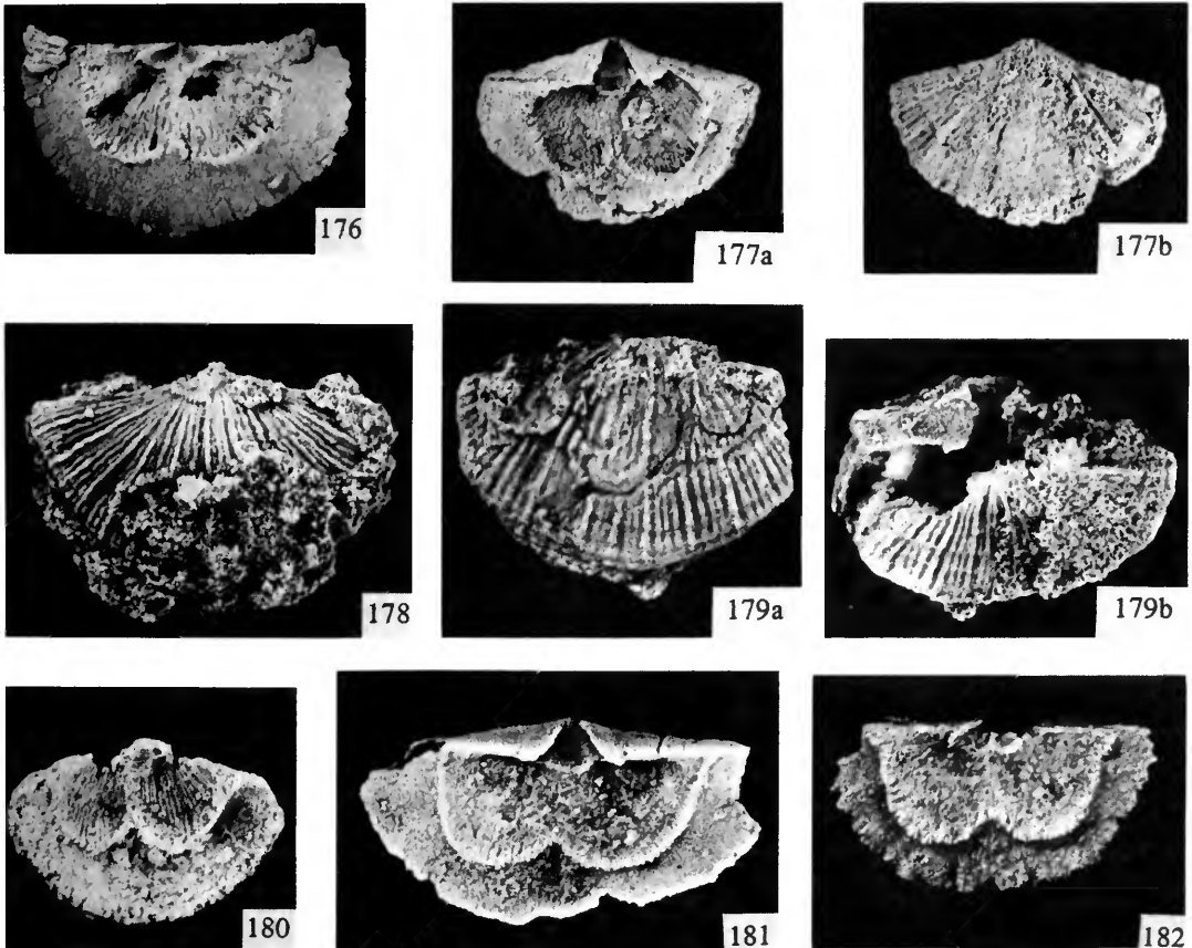
Figs 176–182 Tourmakeadia fimbriata gen. et sp. nov. Fig. 176, holotype BB 95538, interior of brachial valve, \times 5 ; Fig. 177a, b, paratype BB 95539, interior and exterior of incomplete pedicle valve, both \times 4 ; Fig. 178, paratype BB 95543, ventral view of conjoined valves, \times 4 ; Fig. 179a, b, paratype BB 95541, ventral and oblique posterior views of conjoined valves, both \times 5 ; Fig. 180, paratype BB 95544, interior of incomplete pedicle valve, \times 5 ; Fig. 181, paratype BB 95542, interior of incomplete pedicle valve, \times 4 ; Fig. 182, paratype BB 95540, interior of incomplete brachial valve, \times 6 .
