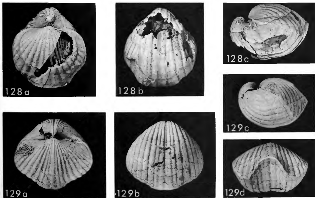
Figs 128–129 Skelidorygma integricosta (Phillips). Fig. 128a–c, incomplete young shell from Co. Fermanagh; viewed dorsally (showing part of the spirulum), ventrally and laterally. BB63694, \times 2 . Fig. 129a–d, lectotype, here chosen, from the Viséan of Bolland, Yorkshire; viewed dorsally, ventrally, laterally and anteriorly. B269, \times 1 .
