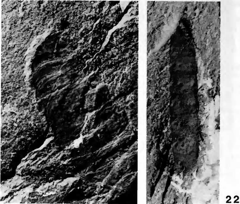
21 Fig. 21 Fly larva, Diptera species 2. In.49650, \times 1.5 . Arrow indicates mandibular sclerite. 22 Fig. 22 Fly larva, Diptera species 3. In.49656, \times 4 .
