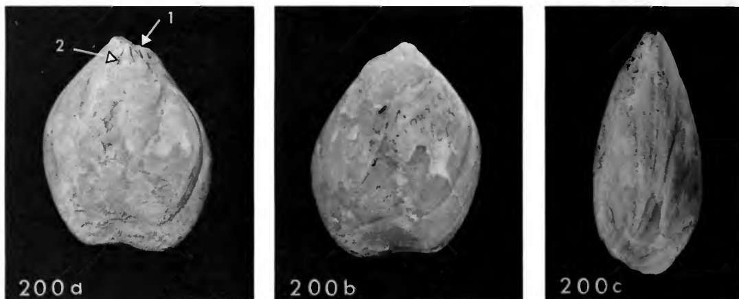
Fig. 200 Beecheria hastata (J. de C. Sowerby). Lectotype selected by Parkinson (1952), viewed dorsally, ventrally and laterally. Arrow 1 points to a dental plate and arrow 2 to the impression of the posterior ends of the hinge plates. From the early Viséan of Limerick, Ireland. B61657, \times 1 .
