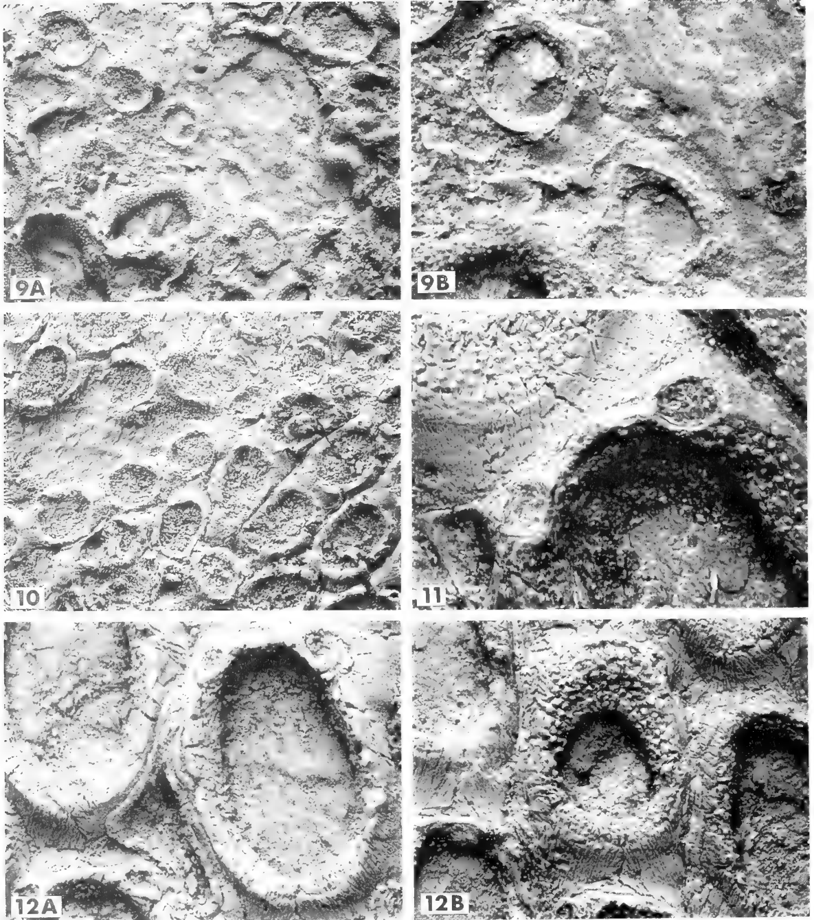
Figs 9–12 Eokotosokum bicystosum (Allan & Sanderson), L. Maastrichtian, Edmonton Group, Horseshoe Canyon Formation, Drumheller marine tongue; Drumheller area, Alberta. Scanning electron micrographs of uncoated specimens imaged using back-scattered electrons. Fig. 9, TMP 91.136.2 (see also Fig. 6); 9A, early zooids arranged in a uniserial line running top left to bottom right of the micrograph, \times 70 ; 9B, ancestrula (top left) with proximal bud (bottom right), \times 170 . Fig. 10, TMP 91.136.3, early zooids of another colony, \times 56 . Fig. 11, BMNH D57396 (see also Fig. 8), large distolateral spine bases of an autozoid, \times 310 . Fig. 12, TMP 91.136.1 (see also Fig. 5), kenozooids; 12A, small kenozooid with reduced calcification infilling area between autozooids, \times 180 ; 12B, large, vicarious kenozooid, \times 173 .
