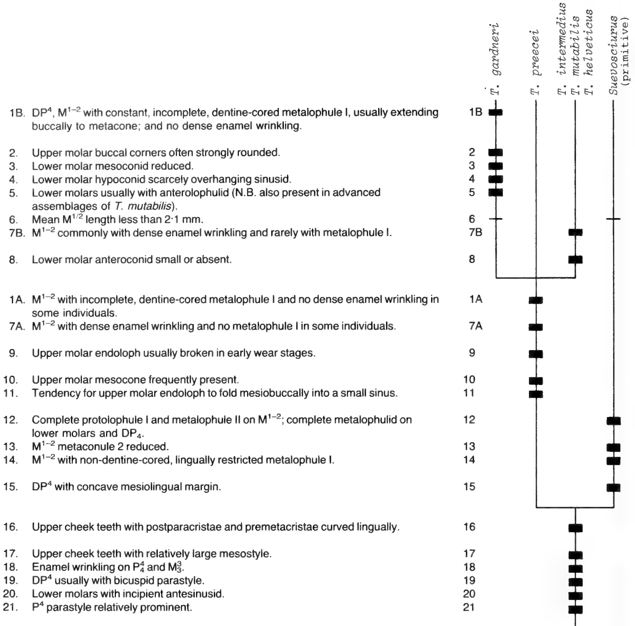
Fig. 16 Cladogram of species of Treposciurus and the genus Suevosciurus . Synapomorphies indicated by broad bar, parallelisms by narrow bar. Characters 1 and 7 are multistate.
