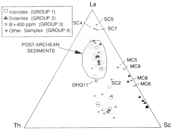
Fig. 11 Ternary diagram, after Taylor and McLennan (1985).
