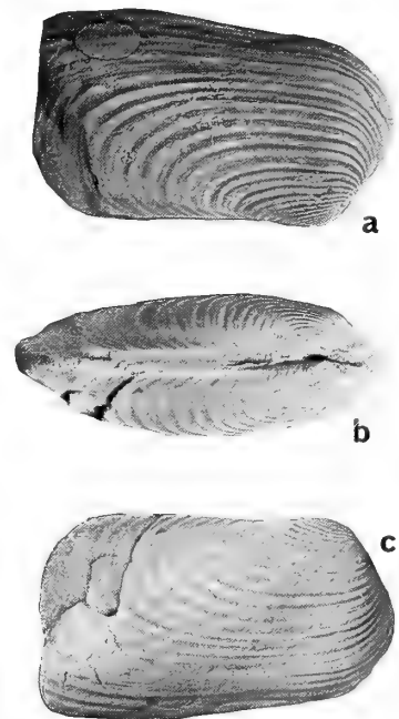
Fig. 23 Wilkingia regularis (King, in de Verneuill ). Lower Carboniferous, Viséan (Asbian), Redesdale Ironstone, Redesdale, Northumberland. BM L45252, Hind Collection, neotype (selected herein) of Venus elliptica Phillips, 1836 ( non Lamarck, 1818). Fig. 23a, left valve; Fig. 23b, dorsal view; Fig. 23c, right valve; all \times 1 .
