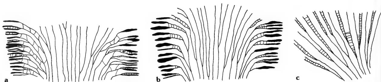
Fig. 8 Longitudinal sketches of the new species described from the Llanbedrog Mudstones. a, Stigmatella oakleyi . b, Pedrogopora taylora . c, Diplotrypa nontabulata .
