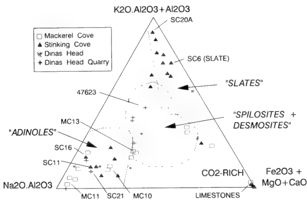
Fig. 5 Ternary diagram (modified after Agrell, 1939) delineating fields for 'adinole', 'spilosite + desmosite' and 'slate'. Samples plotted are all the Dinas Head sediments, and those labelled are referred to in the text.
