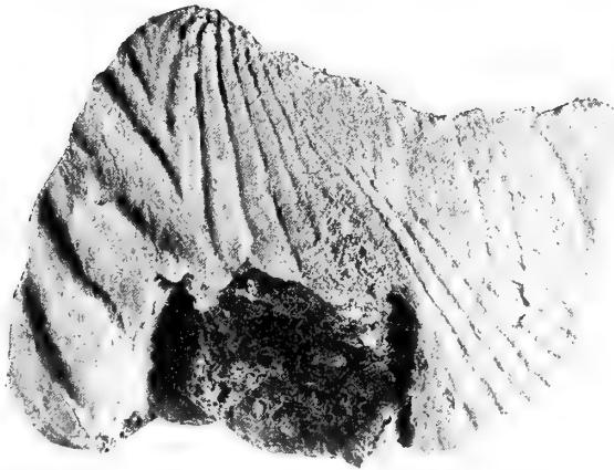
Fig. 18 Siphogrammysia cf. kasanensis (Geinitz). ?Upper Permian, Kazanian, Malaysia, locality 116/F/9B; BM PL5001; \times 2.4 .
