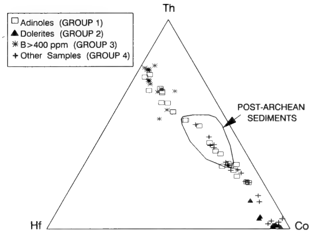
Fig. 10 Ternary diagram, after Taylor and McLennon (1985). Samples plotted are: adinoles — GROUP 1 (open squares); dolerites — GROUP 2 (filled triangles); sediments with B > 400 ppm — GROUP 3 (stars); other samples — GROUP 4 (crosses).
