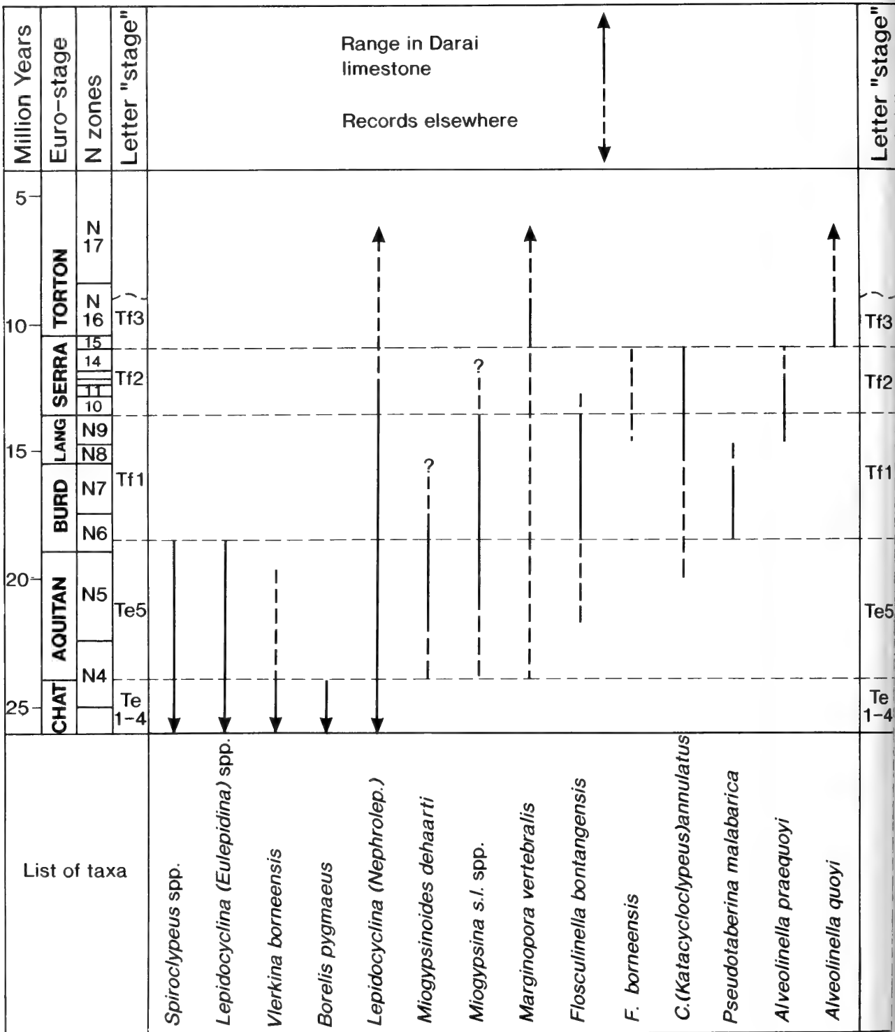
Fig. 3 Known ranges of some important Miocene larger foraminifera in Papua New Guinea and other parts of the Indo-West Pacific region. The smaller benthic marker genus, Austrorillina , is not known above N9 (see Adams, 1984).
