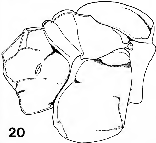
Figs 16–21 16–20, alitrunk, lateral view, of (16) Lissopimpla scutata ; (17) L. excelsa ; (18) Xanthopimpla amon ; (19) X. fraterculus ; (20) X. ankhu . 21, propodeum, lateral view, X. hirsuta .
