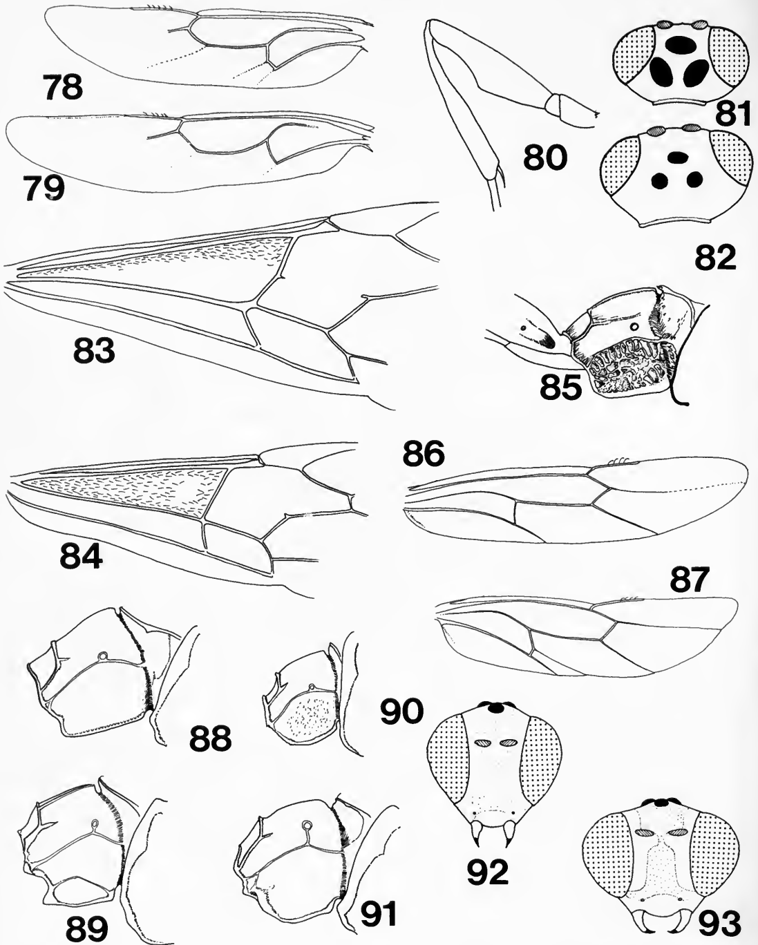
Figs 78–93 78, 79, hind wing of (78) Acrodactyla quadrisculpta ; (79) A. cursor . 80, fore leg, A. micans . 81, 82, head, dorsal view, of (81) A. zekhem ; (82) A. micans . 83, 84, fore wing of (83) Eriostethus maximus ; (84) E. pulcherrimus . 85, propodeum, lateral view, Acrodactyla micans . 86, 87, hind wing of (86) Zatypota rennefer ; (87) Z. velata . 88–91, propodeum, lateral view, of (88) Z. dandiensis ; (89) Z. bingili ; (90) Z. kauros ; (91) Z. phraxos . 92, 93, head, anterior view, of (92) Z. kauros ; (93) Z. celer .
