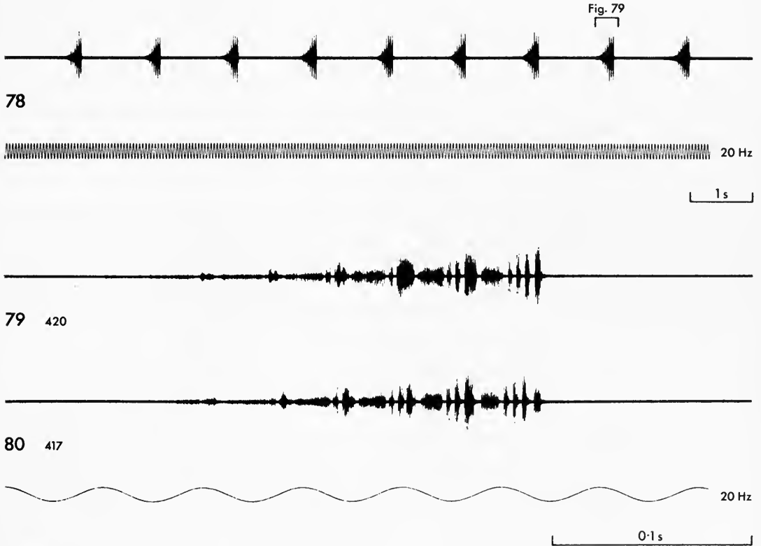
Figs 78-80 Oscillograms of the calling songs of two males of Euchorthippus angustulus . Fig. 79 is a faster oscillogram of the echeme indicated in Fig. 78. Fig. 80 is taken from the song of another male. The small numbers refer to the recordings from which the oscillograms were made and can be used to obtain the full data from Table 2 (p. 108).
