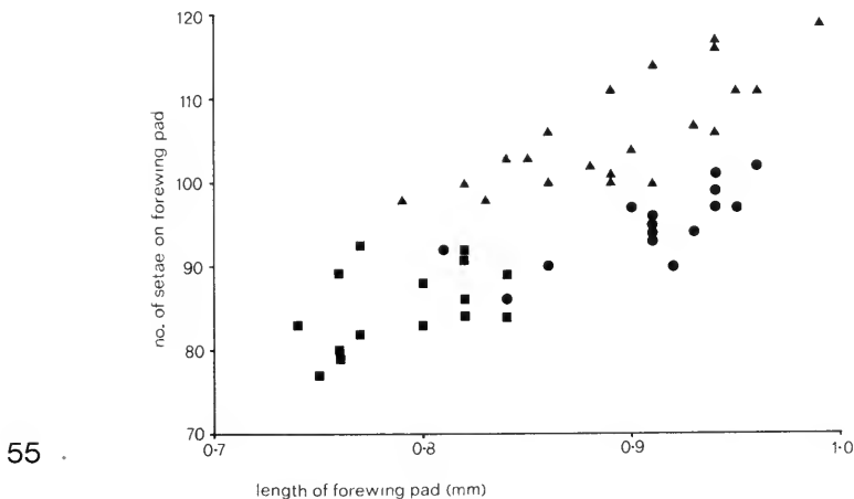
Figs 54, 55 Scatter diagrams comparing characters of Trioza erytrae , T. catlingi and T. menispermicola . 54, adults, length of 1st flagellomere against head width. 55, larvae, number of setae on forewing pad against length of forewing pad.
