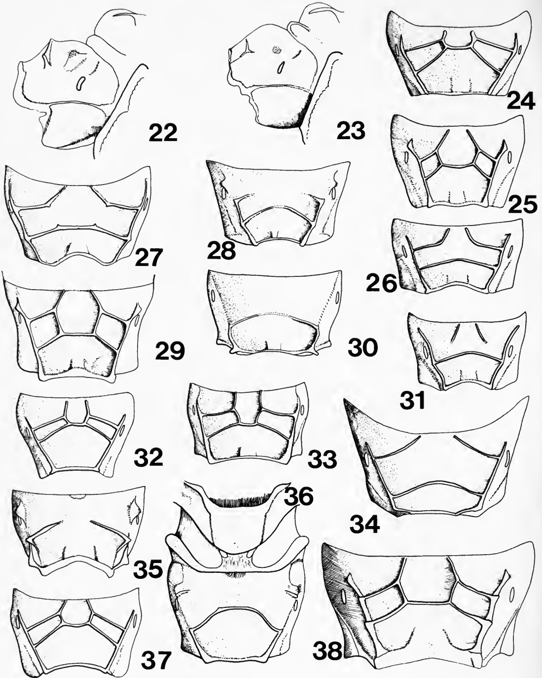
Figs 22–38 22, 23, propodeum, lateral view, of (22) Xanthopimpla quadridens ; (23) X. binodus . 24–38, propodeum, dorsal view, of (24) X. fraterculus ; (25) X. pubidorsis ; (26) X. striata ; (27) X. hiatus ; (28) X. rhopaloceros ; (29) X. arealis ; (30) X. summervillei ; (31) X. amon ; (32) X. ankh ; (33) X. hirsuta ; (34) X. barak ; (35) X. quadridens ; (36) X. terminalis ; (37) X. ochracea ; (38) X. caudata .
