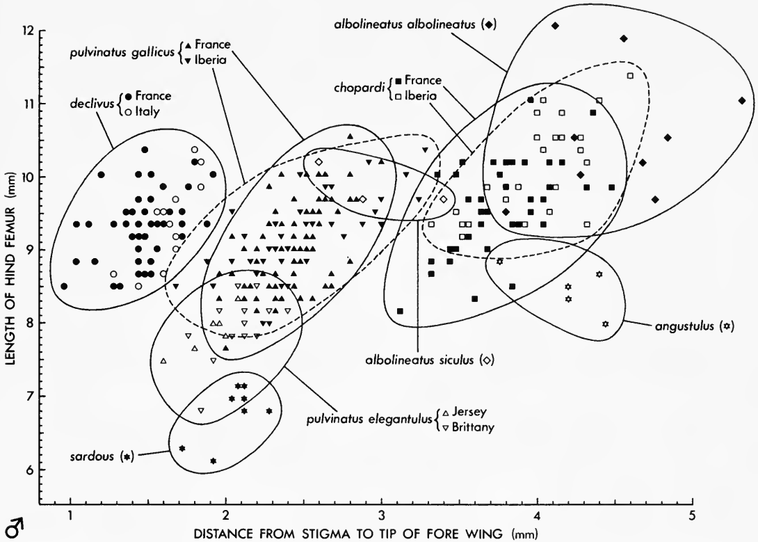
Fig. 10 Scatter diagram showing a plot of the length of the hind femur against the distance from the stigma to the tip of the fore wing in males of Euchorthippus . To facilitate comparison broken lines are used for the two Iberian samples.
