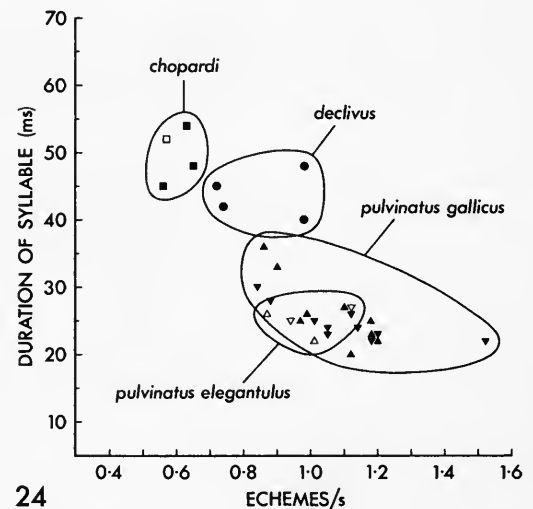
Figs 21–24 Scatter diagrams showing plots of four pairs of characters of the male calling songs of Euchorthippus declivus , E. pulvinatus and E. chopardi . Note that each point represents the mean values of the two characters obtained from one male. The symbols are explained in Fig. 21.
