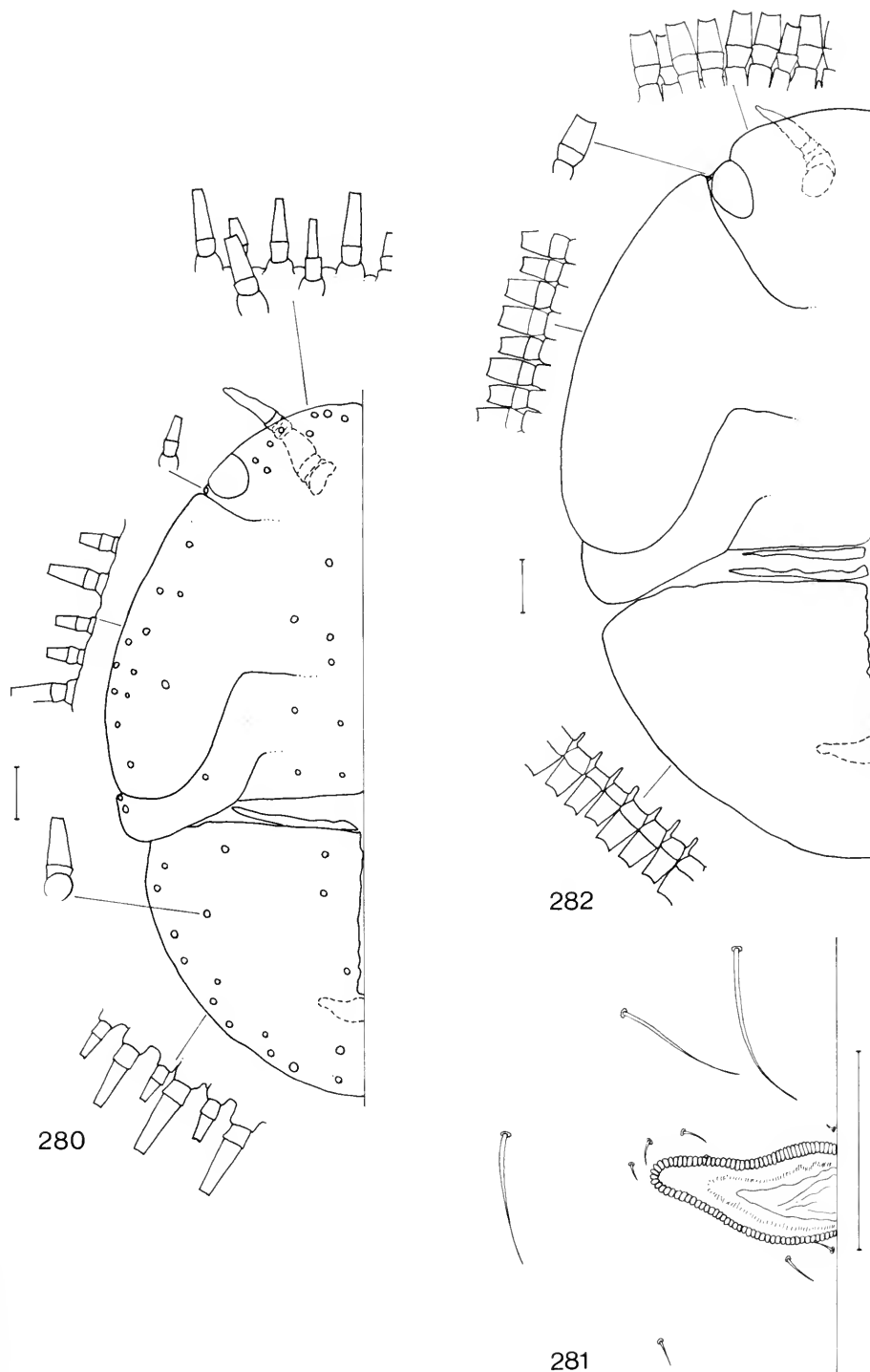
Figs 280–282 Pauropsylla willcocksyi -group, 5th instar larvae. 280, 281, P. willcocksyi ; 280, dorsal view; 281, anal pore area. 282, P. trichaeta , dorsal view.
