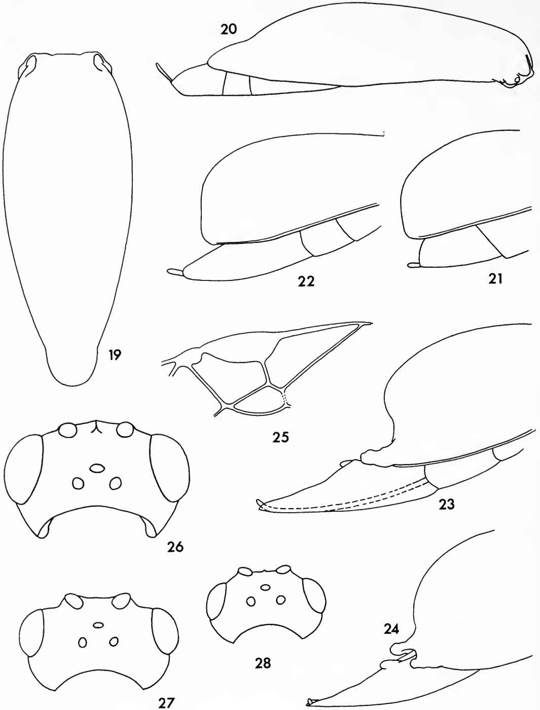
Figs 19–28 19, 20, Ascogaster kasparyani Tobias; (19) carapace, dorsal; (20) carapace, lateral. 21, A. bicarinata (Herrich-Schäffer), carapace, distal. 22, A. caucasica Kokujev, carapace, distal. 23, 24, A. excisa (Herrich-Schäffer); (23) carapace, lateral; (24) carapace, posterolateral. 25, A. annularis (Nees), forewing, anterodistal. 26, A. gonocephala Wesmael, head, dorsal. 27, A. klugii , (Nees), head, dorsal. 28, A. exigua sp. n., head, dorsal.
