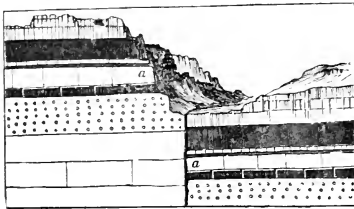
Fig. iv. —Section across a simple fault. (Powell).
