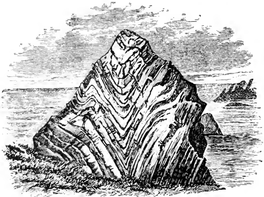
Fig. ii. —Synclinal fold near Banff, Scotland. (Geikie).
