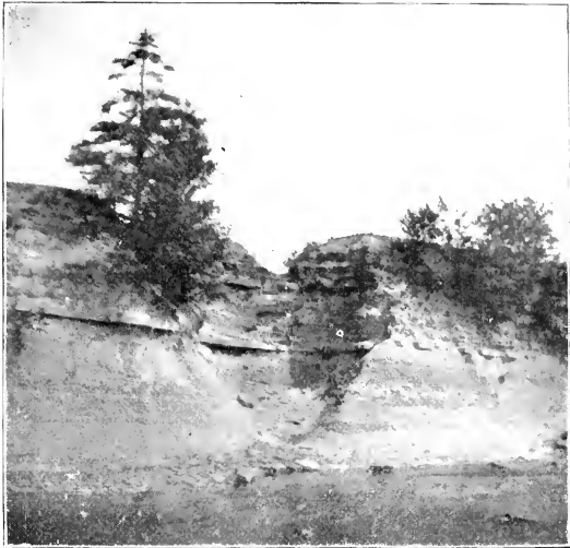
PLATE X.—View of the "corry" in Section 7, showing an example of gorge cutting in an early stage. The backward cutting of the falls produces the gorge, and the downward cutting of the stream the V-shaped trench seen above. The Encrinal limestone is seen near the middle of the cliff.
