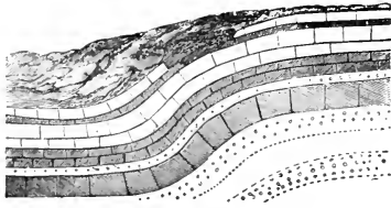
Fig. iii. —A monoclinial fold or flexure. (Powell).
