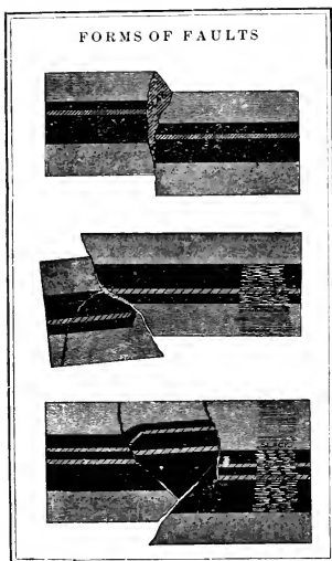
Fig. vi. —Gravity, and simple and compound thrust faults.
