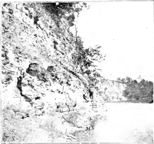
PLATE III. (a).—View of the cliffs in the gorge of Eighteen Mile Creek, above North Evans.
