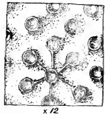
FIG. 60. Fistulicella plana . Enlargement of a portion of the surface, x 12 (after Hall and Simpson).
