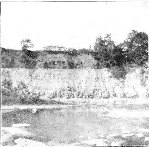
PLATE VII. (a).—View of the upper end of Section 4. The base of the section is formed by the Styliolina limestone, above which are visible the gray and black Genesee, and the Cashaqua and Gardeau shales.
