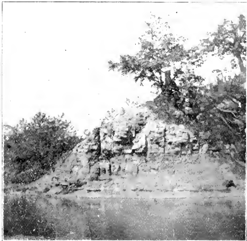
PLATE VI.—View of the lower end of Section 3. The upper portion of the Moscow shales is exposed at the foot of the section. The projecting Styliolina band, the gray and much-jointed black Genesee shales, and a portion of the Cashaqua shales appear above it.
