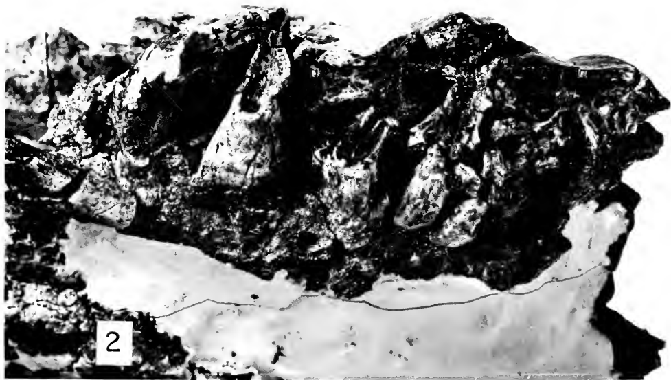
Plate 3. Chilotheridium pottersoni . Fig. 1, LP 2 -M 2 , RP 2 -M 2 of skull No. 1 (70-64K, C9-10), crown view. \times 0.50 . Fig. 2, M 1 (port)-RM 2 of skull No. 2 (70-64K, B12), type, crown view. \times 0.70 .
