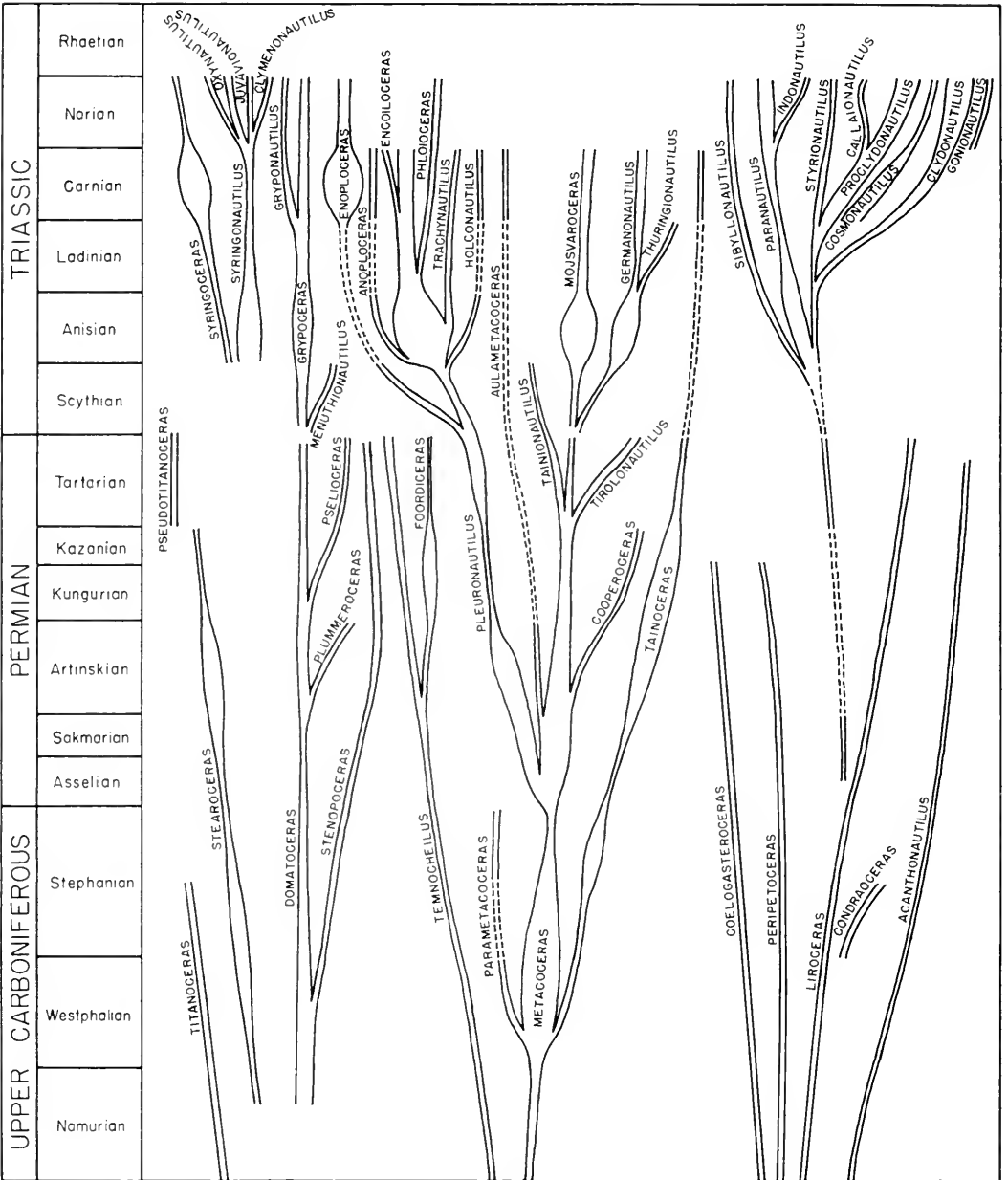
Figure 1. Diagram showing inferred phylogeny and geologic distribution of late Paleozoic and Triassic coiled nautiloids. (Adapted from Kummel, 1953.)
