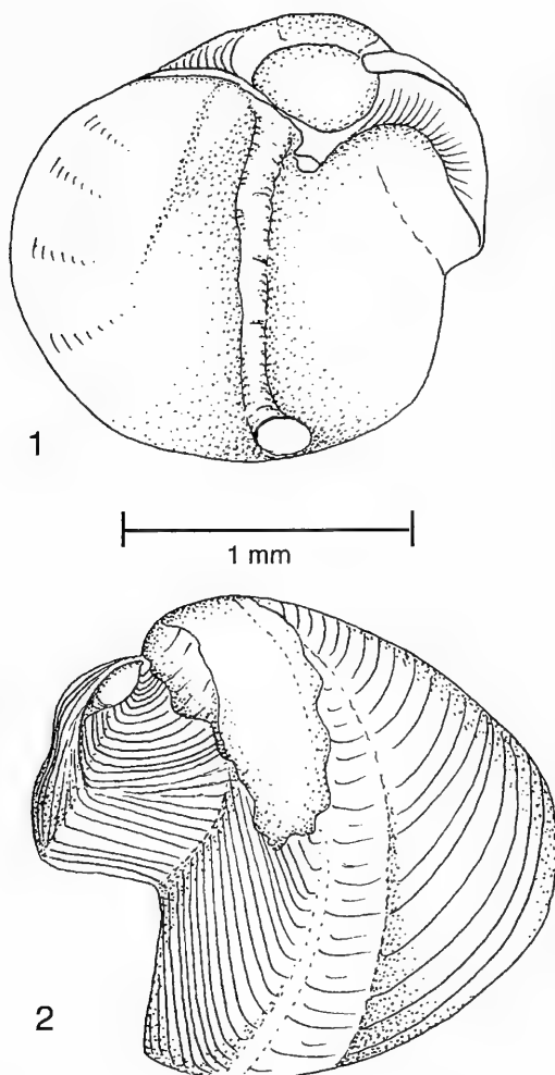
Plate 37. Xyloredo ingolfia Turner from Ingolf Expedition , station 67.
