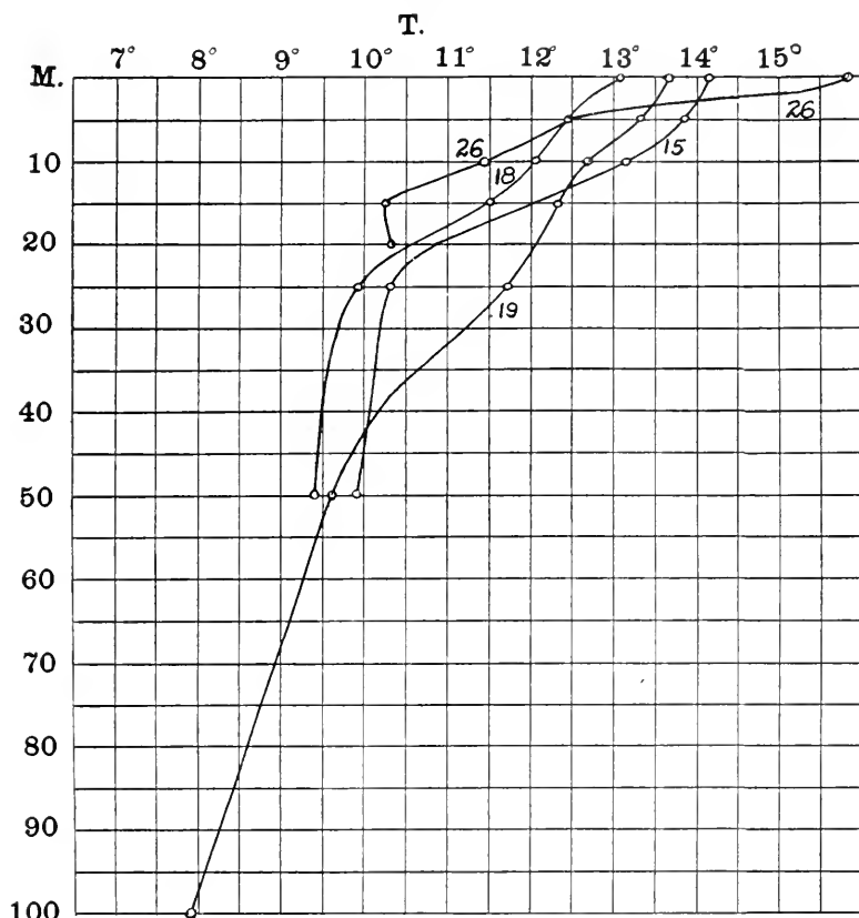
FIG. 4.—Vertical distribution of temperature at successive stations around the shore of the bay (15, 18, 19, 26).
