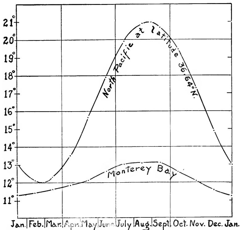
FIG. 23.— Average surface temperature of Monterey Bay, for the year, based on records for 1919-1928 (lower curve), and normal surface temperature for the North Pacific as a whole at the corresponding latitude from calculations by G. F. McEwen (upper curve).
