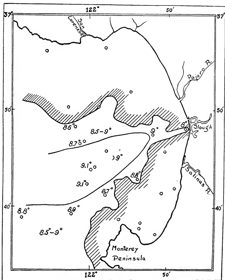
FIG. 8.—Temperature at a depth of 100 meters.
