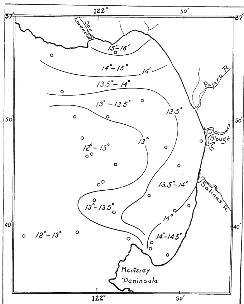
FIG. 2.— Surface temperature, July 1-24, 1928.
