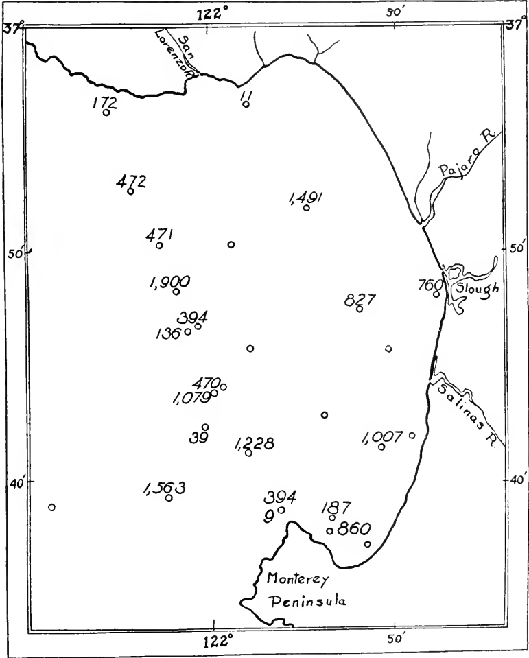
FIG. 43.— Numbers of diatom cells (good and bad condition combined) at the surface, in thousands per liter.
