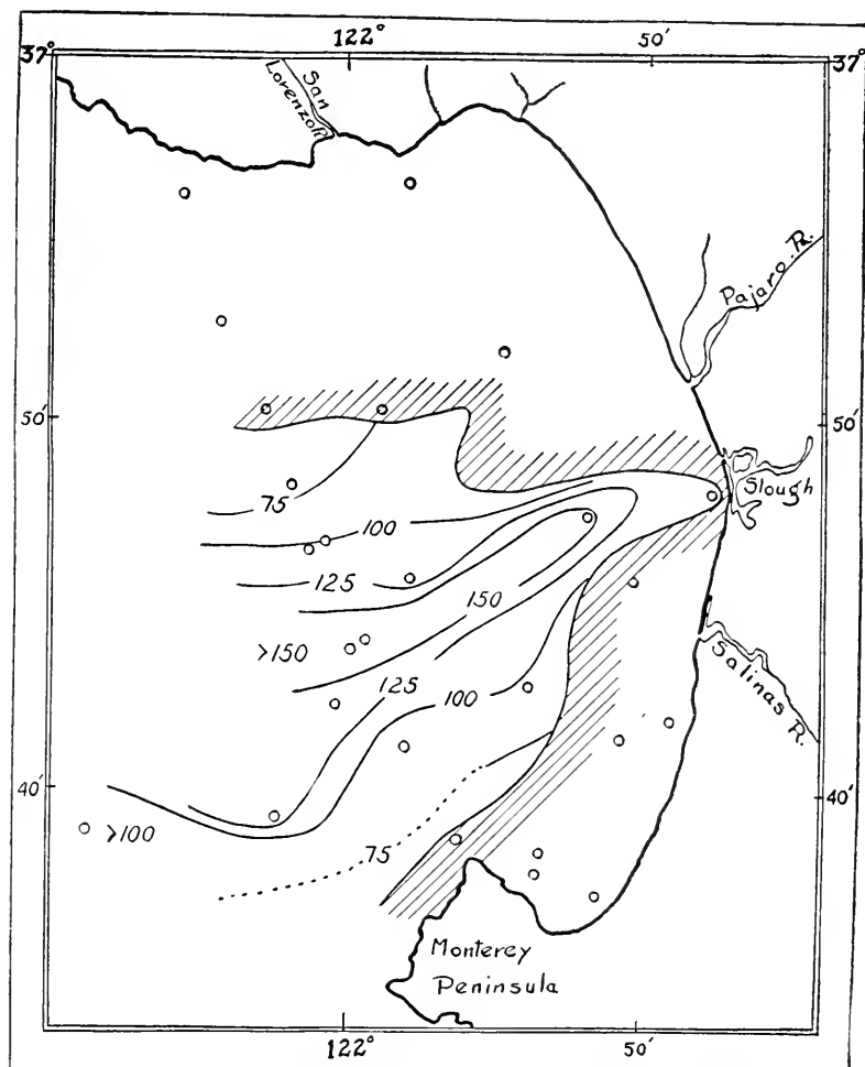
FIG. 18.—Depth in meters below the surface of the isohalobath for 34‰.
