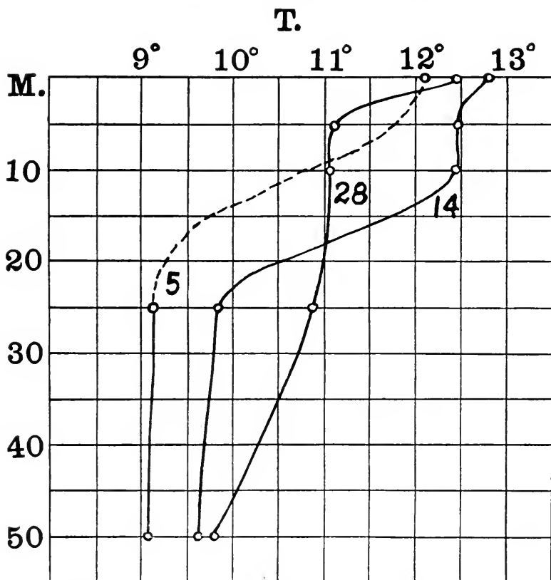
FIG. 22.— Seasonal progression of salinity near Point Pinos, July 5 (Sta. 5); July 16 (Sta. 14); and July 23 (Sta. 28).
