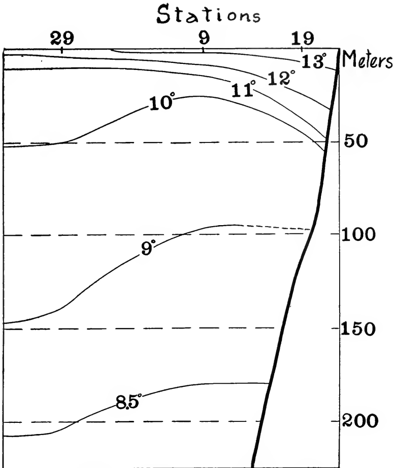
FIG. 6.— Temperature profile, running offshore from Moss Landing, July 12-24.
