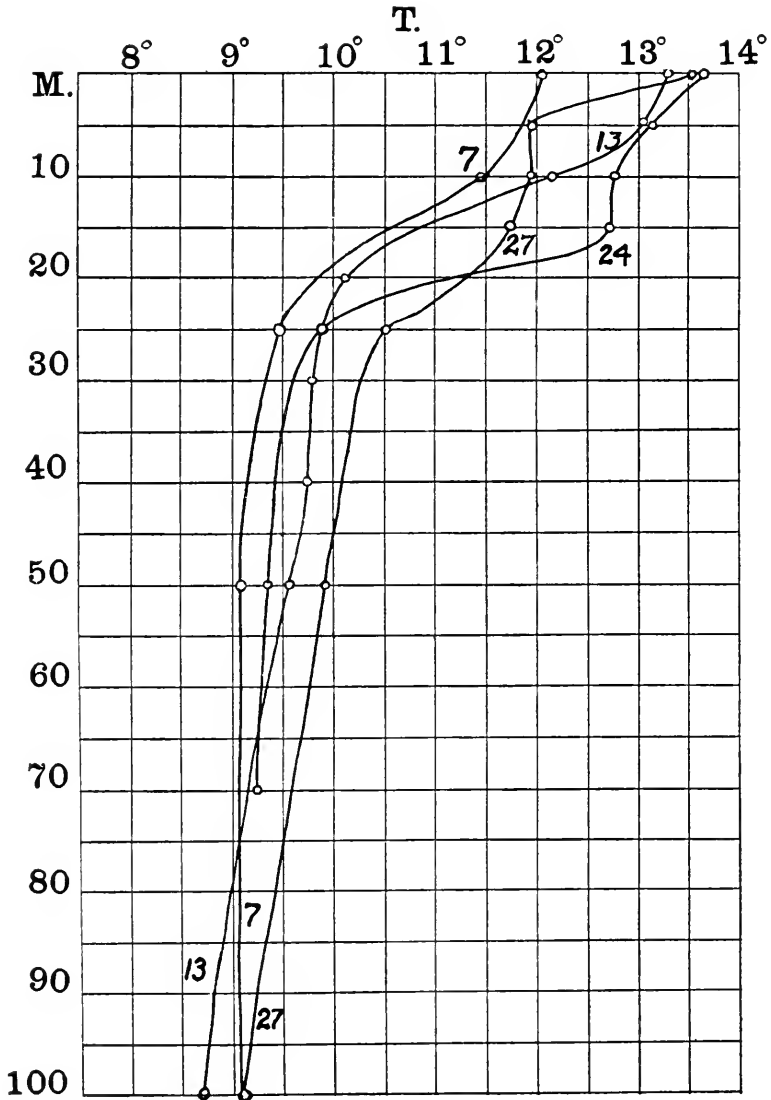
FIG. 3.— Vertical distribution of temperature at representative stations 7, 13, 24, 27) in the upper 100 meters.
