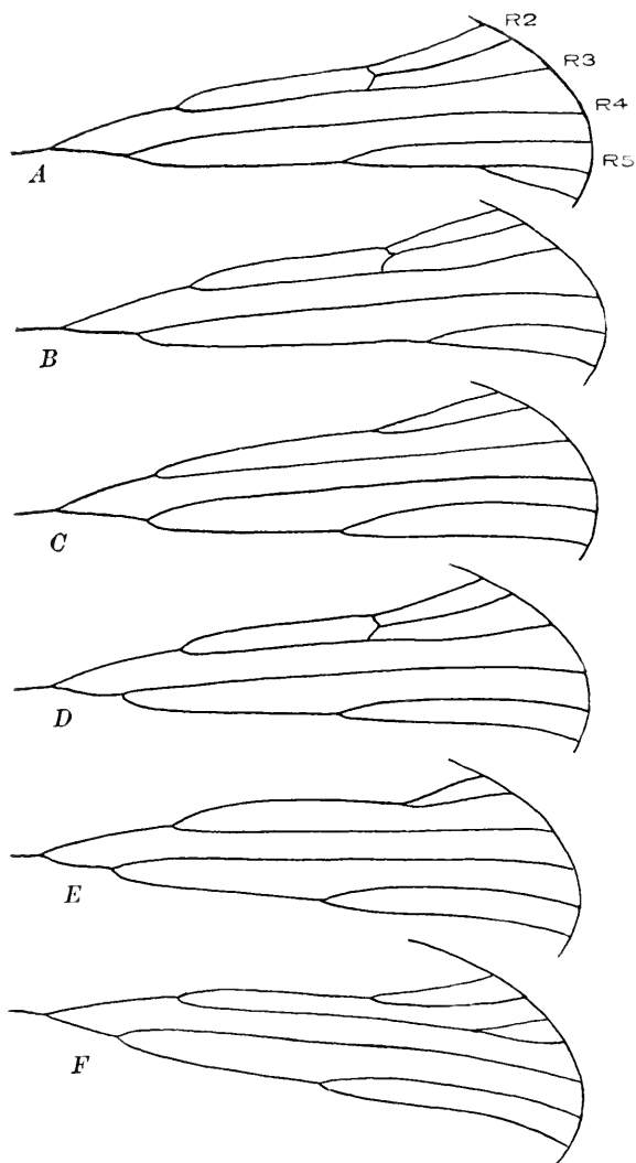
FIG. 2.— Variations in the radial sector of Pernopanorpa inaequalis : A, No. 3021; B, No. 3016; C, No. 3010; D, No. 3019; E, No. 3018; F, No. 3013.
