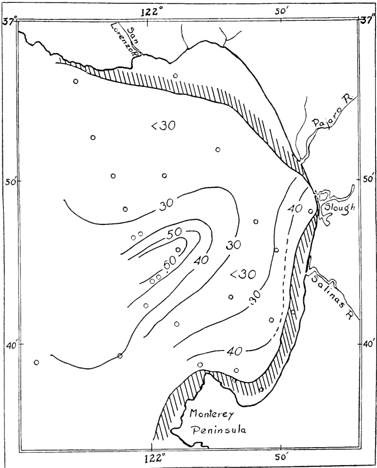
FIG. 19.—Depth in meters below the surface of the isotherm bath for 10°, July 11–24.
