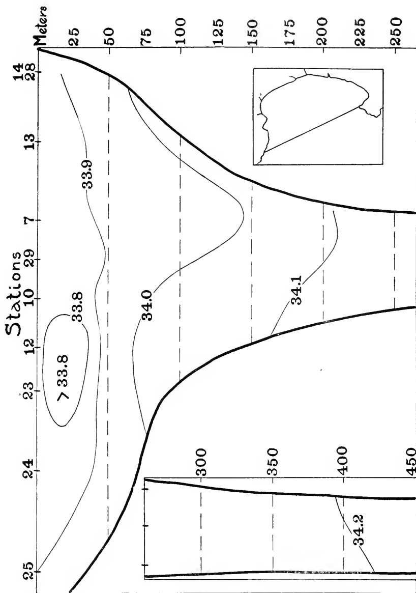
FIG. 15.— Profile of salinity, crossing the mouth of the bay, July, 10-24.
