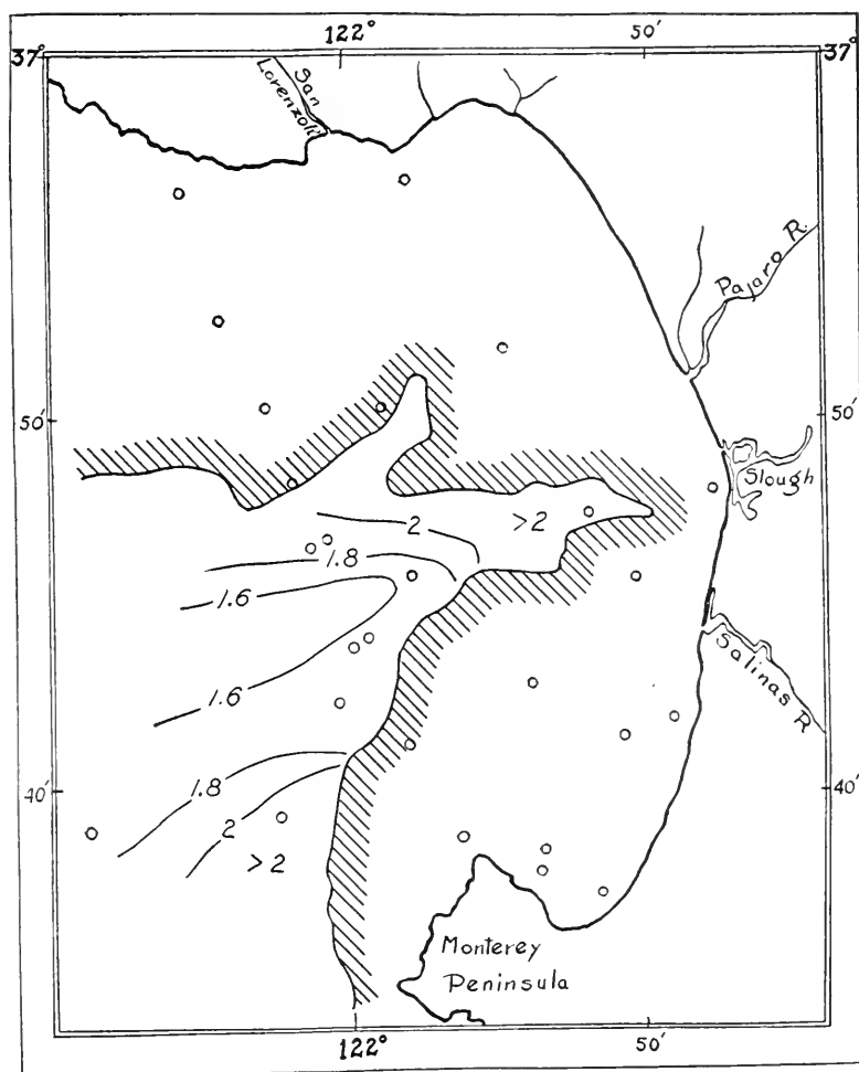
FIG. 33.— Distribution of silicates (in milligrams per liter of SiO 2 ) at a depth of 200 meters.
