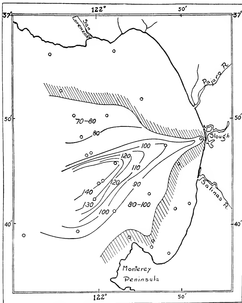
FIG. 17.— Depth in meters below the surface of the isotherm bath for 9°, July 11-24.
