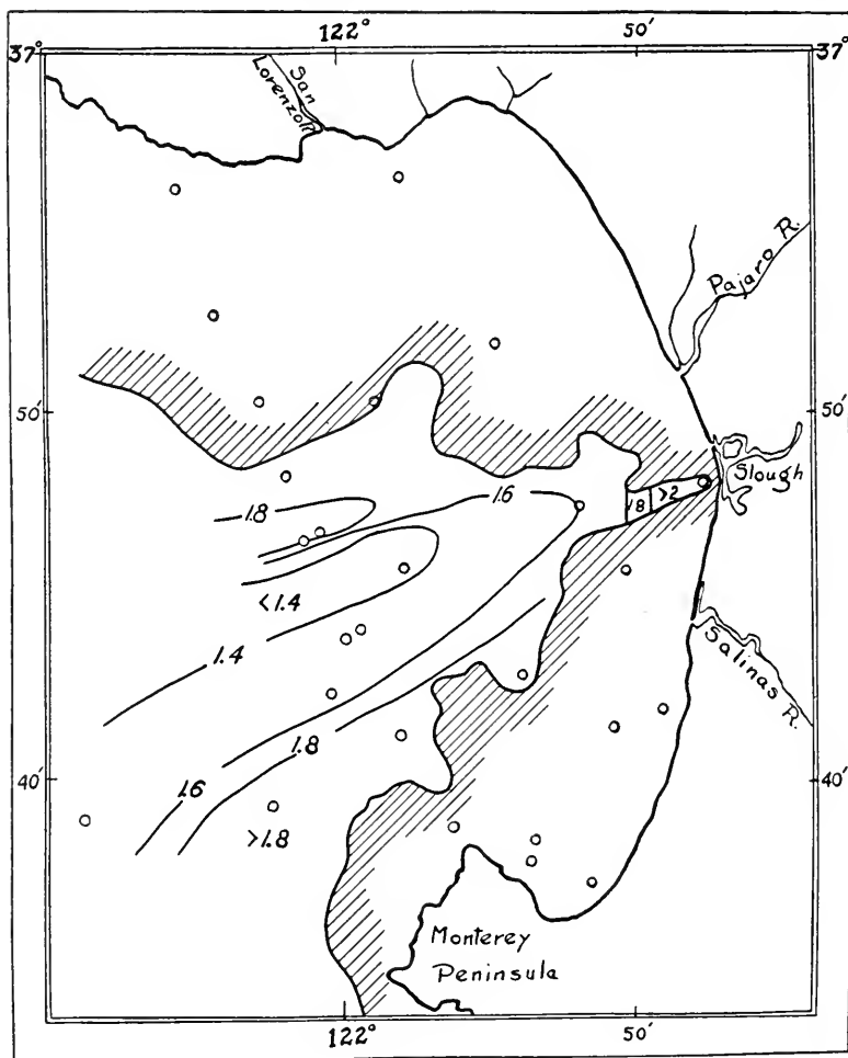
FIG. 29.— Distribution of silicates (in milligrams per liter of SiO 2 ) at a depth of 100 meters.
