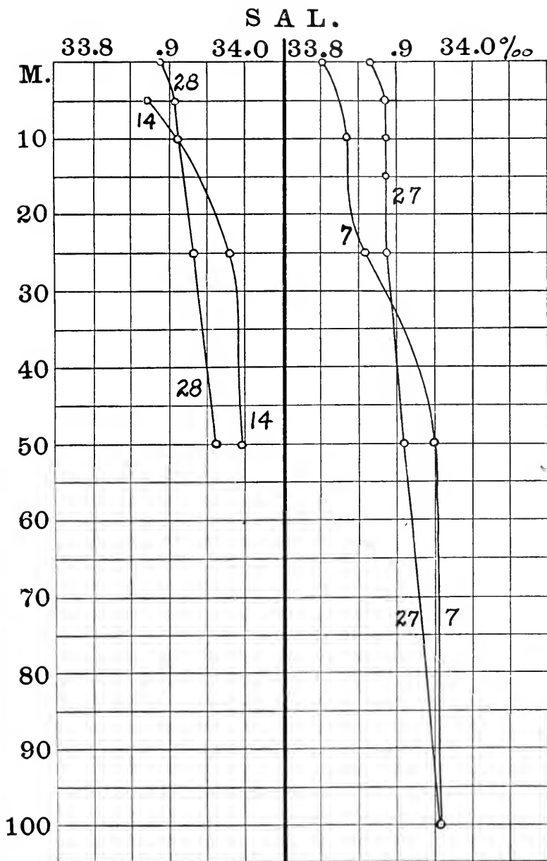
FIG. 13.—Vertical distribution of salinity in the upper 100 meters at pairs of stations off Point Pinos, July 16 and 23 (14, 28); also at the mouth of the bay, July 10 and 23 (7, 27).
