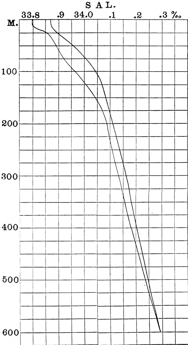
FIG. 16.— Maximum and minimum values of salinity, surface to 600 meters, Stations 8, 10, 17, 27, 29.
