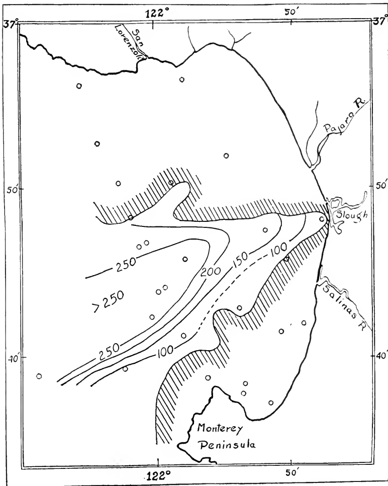
FIG. 36.— Depth below the surface of the layer of 2 milligrams of \text{SiO}_2 per liter.
