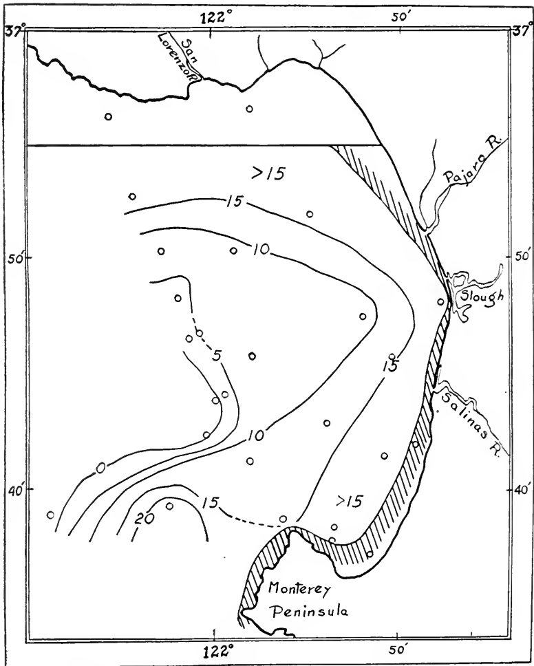
FIG. 39.— Depth below the surface of the layer of .05 milligram P_2O_5 per liter.
