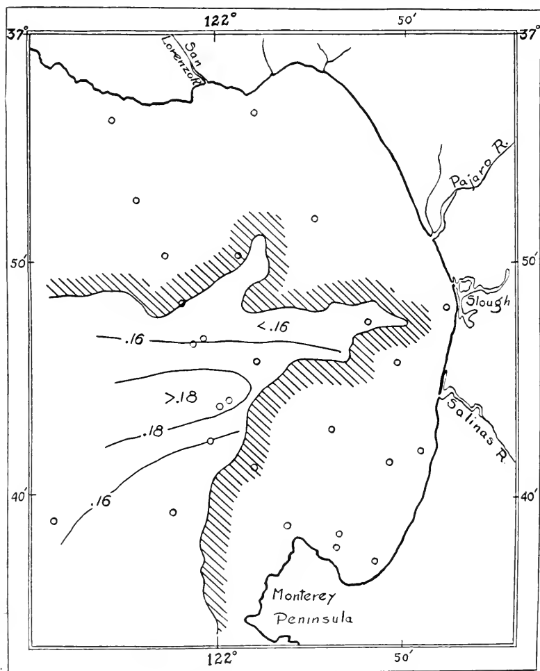
FIG. 32.— Distribution of phosphates (in milligrams per liter of P_2O_5 ) at a depth of 200 meters.
