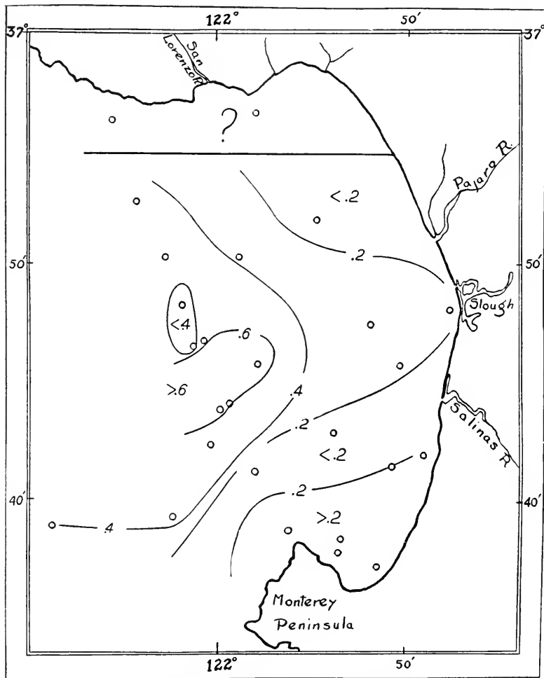
FIG. 25.— Distribution of silicates (as milligrams per liter of SiO 2 ), at the surface.
