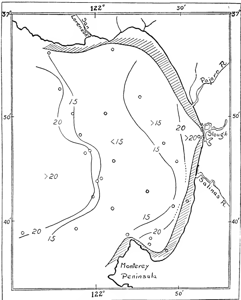
FIG. 20.— Depth in meters below the surface of the isotherm bath for 11°, July 11-24.
