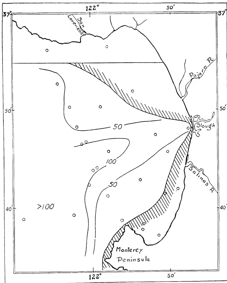
FIG. 38.— Depth below the surface of the layer of .15 milligram P_2O_5 per liter.
