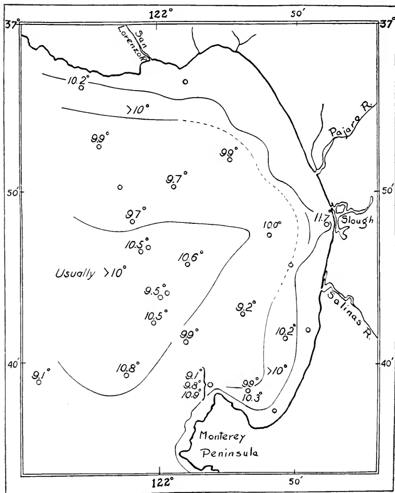
FIG. 5.— Temperature at a depth of 25 meters, July 1-24, 1928.
