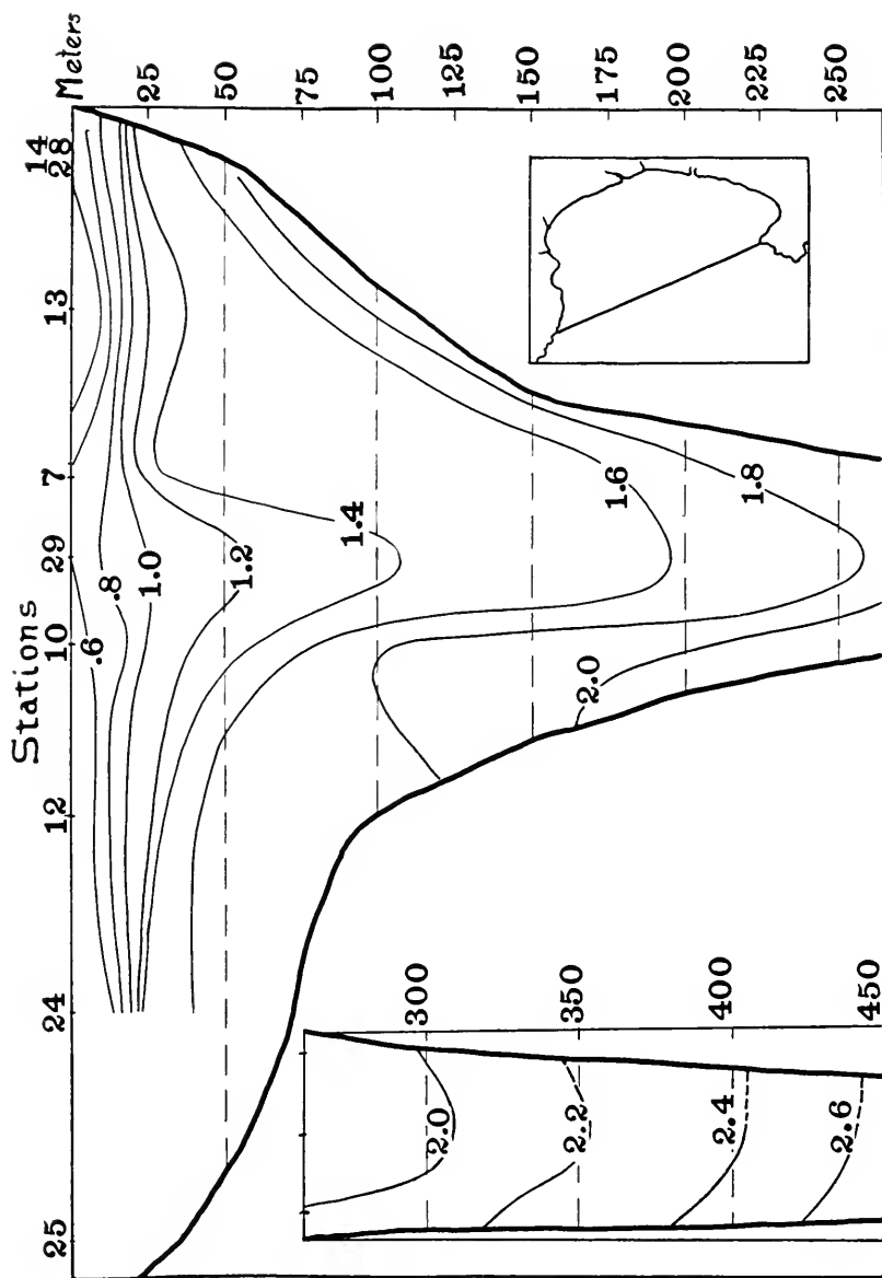
FIG. 30.—Profile across the mouth of the bay for silicates (in milligrams per liter of SiO 2 ).
