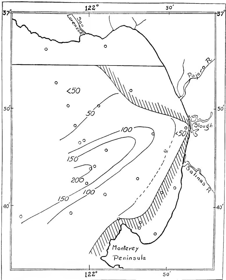
FIG. 37.— Depth below the surface of the layer of 1.6 milligrams of SiO 2 per liter.
