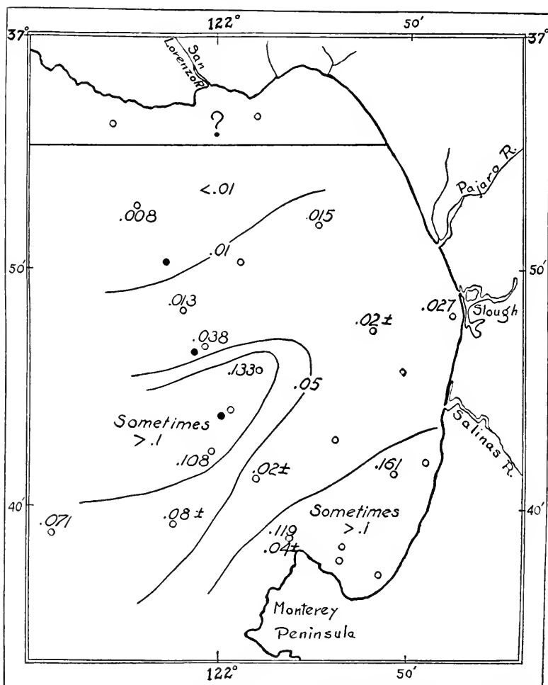
FIG. 34.—Distribution of nitrates (in milligrams per liter of \text{NO}_3 ) at the surface. Heavy dots, nitrate-free.
