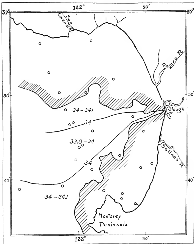
FIG. 14.— Salinity at a depth of 100 meters.
