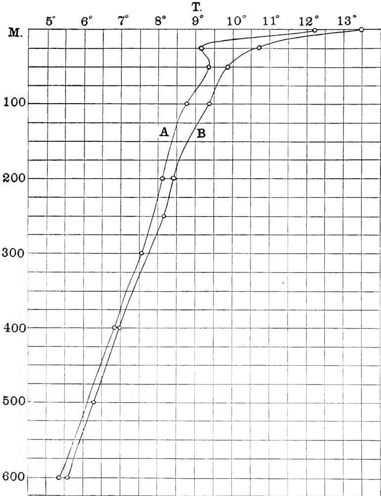
FIG. 9.— Maximum (B) and minimum (A) temperatures, surface to 600 meters, at Stations 8, 10, 17, 27 and 29.
