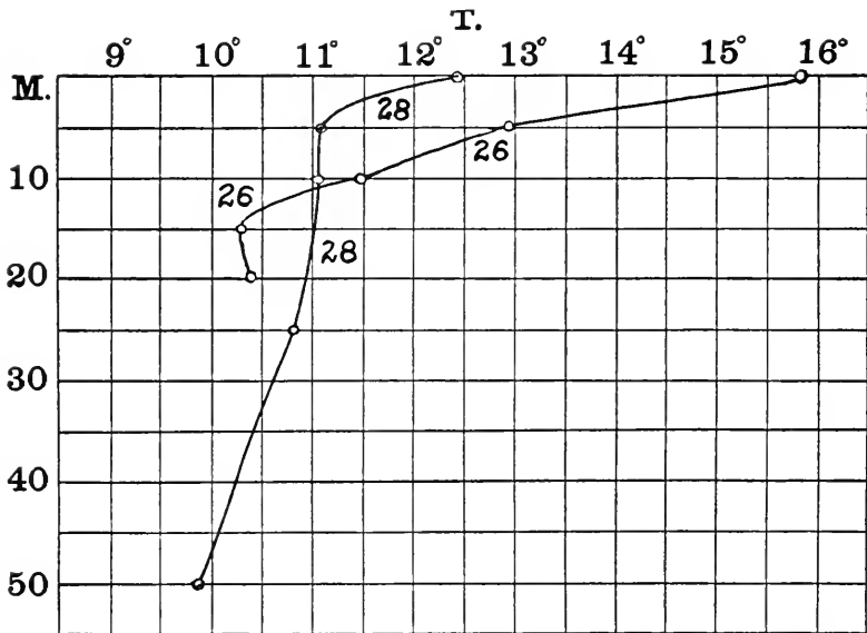
FIG. 21. Vertical distribution of temperature in the northern and southern bights of the bay (Stations 26, 28).
