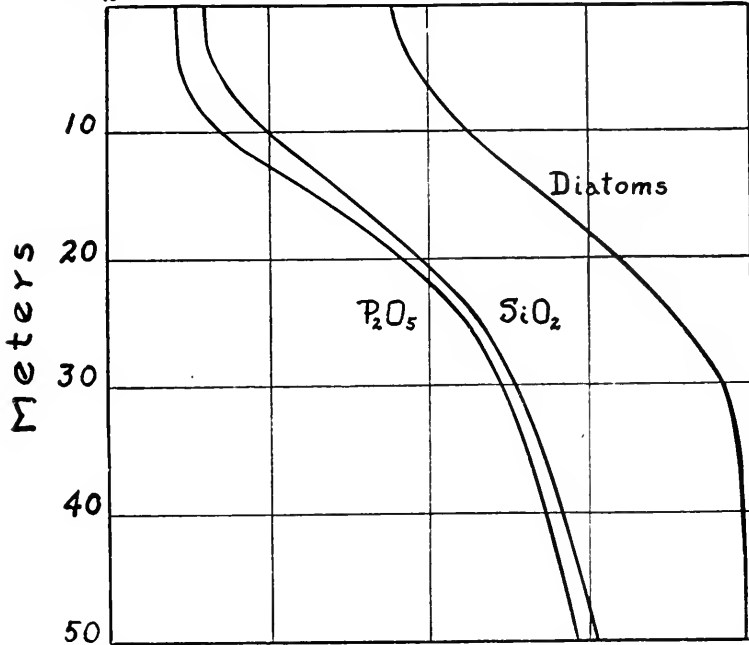
FIG. 41.— Vertical distribution of mean values for phosphates ( P_2O_5 ) and silicates ( SiO_2 ), in milligrams per liter, and of average number of diatom cells in thousands per liter, in the upper 50 meters, at Stations 7, 10, 12, 13, 15, 16, 18, 19, and 24.
