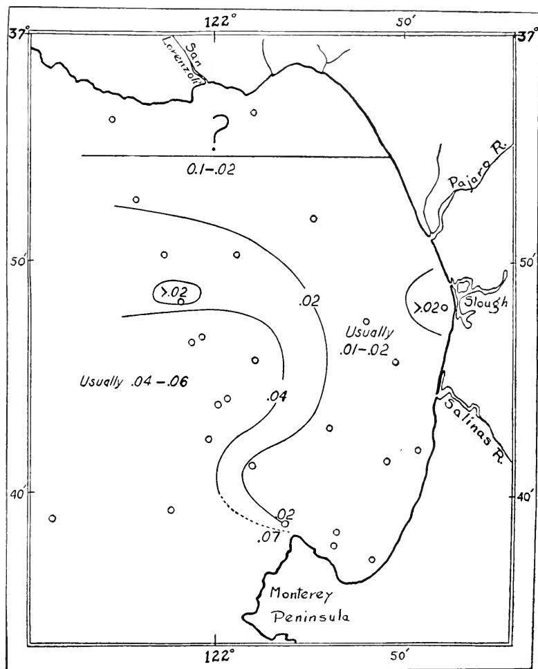
FIG. 26.— Distribution of phosphates (as milligrams per liter of P 2 O 5 ), at the surface.
