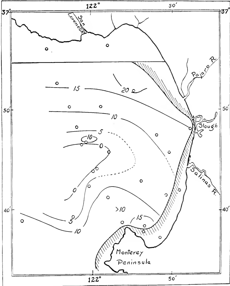
FIG. 40.— Depth below the surface of the layer of .6 milligram of \text{SiO}_2 per liter.
