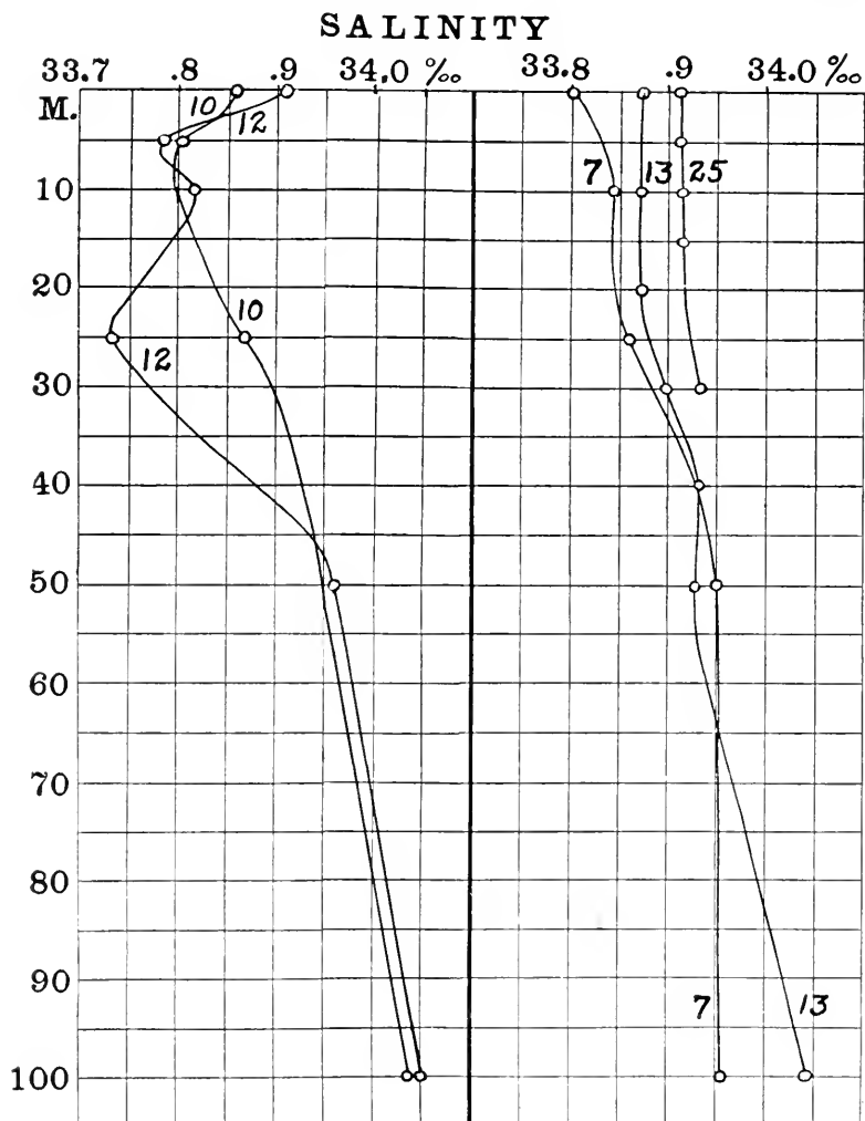
FIG. 12.— Vertical distribution of salinity in the upper 100 meters at representative stations (10, 12; and 7, 13, 25).
