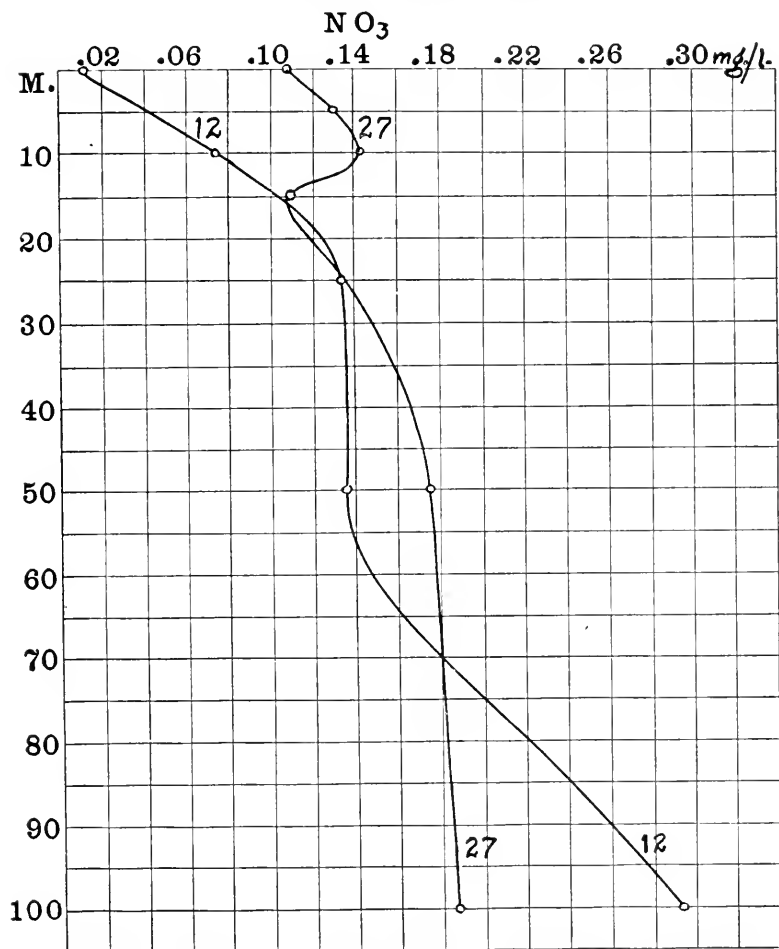
FIG. 35.—Vertical distribution of nitrates (in milligrams per liter of \text{NO}_3 ) at Stations 12 and 27.
