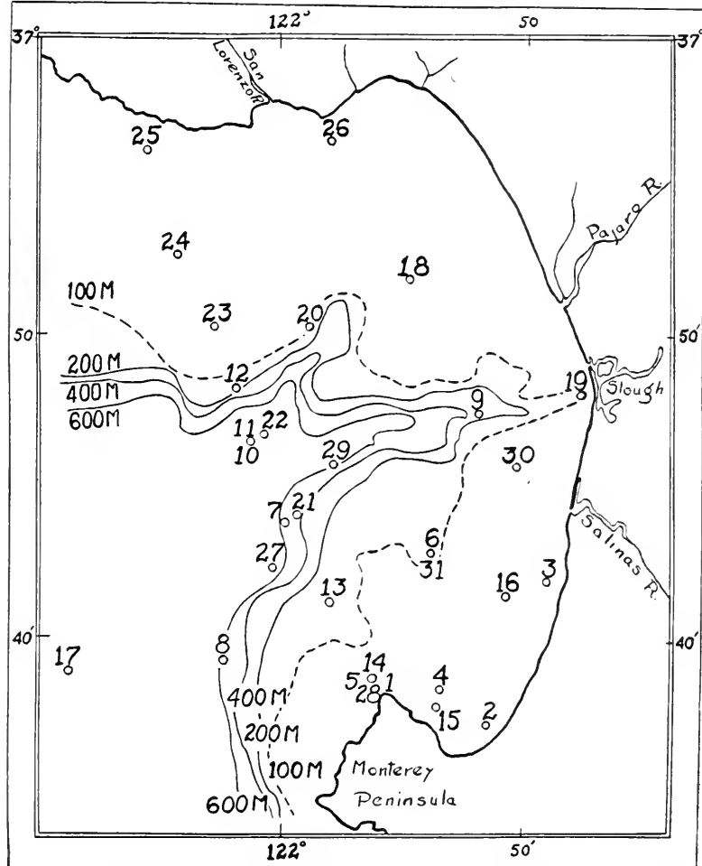
FIG. 1.—Chart of Monterey Bay, showing locations of stations, and bottom contours for depths of 100, 200, 400 and 600 meters.
