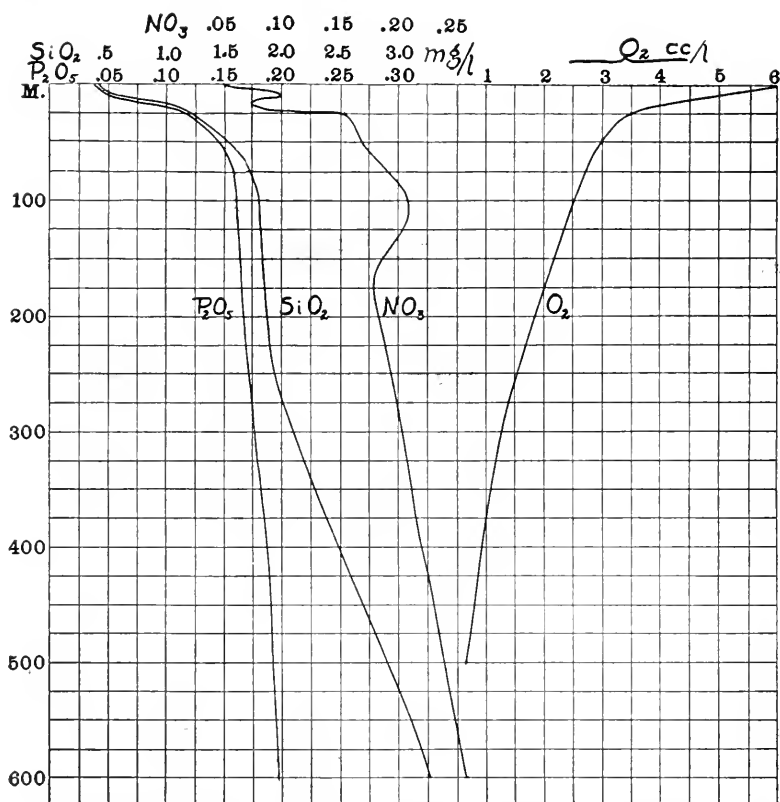
FIG. 28.— Mean value, for all stations of record, of phosphates (as P_2O_5 ), of silicates (as SiO_2 ), and of nitrogen in the form of nitrate, in milligrams per liter, and of dissolved oxygen in cubic centimeters per liter reduced to pressure of 760 mm. of mercury and temperature of 0^\circ C .
