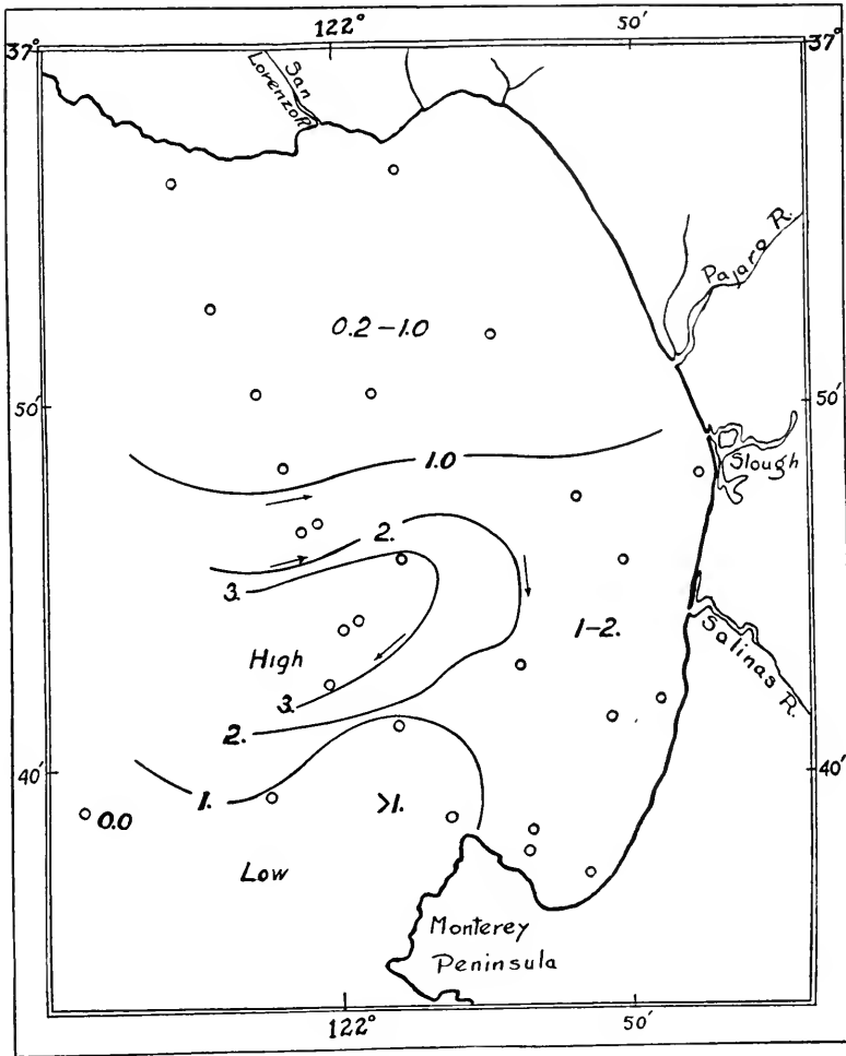
FIG. 24.— Dynamic gradient and indicated drift, at the surface, July 10-24, referred to the offing of Point Pinos (Sta. 17) as base station. The dynamic heights are given for every one dynamic centimeter.
