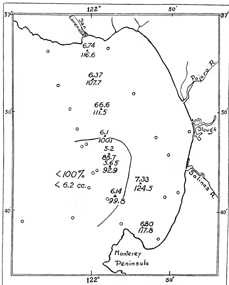
FIG. 42.—Oxygen at the surface, in cubic centimeters per liter (upper figures) and in per cent of saturation (lower figures).
