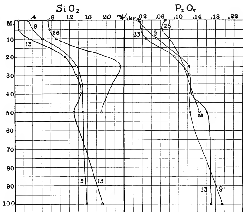
FIG. 27.— Vertical distribution in the upper 100 meters, of silicates (as \text{SiO}_2 ) and of phosphate (as \text{P}_2\text{O}_5 ) in milligrams per liter, at representative stations (9, 13, 28).
