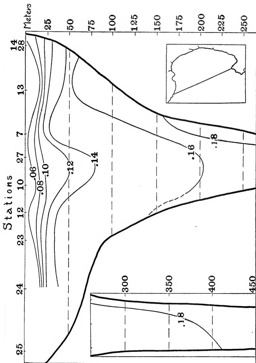
Fig. 31.—Profile across the mouth of the bay for phosphates (in milligrams per liter of P 2 O 5 ).
